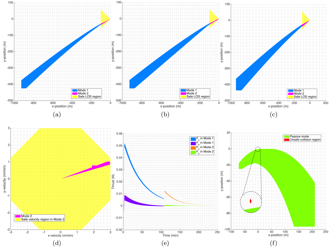
Figure 4: Reachable positions for rendezvous without any transition to Passive as computed by: (a) SDVTool (linear), (b) SpaceEx (linear), and (c) C2E2 (nonlinear). Reachsets computed by SDVTool for: (d) velocity in Mode 2, (e) thrust, and (f) positions reached after a transition to Passive during [120,125min].
