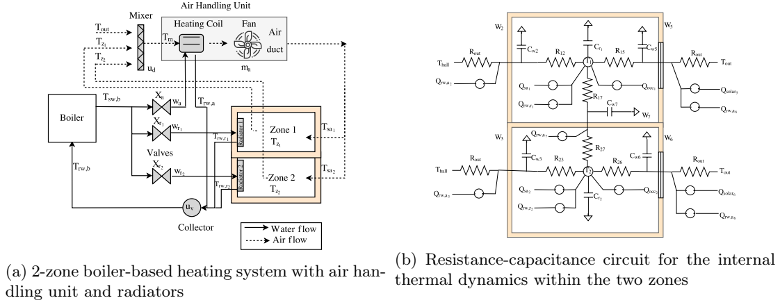
Figure 1: Building automation system setup
