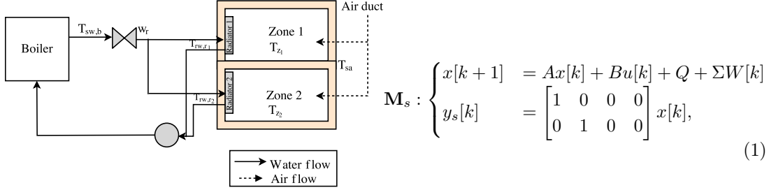
Figure 3: BAS setup for the first case study
