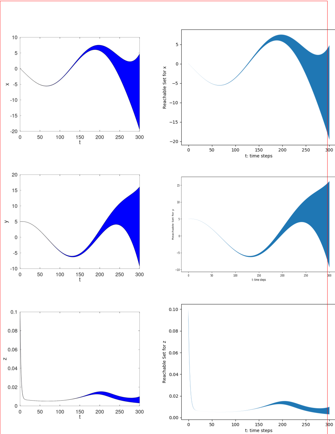
Figure 2: Figure depicting the reachable set computation of the Rossler model.
