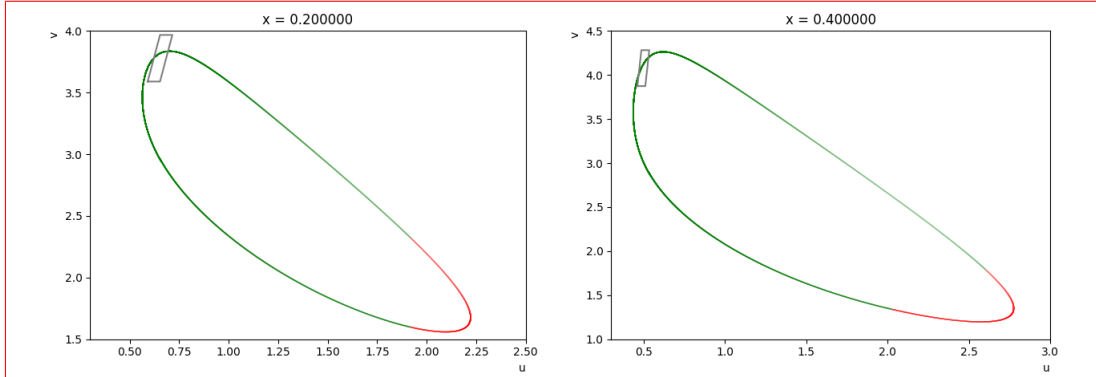
Figure 2: Brusselator: A cyclic trajectory for plan x = 0.2 (left) and x = 0.4 (right); the green zone indicates the contractive area ( \lambda < 0 ) and the red zone the expansive one ( \lambda > 0 )
