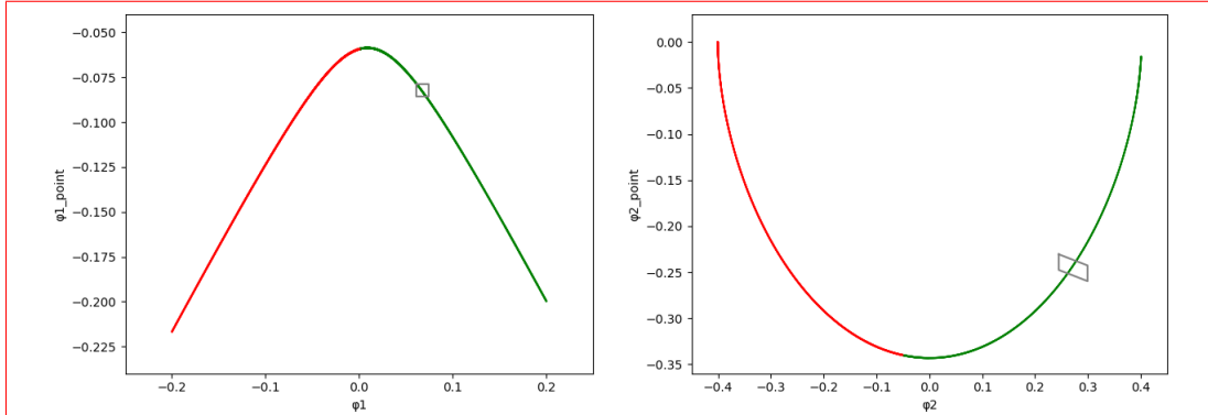
Figure 5: Biped: A cyclic trajectory for plan \phi_1 (left) and \phi_2 (right); the green zone indicates the contractive area ( \lambda < 0 ) and the red zone the expansive one ( \lambda > 0 )
