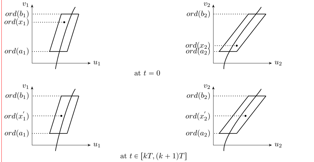
Figure 1: Scheme of S_1 (left) and S_2 (right) at t = 0 (top) and for some t \in [kT, (k+1)T] (bottom).
