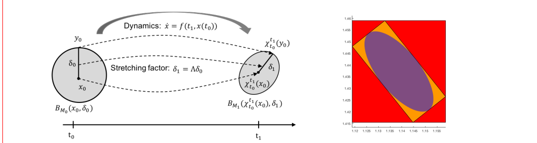
Figure 1: (Left) Visualization of one step of the Lagrangian Reachtube (LRT). The dashed arrows reflect the solution flow \chi of Eq. (1)(left). In this figure, \delta_0 = \eta \xi_0 and \delta_1 = \eta \xi_1 . (Right) Brusselator snapshot of the wrapping deficiency of Line 3 in Algorithm 1.
