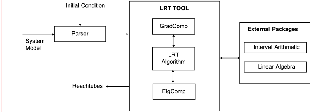
Figure 2: Overall architecture of our new stand-alone LRT tool. GradComp stands for Gradient Computation, and EigComp stands for Eigenvalue Computation.
