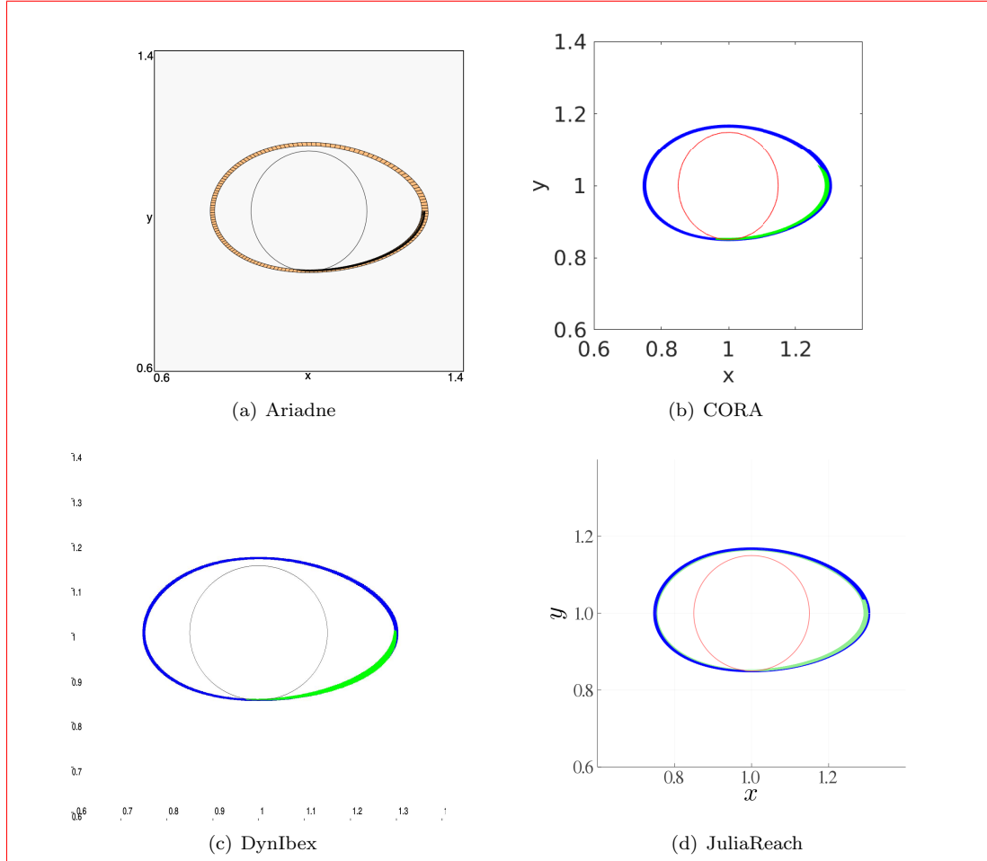
Figure 5: Reachable set overapproximation for LOVO20, with x, y \in [0.6, 1.4] , where the circular guard is shown.
