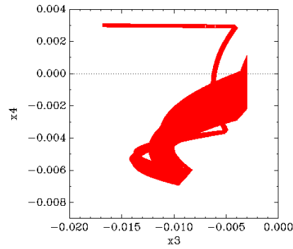
(e) XSpeed.
