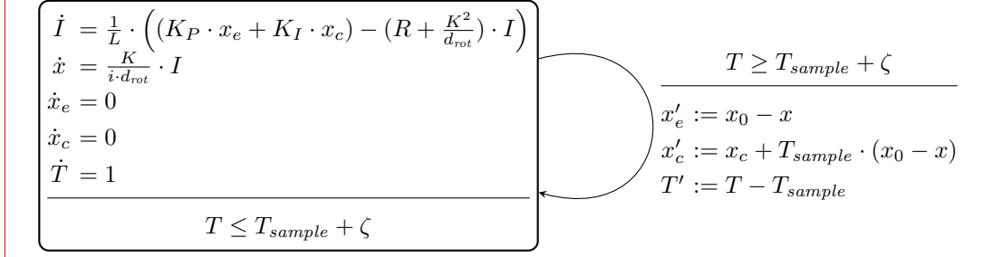
Figure 18: Hybrid automaton of the electro-mechanical brake with periodic discrete-time PI controller and sampling jitter.
