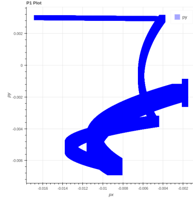
(b) C2E2.
