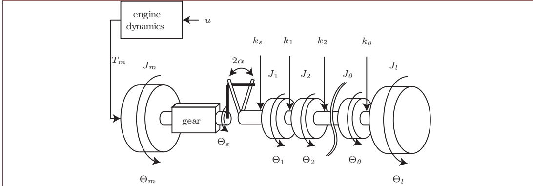
Figure 7: Powertrain model.
