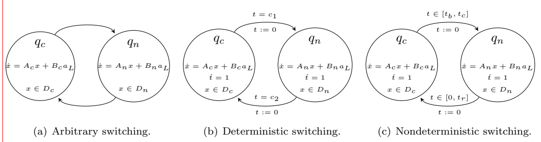
Figure 13: Three options adapted from the original benchmark proposal [16]. On the left, the system can switch arbitrarily between the modes. In the middle, mode switches are only possible at given points in time. On the right, mode switches are only possible during given time intervals.
