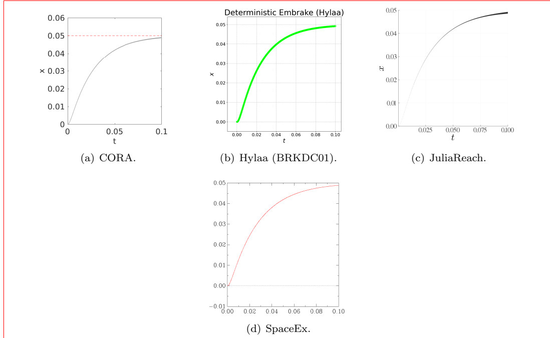
Figure 19: Brake: Reachable sets for x over time. Some tools additionally show possible trajectories.
