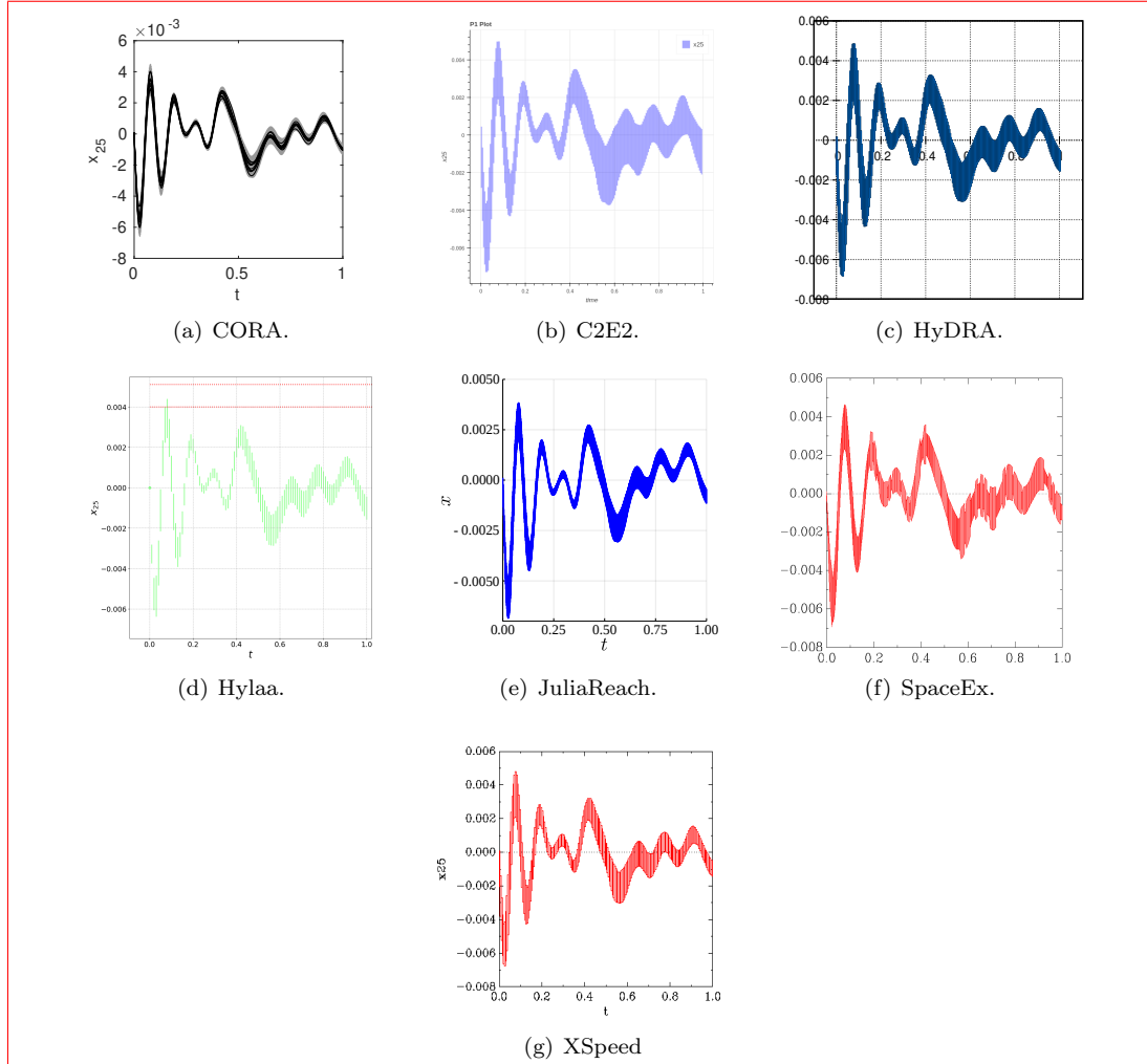
Figure 11: Building (BLDC01): Reachable sets of x_{25} plotted over time up to time 1. Some tools additionally show possible trajectories.
