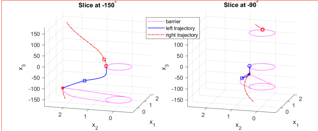
Figure 6: Left and right trajectories leading from crossover points for slices x_3 = -5\pi/6 and x_3 = -\pi/2 of the RCBRT with \beta = 0.5 and the pursuer at the origin. Slices of the target cylinder are also shown at the terminal points of the trajectories. For the slice at x_3 = -\pi/2 , the portion of the left barrier between the star symbol at the crossover point and the square symbol is part of the left trajectory. Figure taken from [Mitchell, 2001, figure 3].
