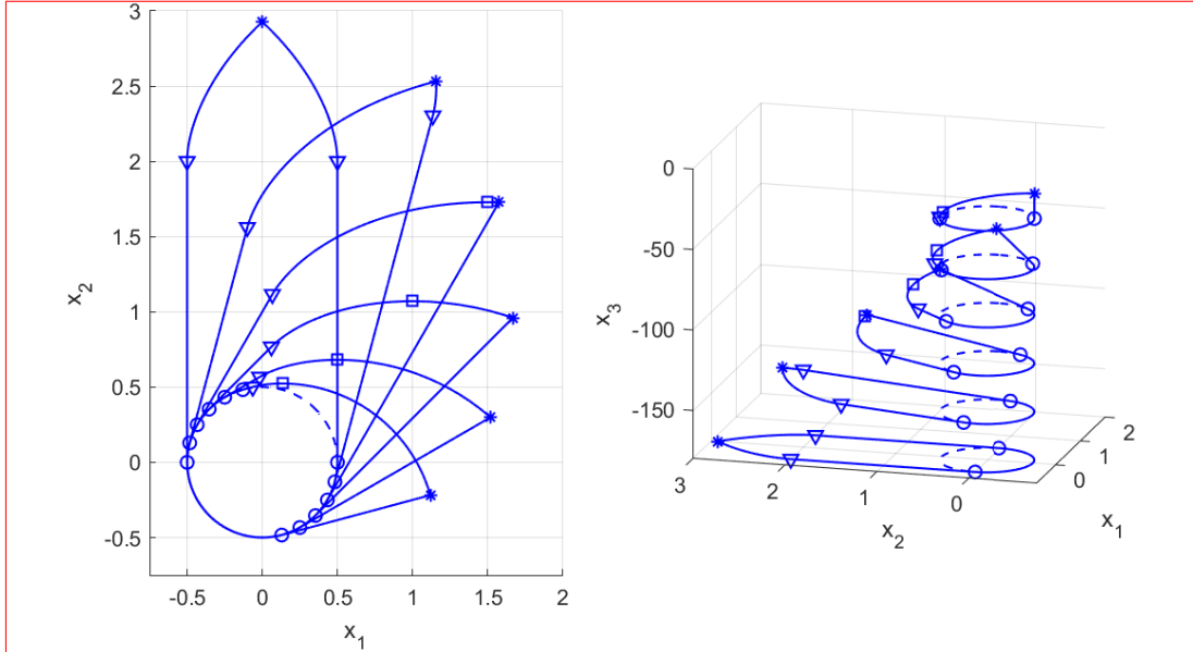
Figure 4: Two views of slices at fixed x_3 of the boundary of the RCBRT with \beta = 0.5 and the pursuer at the origin. The labelling is the same as that in figure 3. Figure taken from [Mitchell, 2001, figure 5], and the left subplot recreates [Merz, 1972, figure 7].
