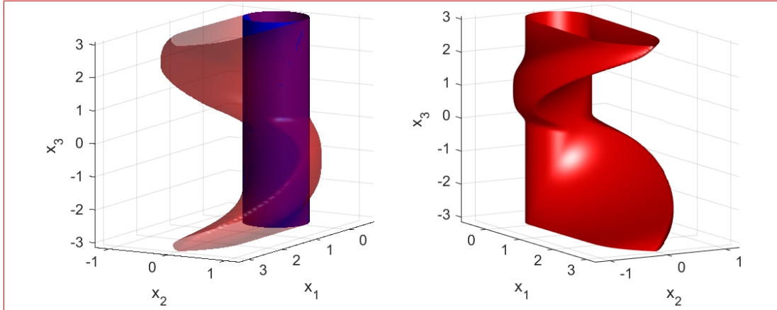
Figure 2: Two views of the surface of the RCBRT (red shape) for the basic problem. On the left, the RCBRT surface is partially transparent and the target set is shown as a solid blue cylinder. This set is the same as that shown in [Mitchell et al., 2005, Figure 3], [Mitchell, 2002, Figure 3.5] and [Mitchell, 2001, Figure 8], but with relative heading in [-\pi, \pi) (instead of [0, 2\pi) ) and different values for \beta , v_e and v_p .
