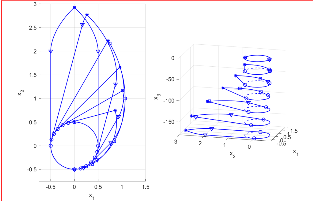
Figure 3: Two views of slices at fixed x_3 of the boundary of the RCBRT with \beta = 0.5 and the evader at the origin. Note that the x_1 and x_2 coordinates are swapped compared to the coordinate system in figure 1. The large circles are slices of the target set \mathcal{T} . The star symbols are the crossover points for each slice, the small circle symbols are the intersection of the barrier and the target set slices, and the triangle / square symbols denote points on the barrier slices where the combination of optimal trajectory segments to reach the barrier changes. Figure taken from [Mitchell, 2001, figure 6].
