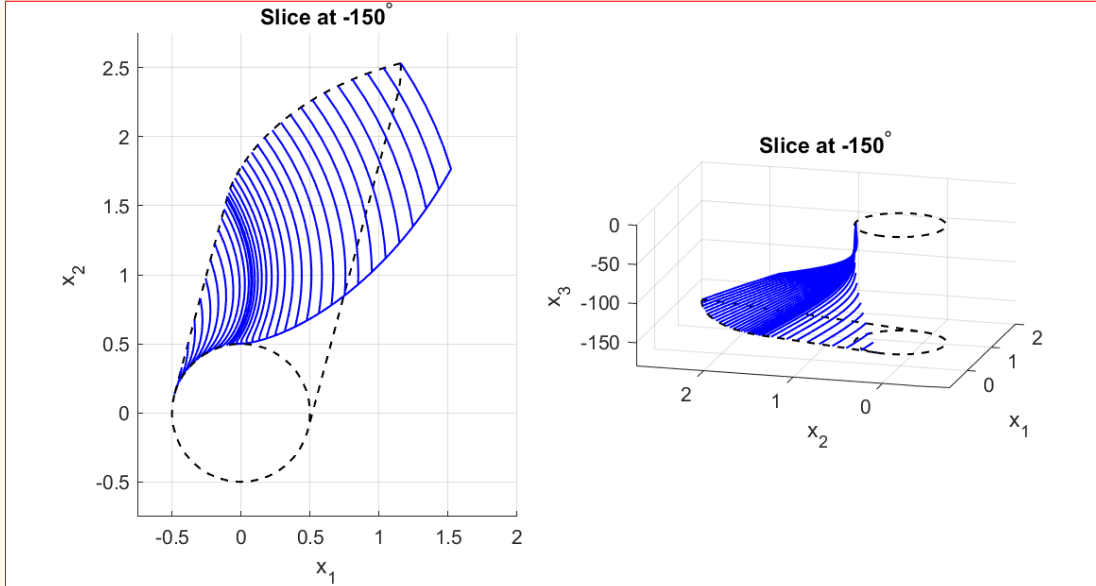
Figure 5: Two views of a coarse sampling of trajectories whose endpoints form a slice of the left barrier of the RCBRT with \beta = 0.5 and the pursuer at the origin. Note that the set of trajectories starting from points closer to the crossover point all share a terminal trajectory segment. Figure taken from [Mitchell, 2001, figure 4].
