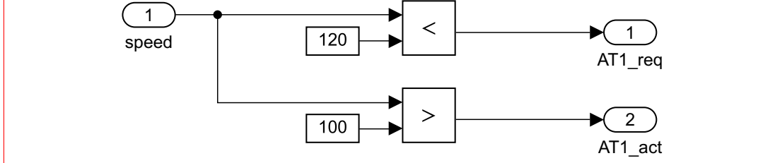
Figure 1: An example of the requirement structure used in the benchmark. Each requirement model contains one safety specification, here AT1_req , and one or more activation specifications, here AT1_act .
