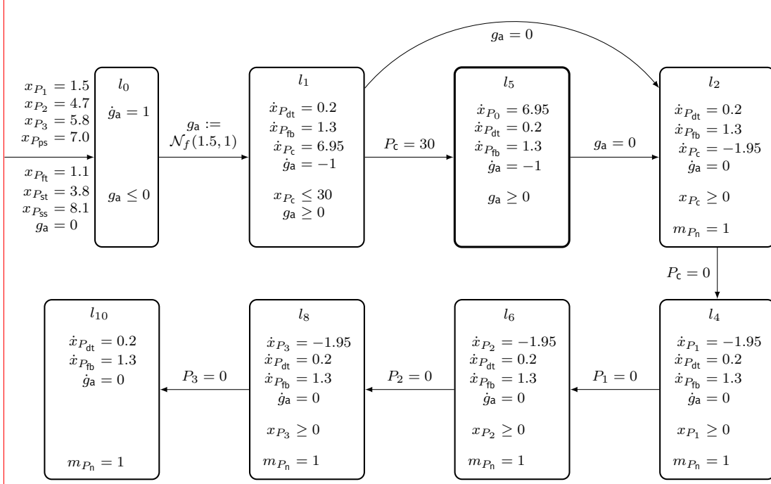
Figure 2: Transformed automaton for the water sewage facility with extension A and \mu = 1.5h and a capacity of 30 \cdot 10^6 l for the community buffer P_c . The random variable that describes the duration of the heavy rain is represented by the stochastic clock g_a . Note that all values not shown in the figure are zero.
