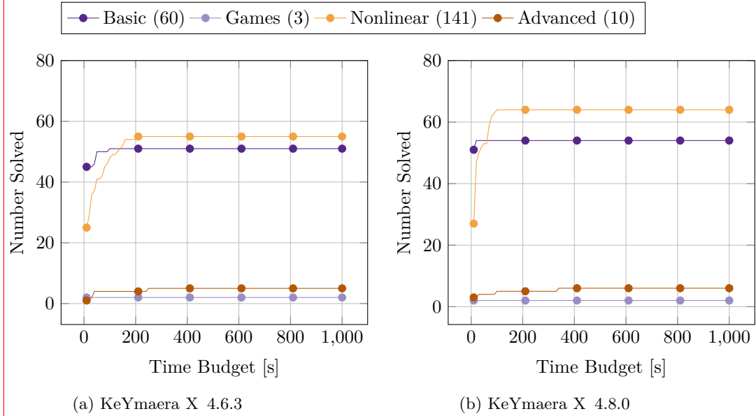
Figure 9: Result summary: Number of examples solvable fully automatically (A) with individual time budgets.
