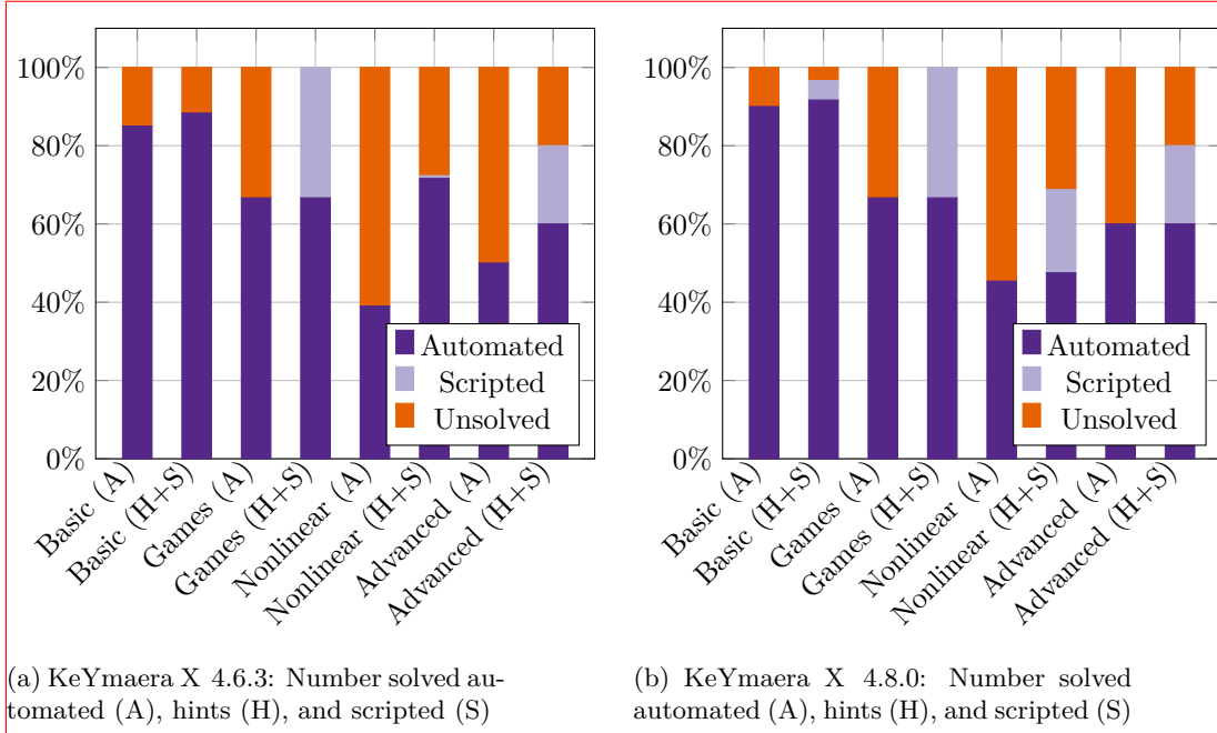
Figure 8: Result summary: The trend started in [MST + 19] continues: KeYmaera X 4.8.0 automation is now at the level of KeYmaera X 4.6.3 scripting; additional scripting in KeYmaera X 4.8.0 increases the number of solvable examples.
