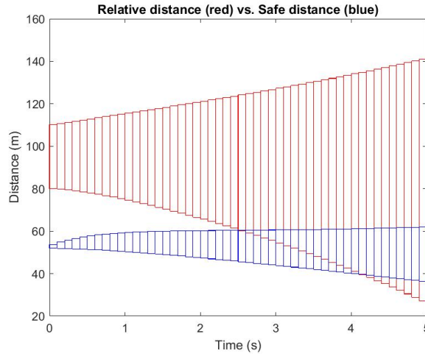
Figure 5: NN . Reachability analysis results of the ACC benchmark using a controller with 5 hidden layers (ReLU) of 20 neurons each.
