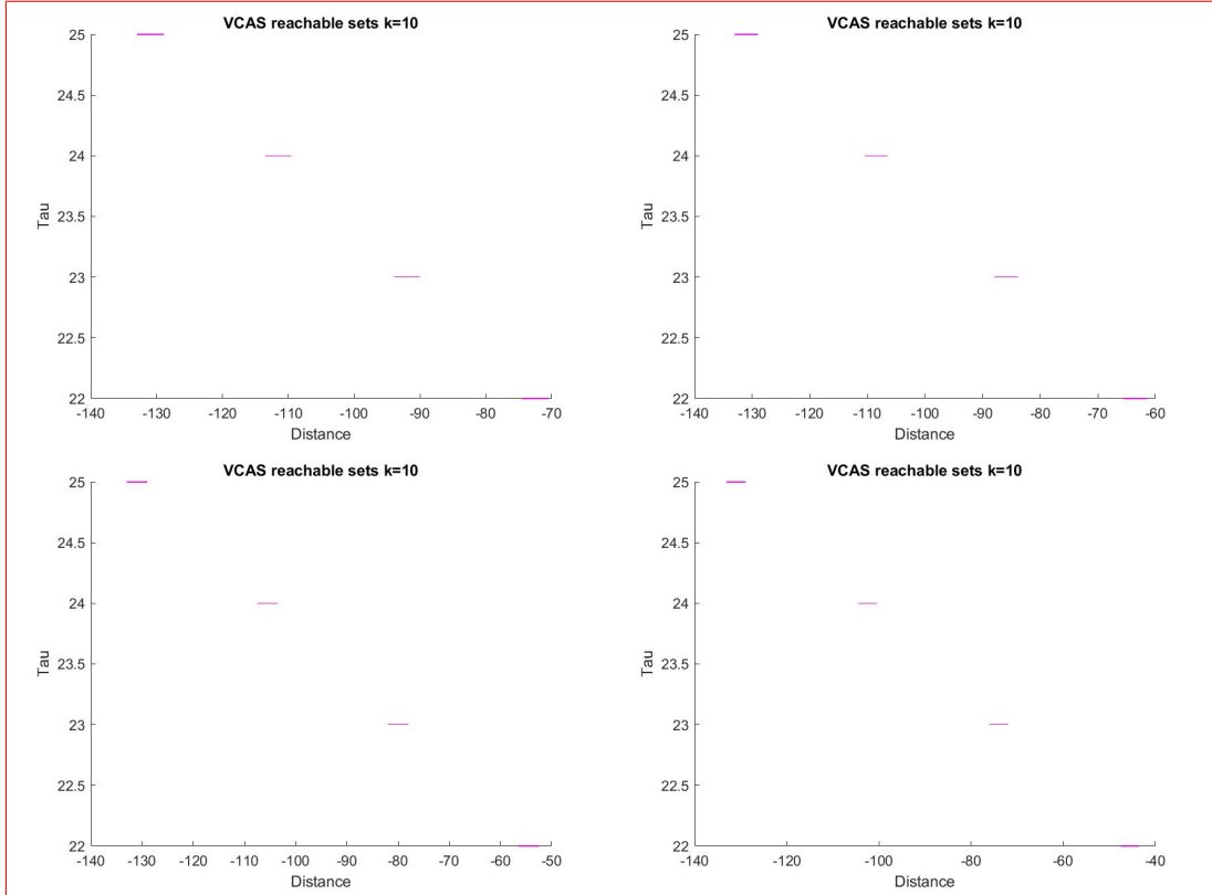
Figure 10: NNV . VCAS results when we choose the middle acceleration. The simulations were stopped before 10 steps since the safety property was violated.
