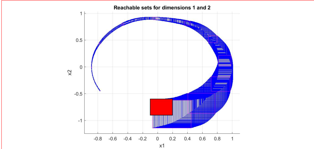
Figure 9: NNV . Reachability analysis results of TORA with sigmoid controller.
