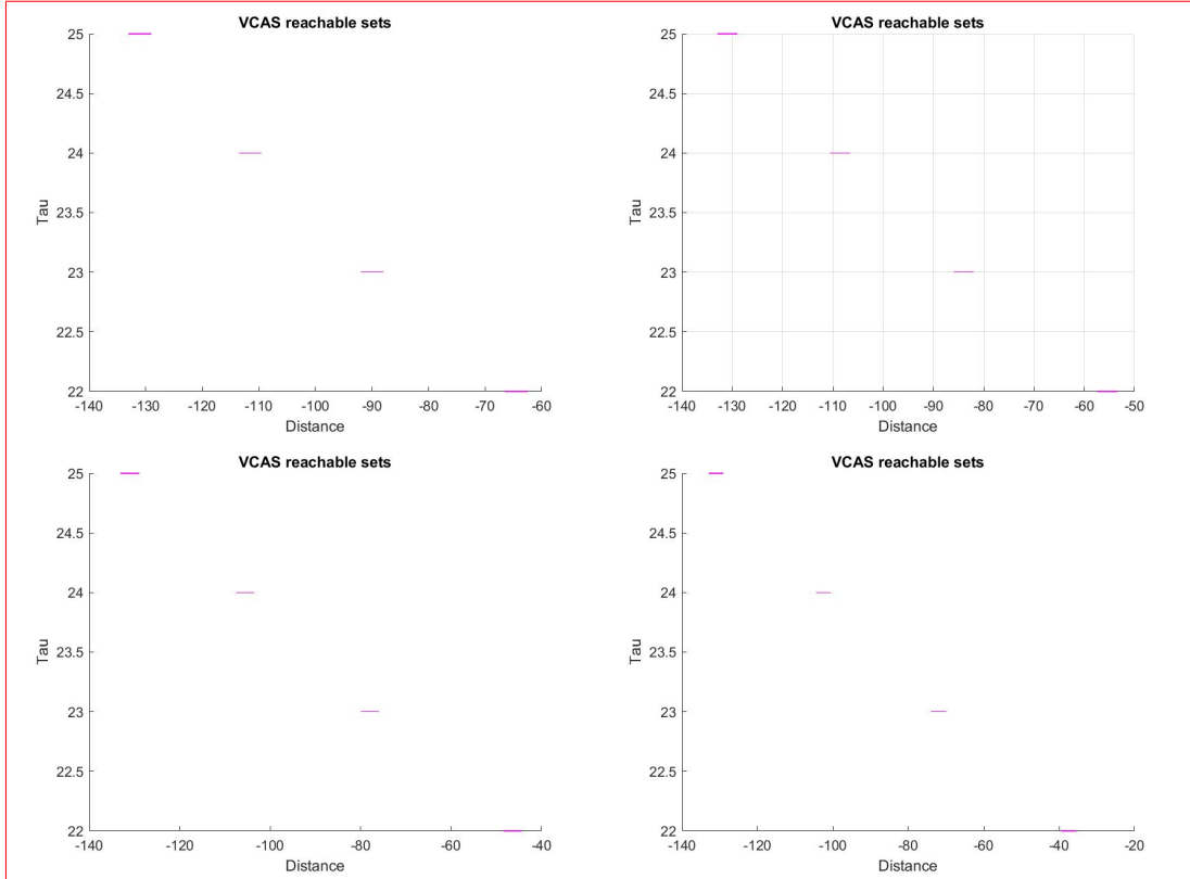
Figure 11: NNv . VCAS results when we choose the worst possible acceleration. The simulations were stopped before 10 steps since the safety property was violated.
