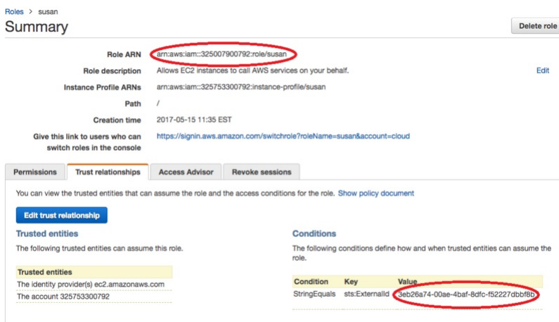
Fig. 8.30: The Roles Administration dialog
