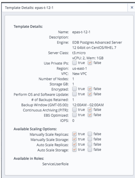
Fig. 5.9: Reviewing Template details
