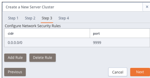
Fig. 5.4: Specify cluster security rules on the Step 3 tab.
