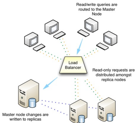
Fig. 2.3: EDB Ark performs automatic load balancing
