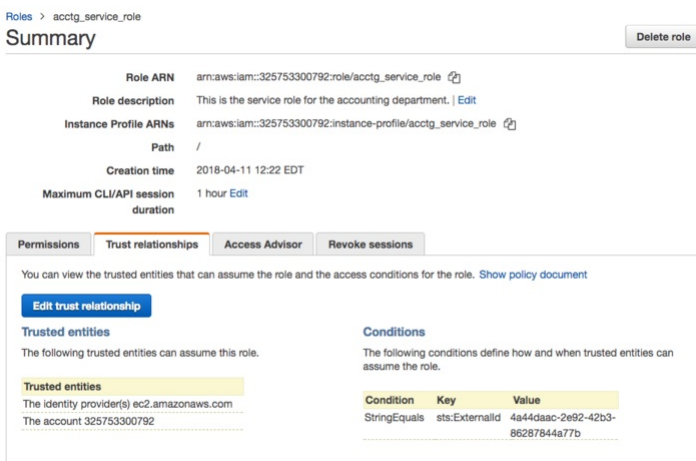
Fig. 6.14: The role detail summary
