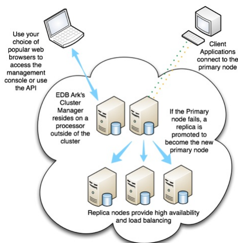
Fig. 2.1: Using EDB Ark in a Private Cloud.
