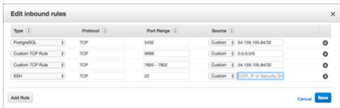
Fig. 11.1: Editing the Inbound Rules
