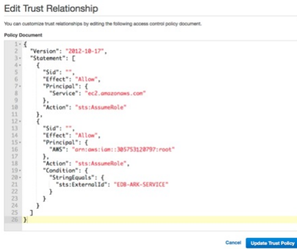
Fig. 6.13: The policy document
