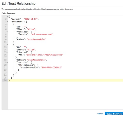
Fig. 3.12: The Policy Document
