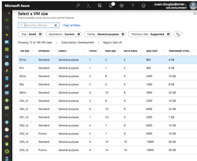
Fig. 6.41: Selecting a machine size
