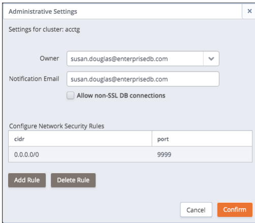
Fig. 5.14: The Administrative Settings dialog
