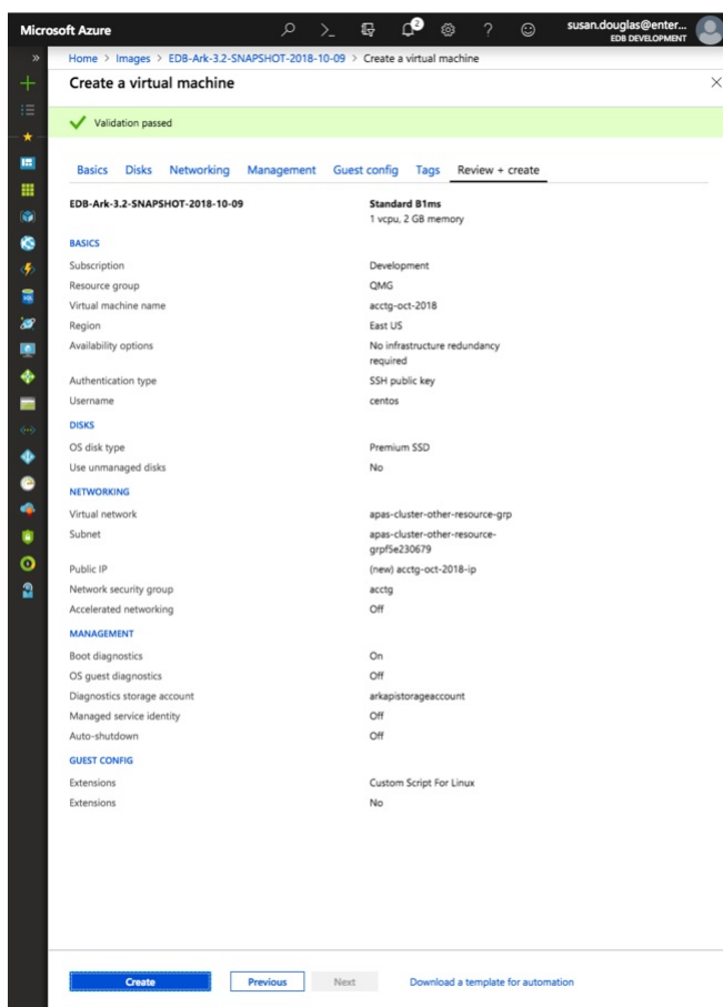
Fig. 6.43: Validating the machine definition
