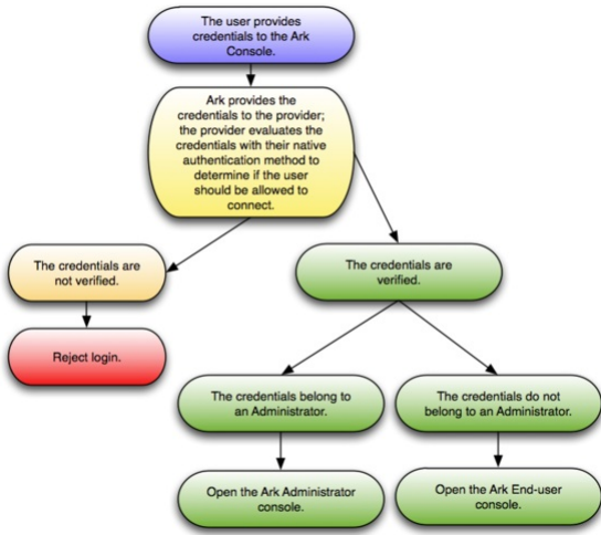
Fig. 5.3: Using Provider Authentication on Azure
