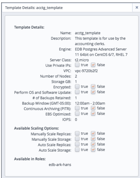
Fig. 8.24: The template details popup
