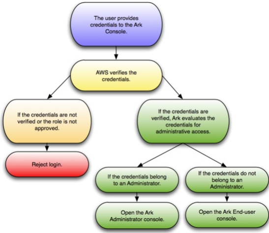
Fig. 5.1: Using Provider Authentication on AWS
