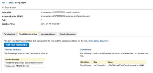
Fig. 3.14: The Summary tab of the Role detail panel.
