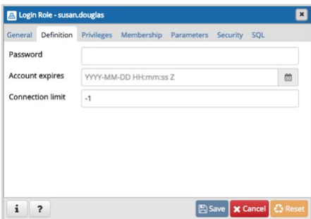
Fig. 4.4: Registering as a login role
