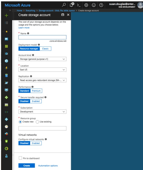
Fig. 6.38: Defining a storage account
