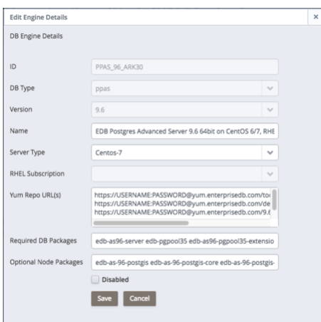
Fig. 8.21: Modifying the Engine Details dialog
