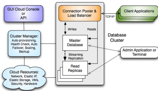
Fig. 2.2: An overview of the EDB Ark architecture
