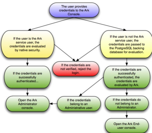
Fig. 5.4: Using PostgreSQL Authentication on Azur
