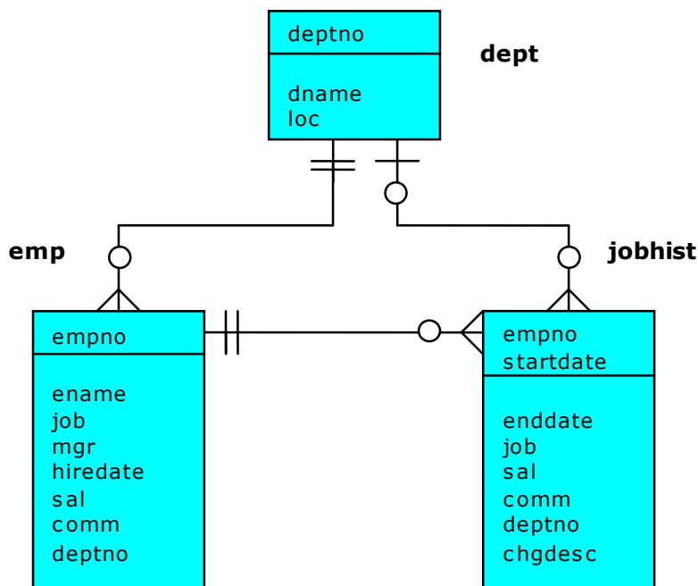
Figure 1 Sample Database Tables
