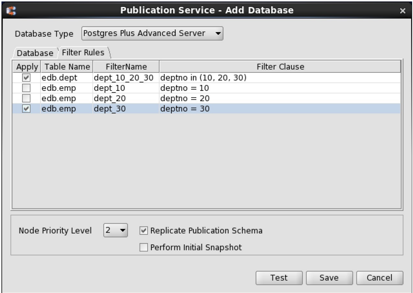
Figure 6-14: Enabling filter rules on a primary node
