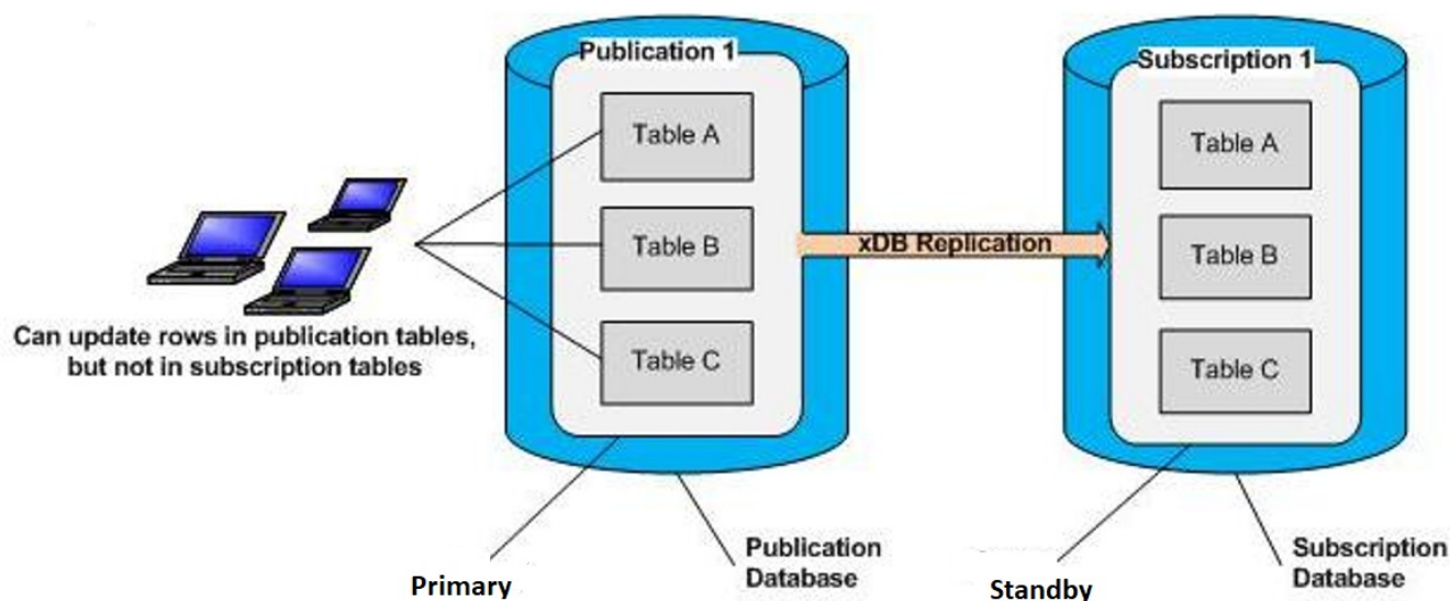
Figure 2-6: Single-Master (Primary-to-secondary) replication
