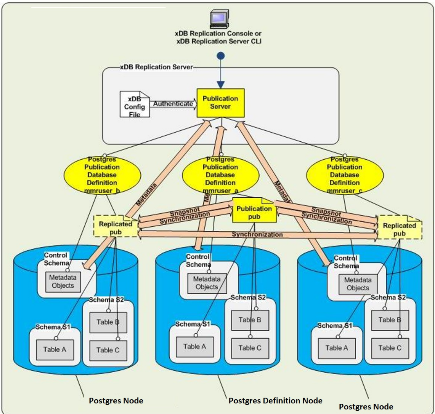
Figure 2-20: Postgres multi-master replication system
