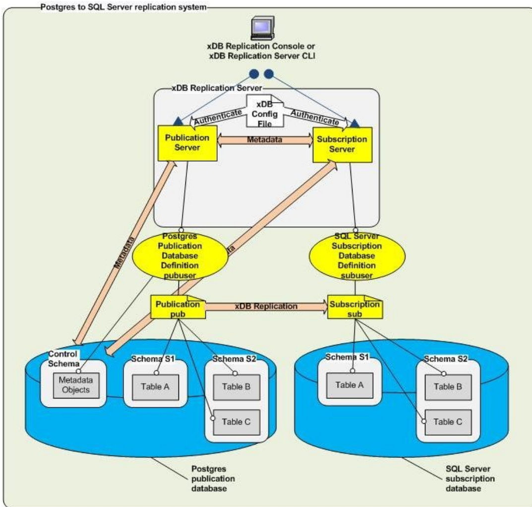
Figure 2-18: PostgreSQL or Advanced Server to SQL Server replication
