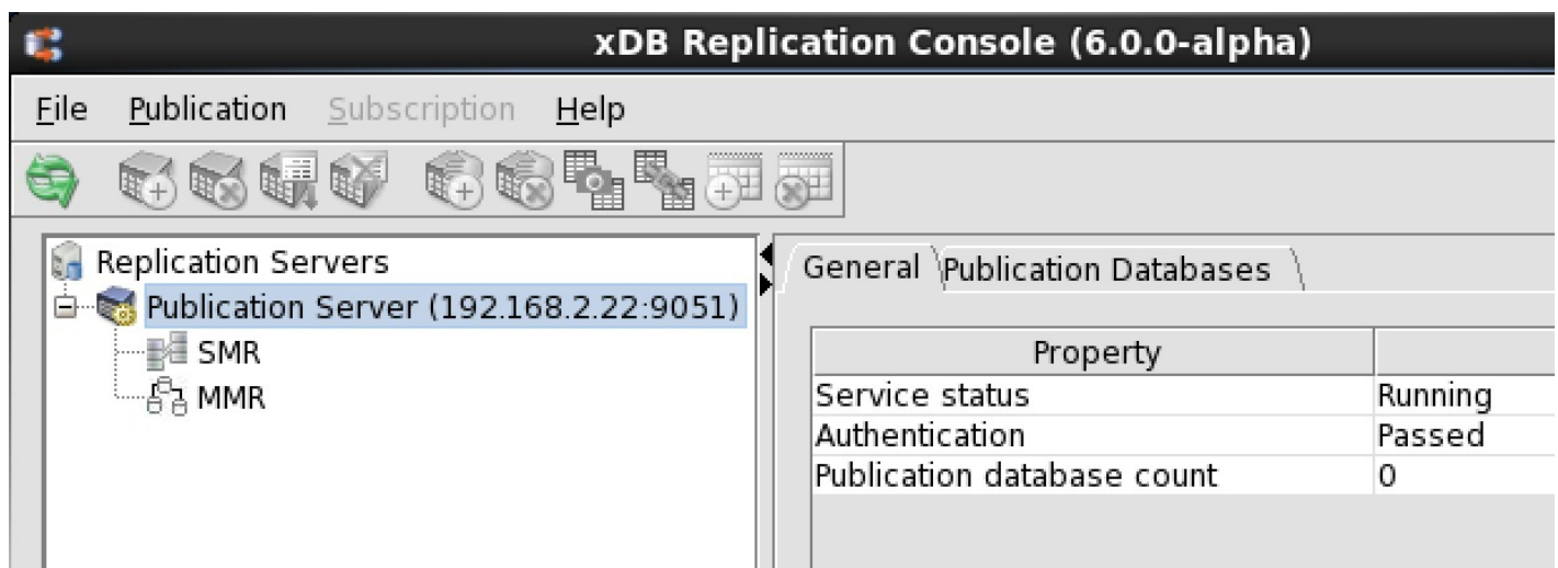
Figure 5-5: Replication tree after registering a publication server
