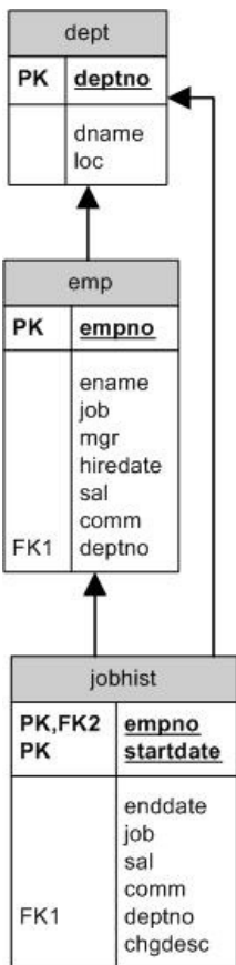
Figure 7-74: Entity relationship diagram of tables with foreign key constraints
