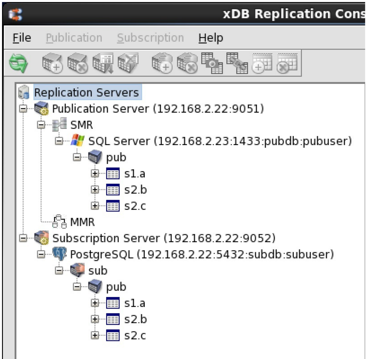
Figure 2-14: SQL Server to Postgres replication tree
