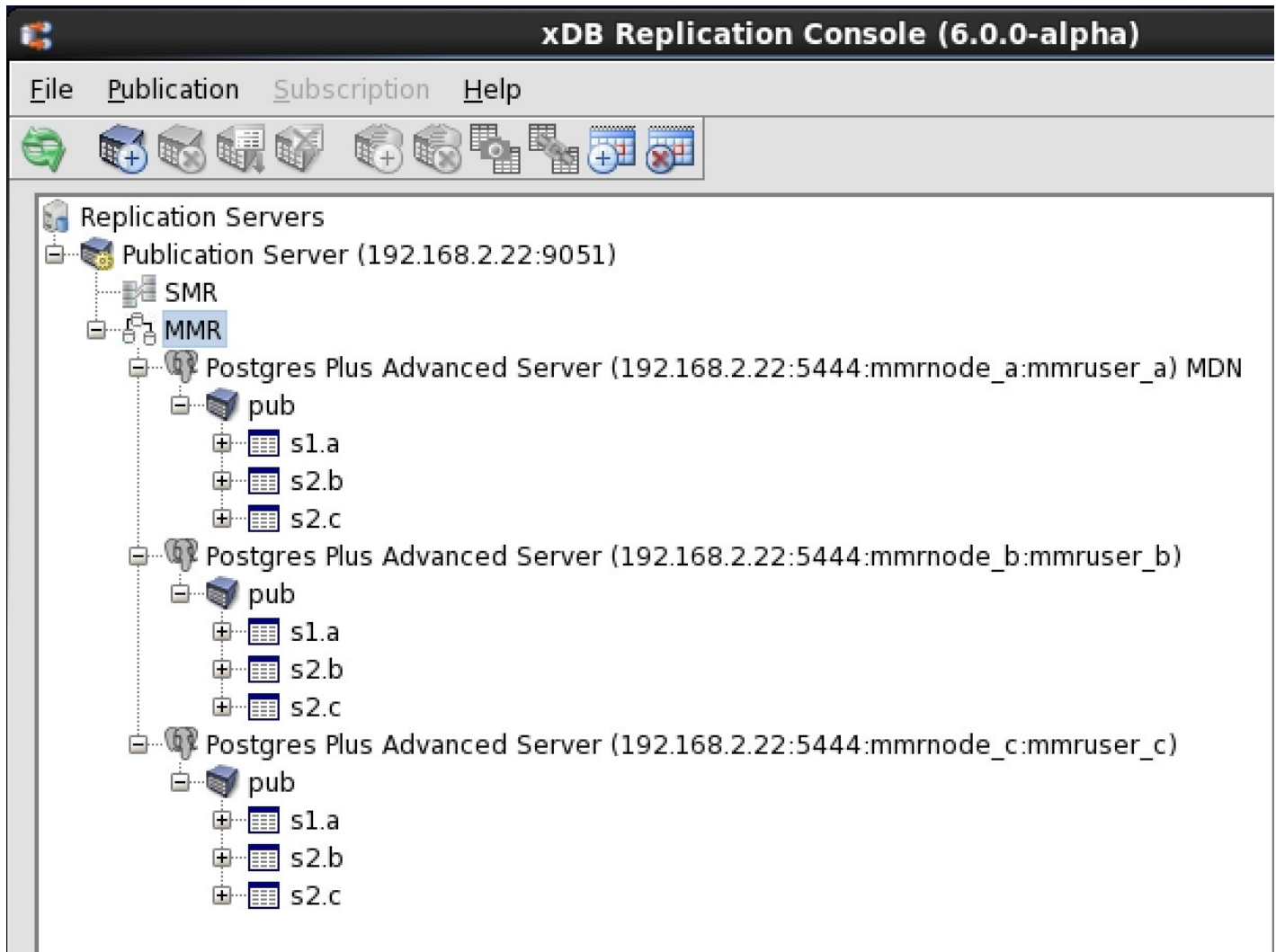
Figure 2-21: Postgres multi-master replication tree
