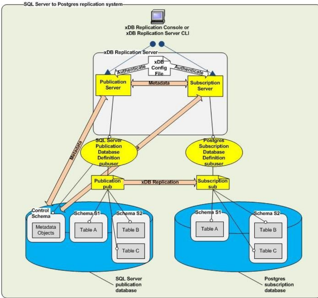
Figure 2-13: SQL Server to PostgreSQL or Advanced Server replication
