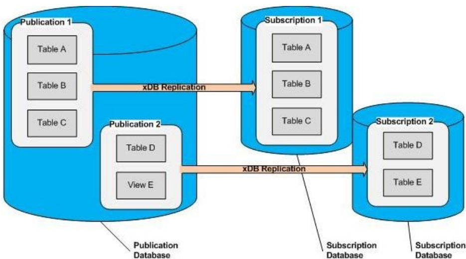
Figure 2-2: Publications replicating to two subscription databases
