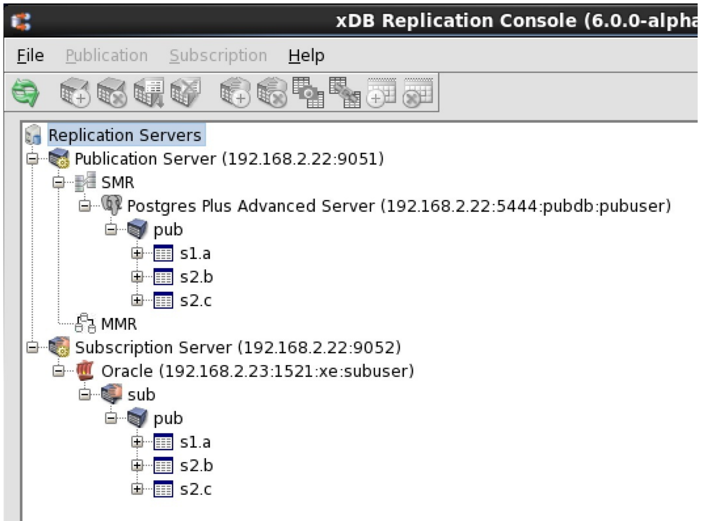
Figure 2-16: Advanced Server to Oracle replication tree
