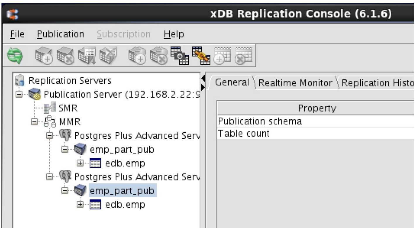
Figure 7-111: MMR system with a Postgres 10 or later partitioned table
