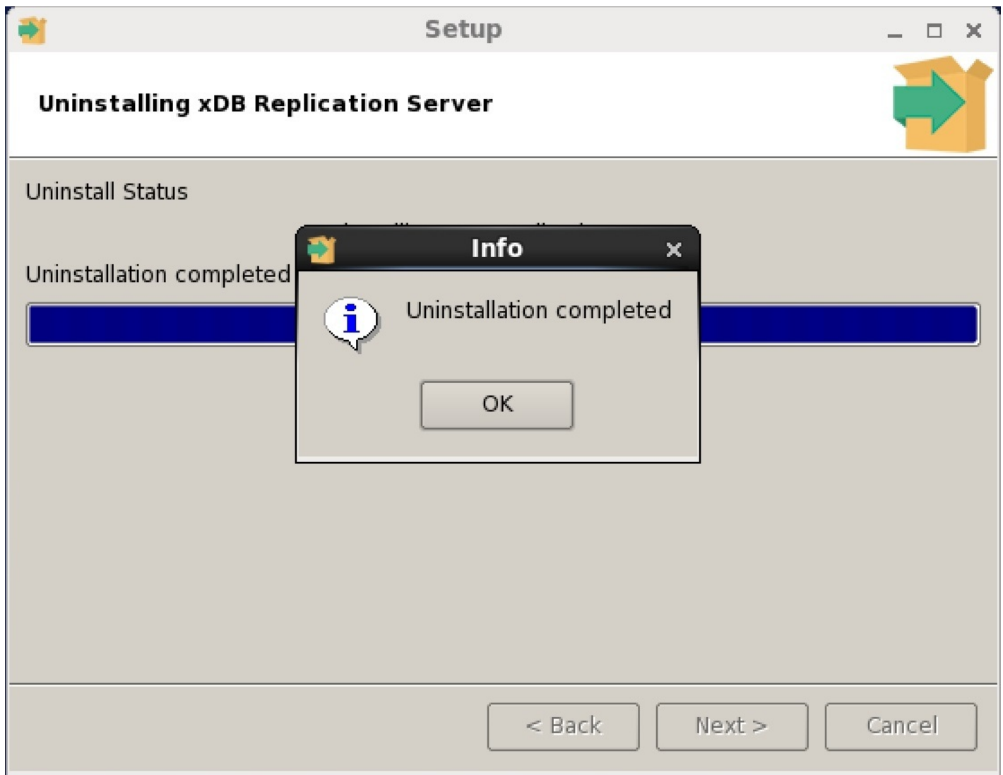
Figure 3-27: Uninstallation completed
