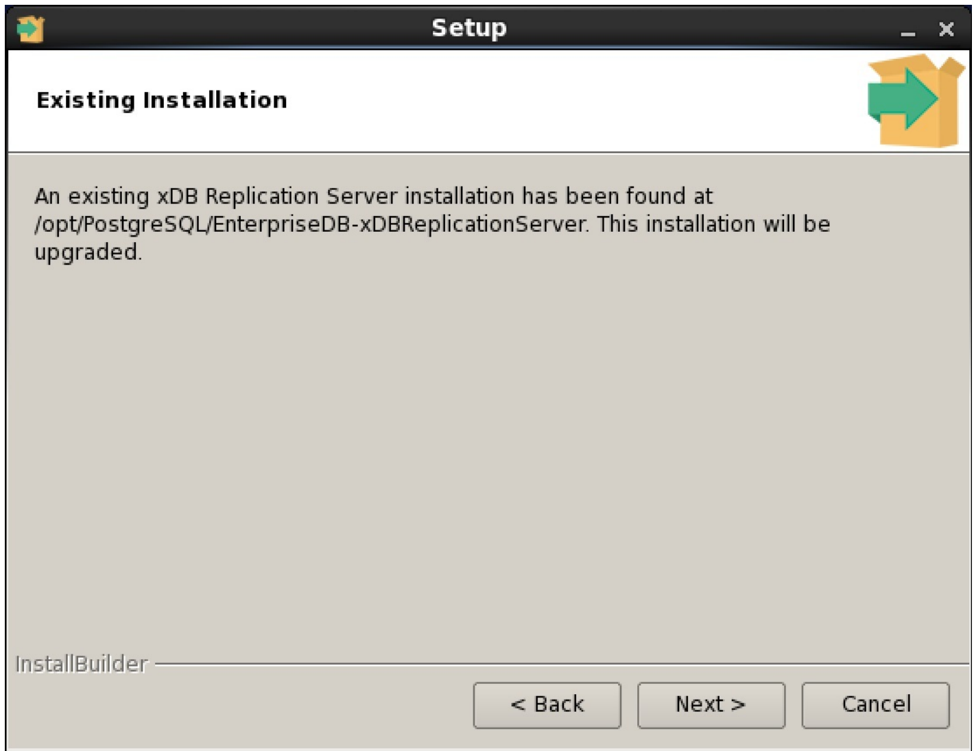
Figure 10-2: Existing installation
