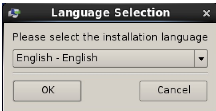
Figure 3-11: Installation language
