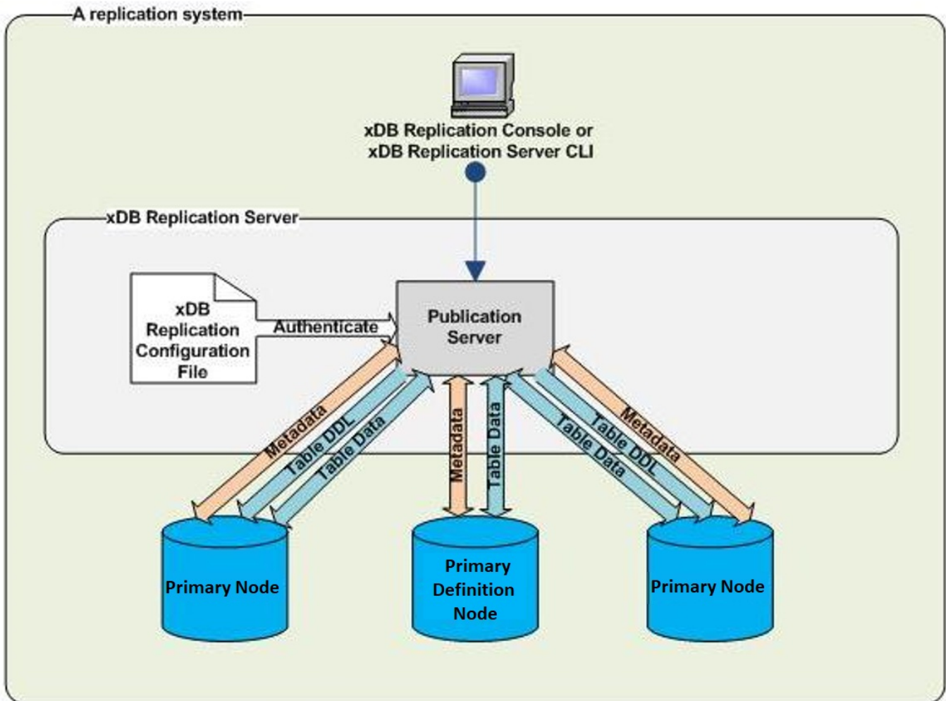
Figure 2 9: xDB Replication Server - physical view (multi-master replication system)
