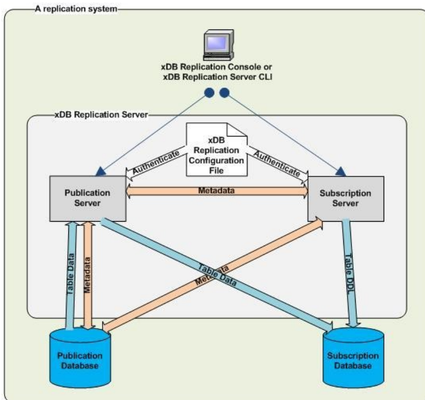
Figure 2-8: xDB Replication Server - physical view (single-master replication system)
