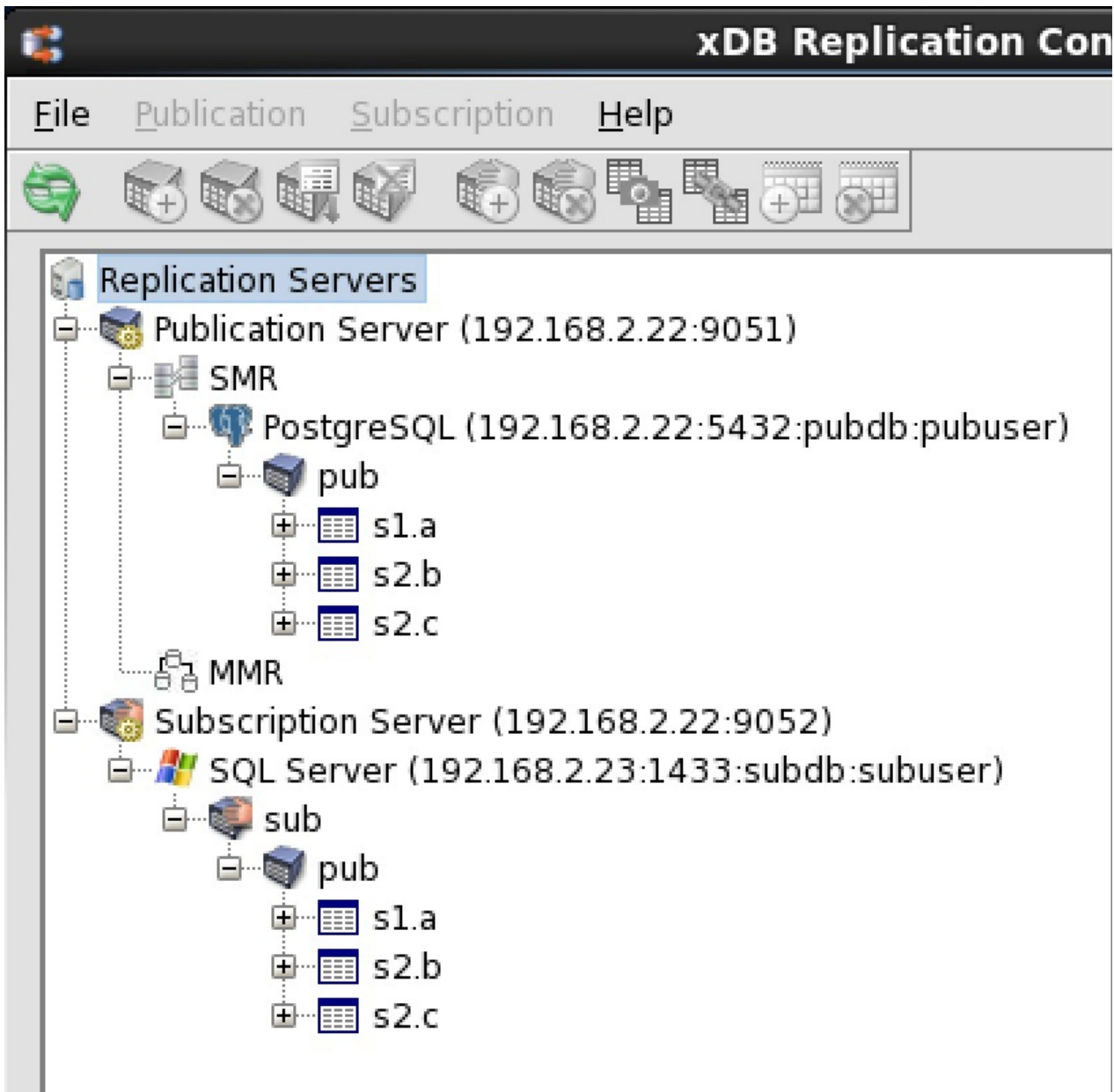
Figure 2-19: Postgres to SQL Server replication tree
