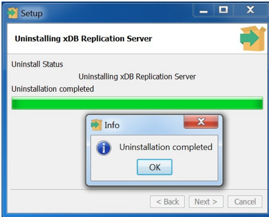
Figure 3-31: Uninstallation completed
