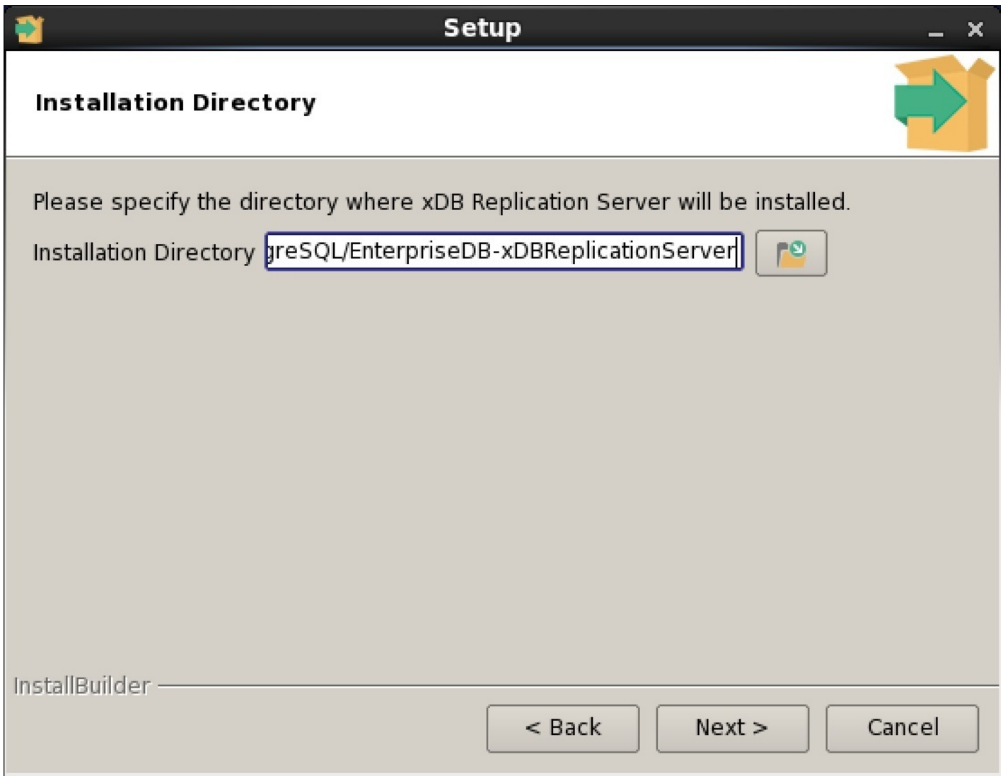
Figure 3-14: Installation directory
