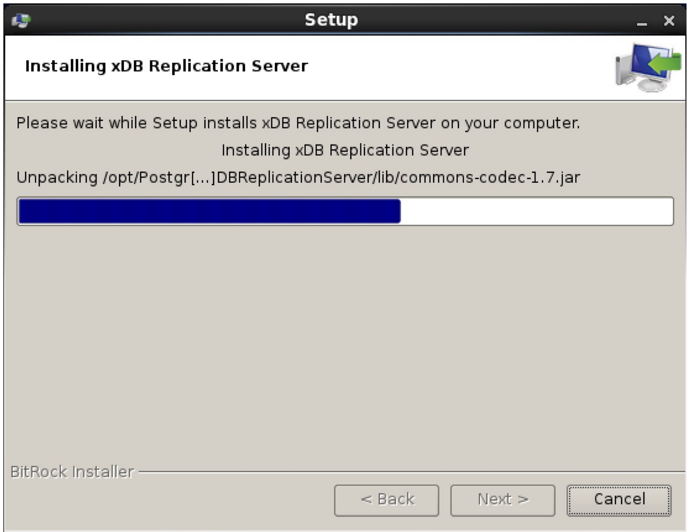
Figure 3-23: Installation progress
