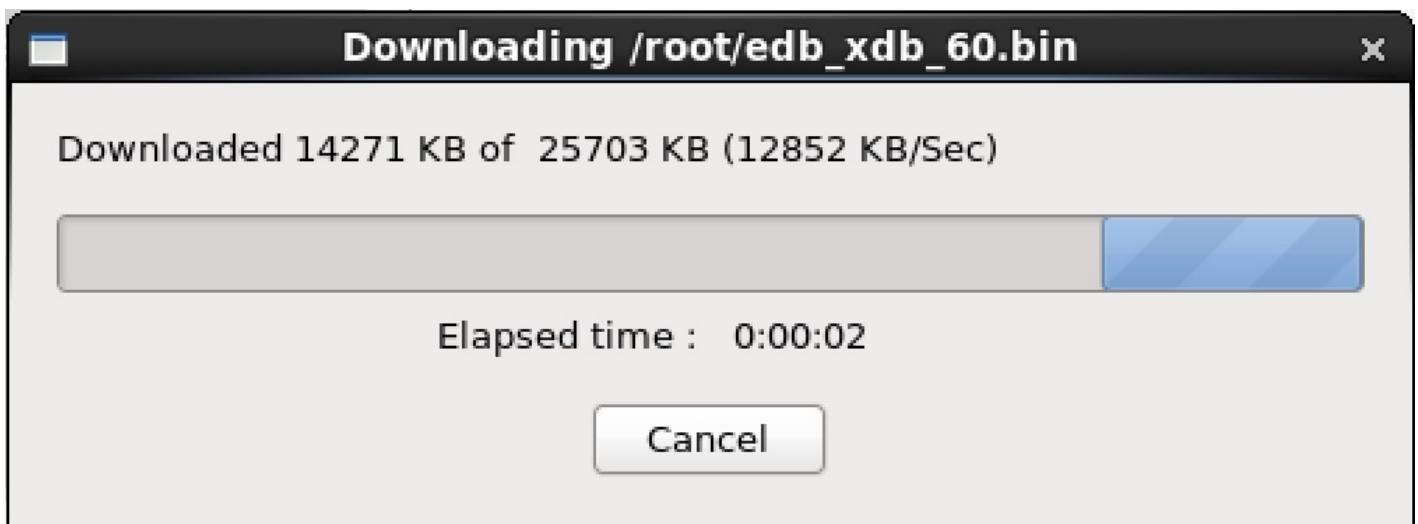
Figure 3-9: Downloading progress
