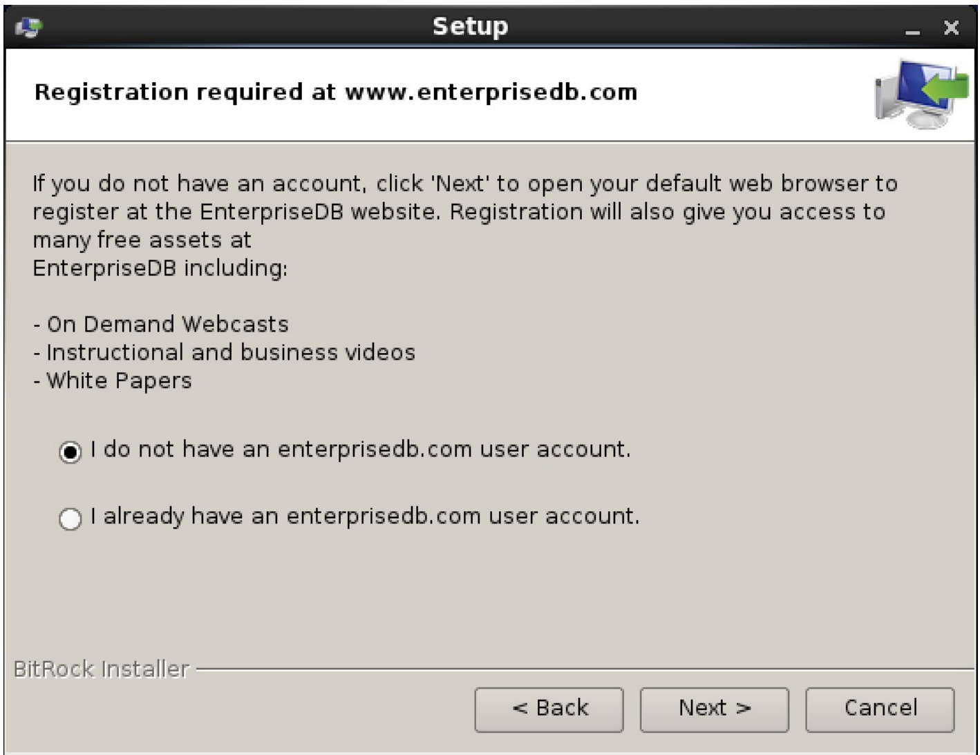
Figure 3-16: Account registration
