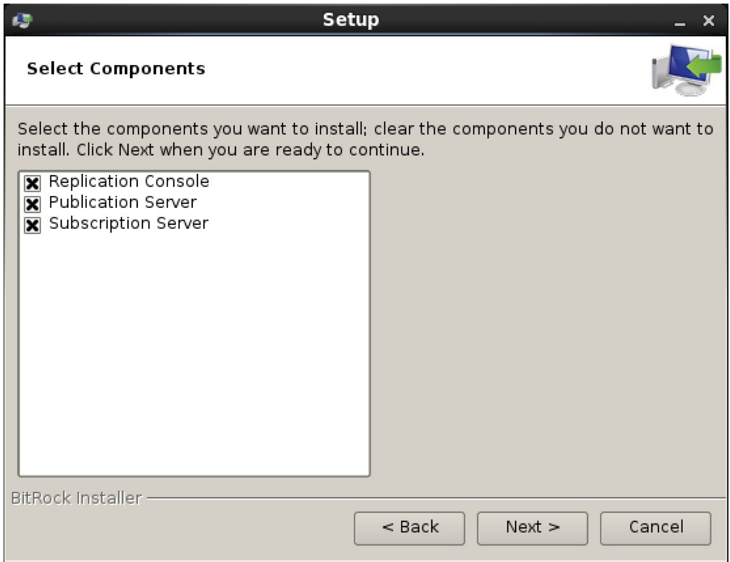
Figure 3-15: Select components
