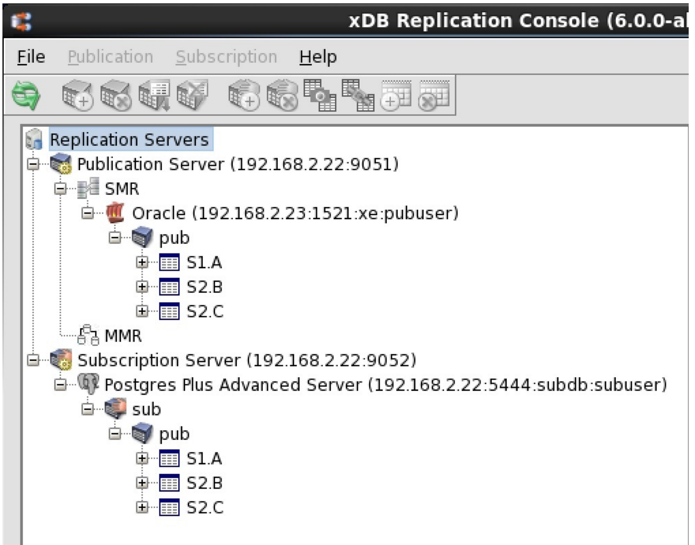
Figure 2-12: Oracle to Postgres replication tree
