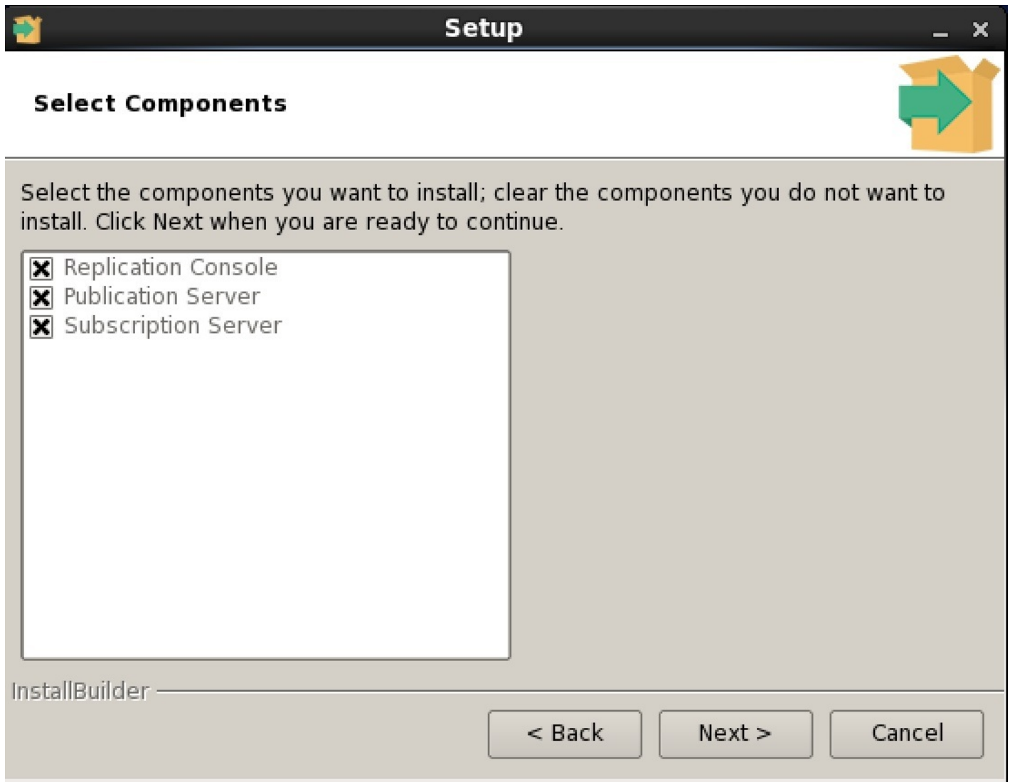
Figure 10-1: Select components
