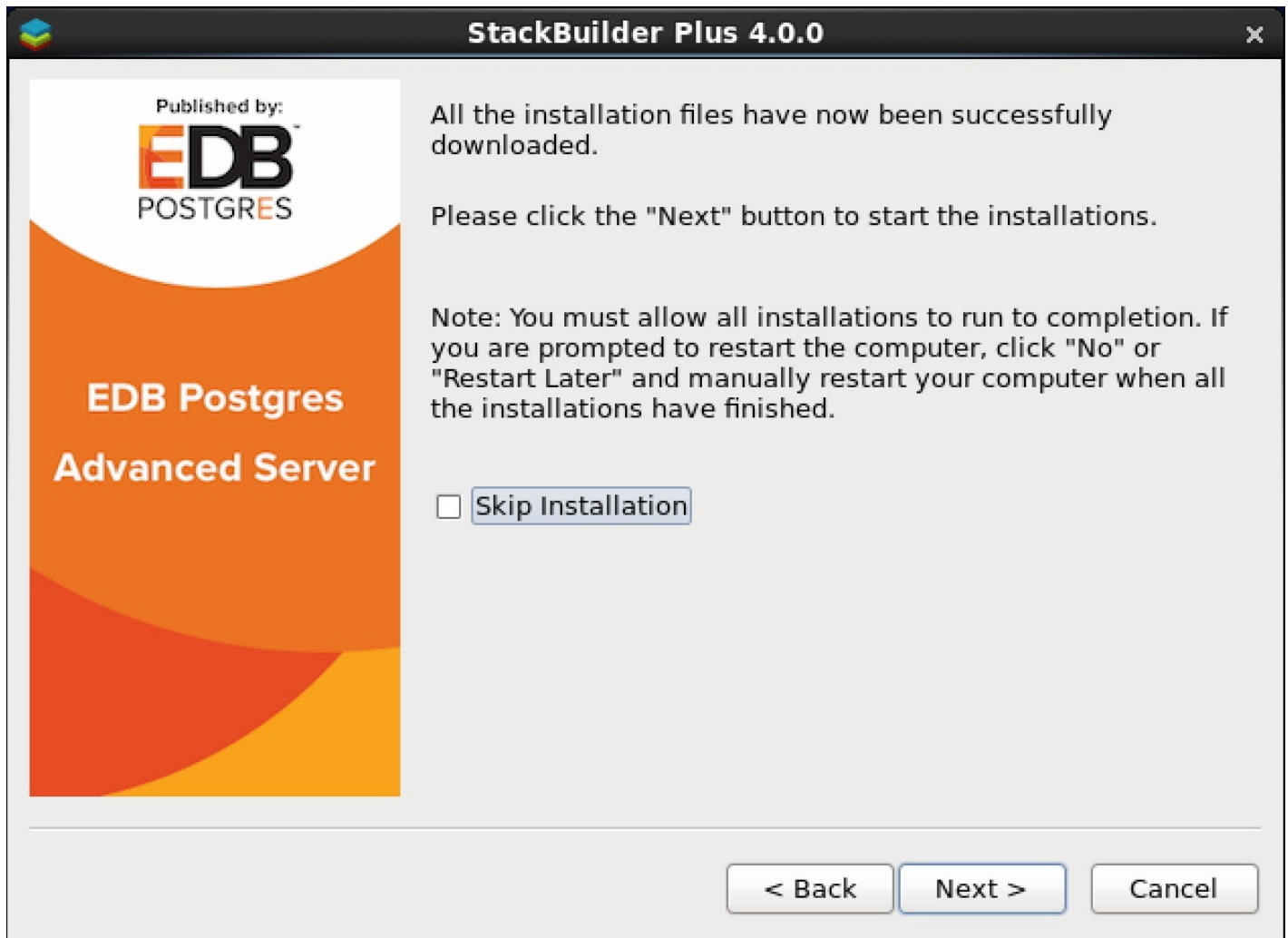
Figure 3-10: Start installation
