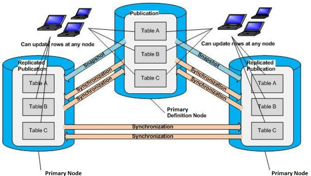
Figure 2-7: In a multi-master replication system, table rows can be updated at any primary node
