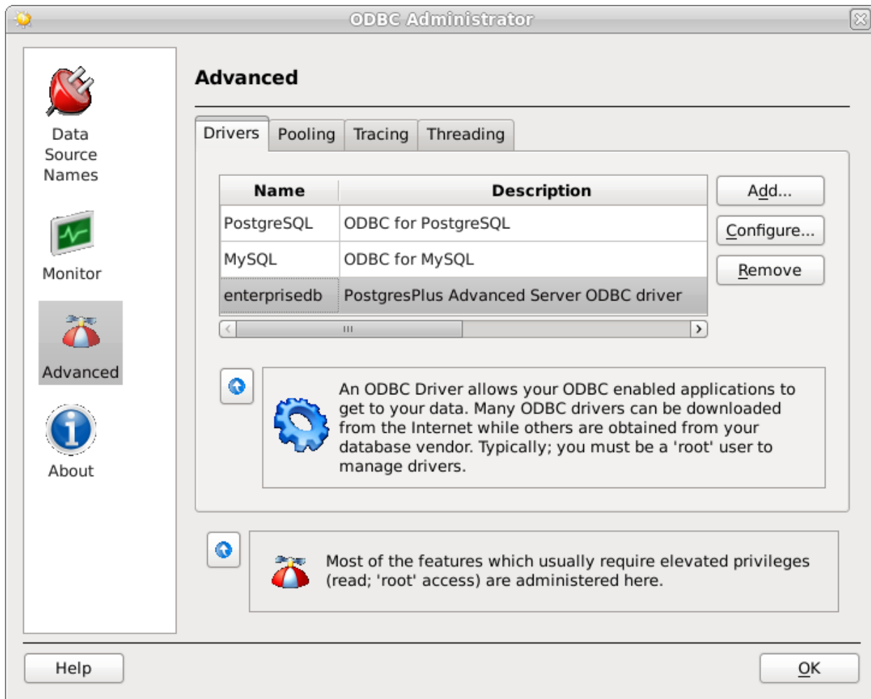
Fig. 9: The Drivers tab shows the installed EDB-ODBC driver
