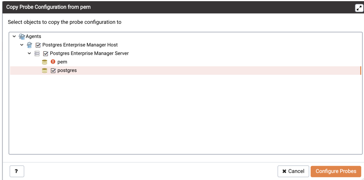
Fig. 4.27: The Copy Probe Configuration tree control
