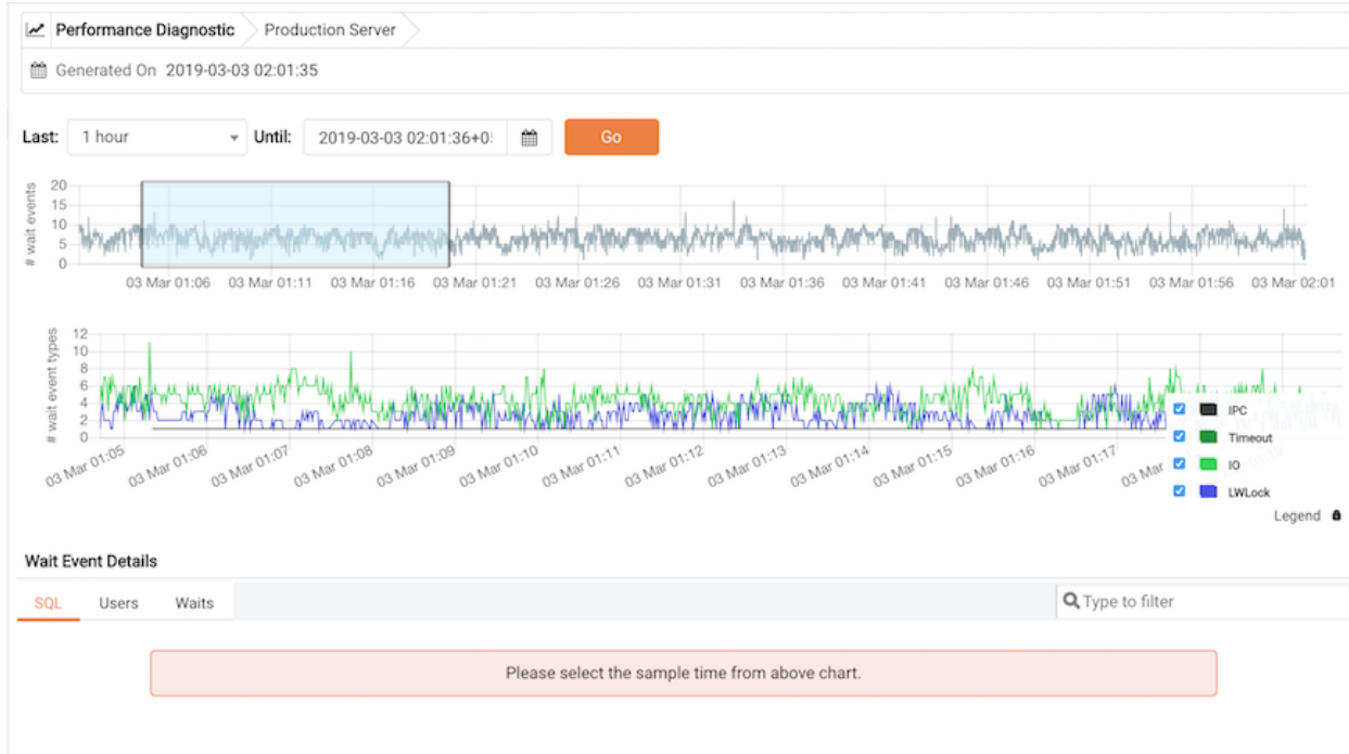
Fig. 15.4: Selecting a timeline
