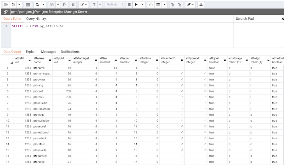
Fig. 1: Query Tool
