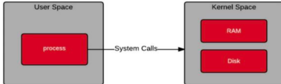
Figure 6.2: process Virtualization
