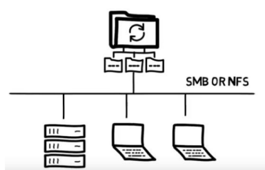
Figure 7.2: File Storage
