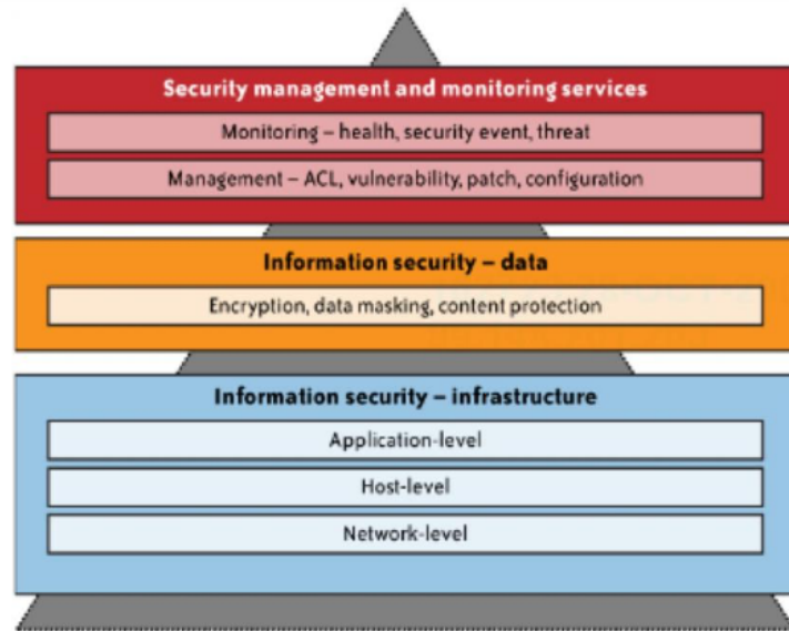
Figure 7.10: Cloud Security
