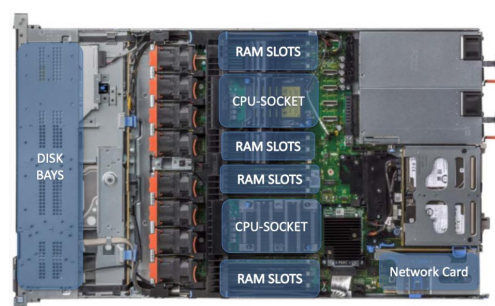
Figure 3.8: Node Components
