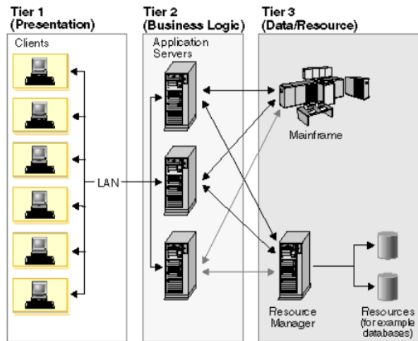
Figure 1.3: 3-tier architecture.
