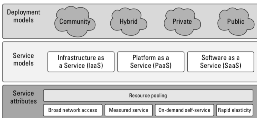
Figure 2.1: Cloud Computing Architecture
