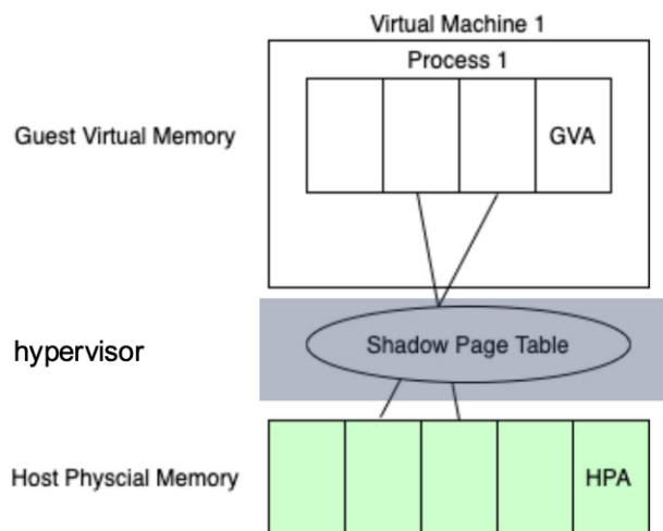
Figure 4.5: Shadow Page Table
