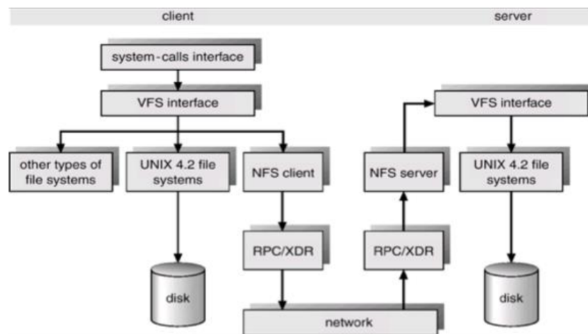
Figure 7.3: Distributed File System
