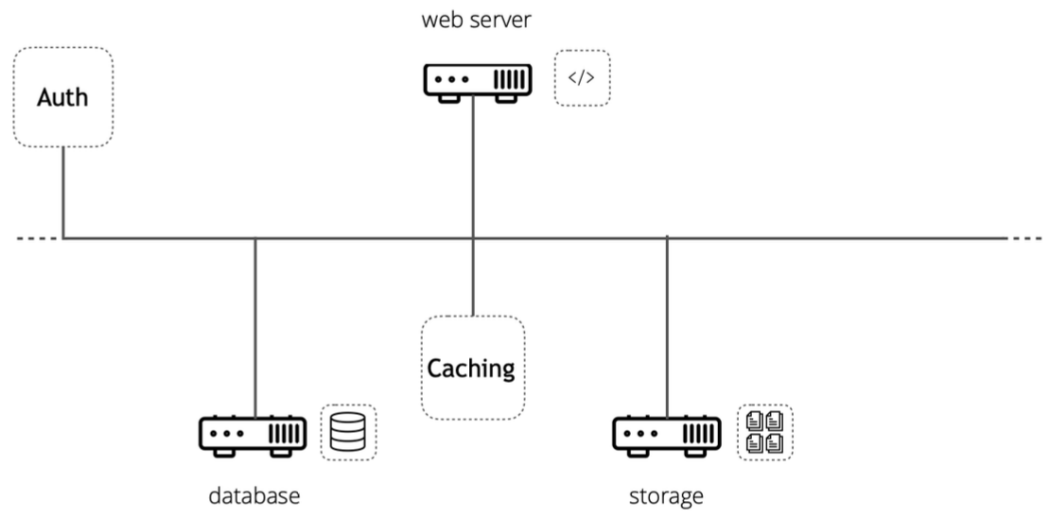
Figure 7.8: Cloud Storage Architecture
