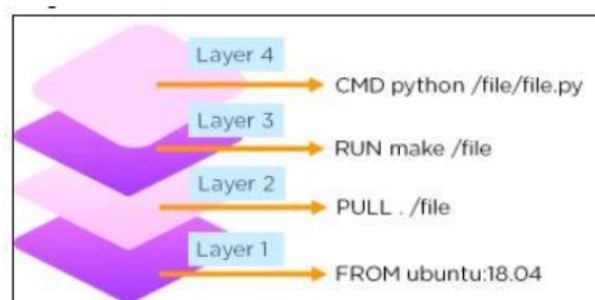
Figure 6.6: Docker Layers
