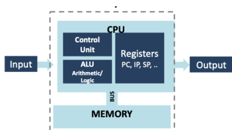
Figure 3.1: Serial Computer
