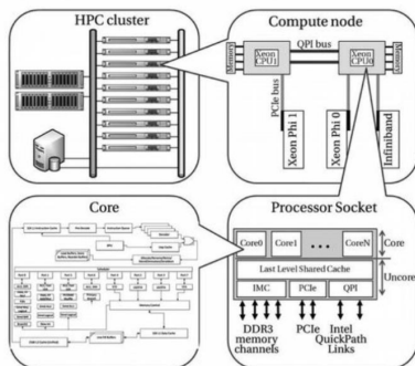
Figure 3.10: Computing Cluster
