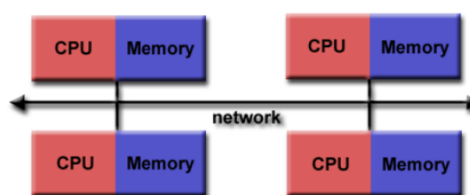
Figure 3.5: Distributed Memory
