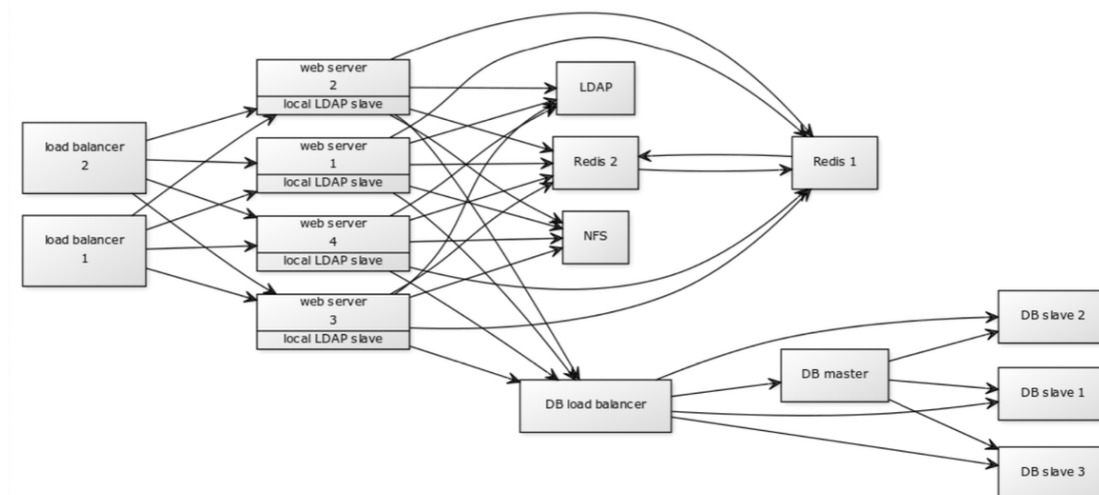
Figure 7.9: Production Deployment
