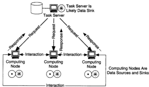
Figure 1.2: Distributed Computing.
