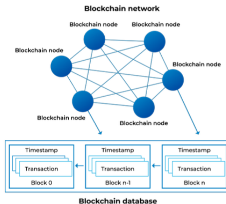
Figure 1.4: Peer-to-peer architecture.
