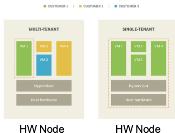
Figure 2.3: Resource pooling
