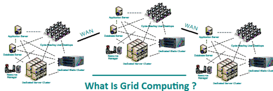
Figure 1.6: Grid Computing.
