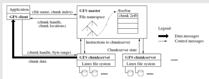
Figure 7.4: Google File System Architecture
