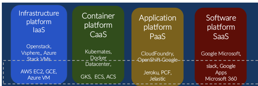
Figure 2.4: Cloud Service Models
