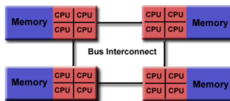
Figure 3.4: Non-Uniform Memory Access (NUMA)
