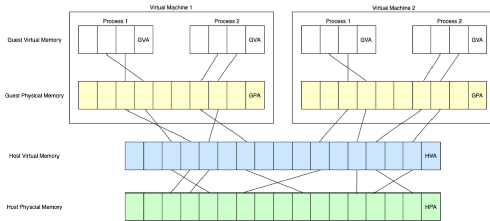
Figure 4.4: Memory virtualization
