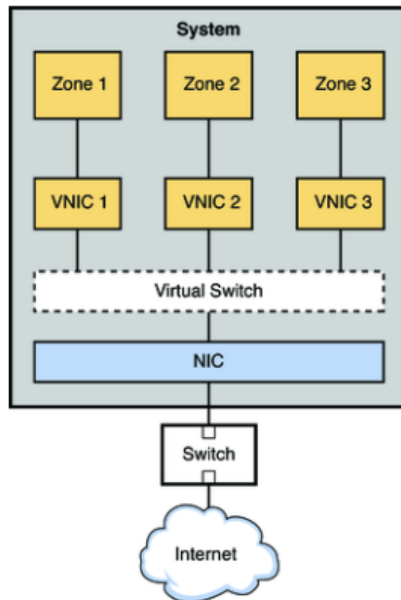
Figure 4.6: Network virtualization
