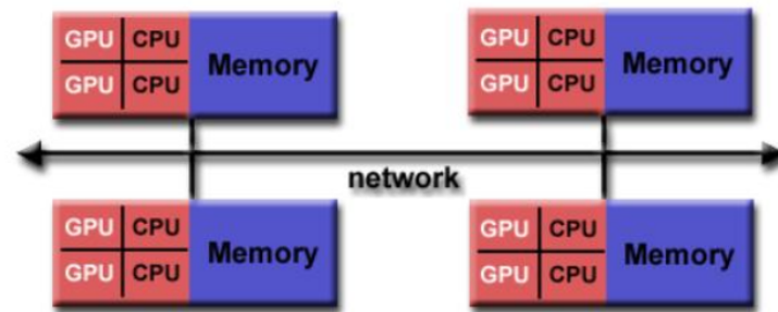
Figure 3.6: Computer Cluster
