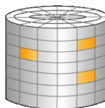
Figure 7.1: Block Storage
