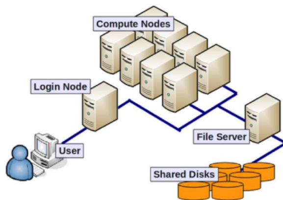
Figure 1.5: Computer Cluster.
