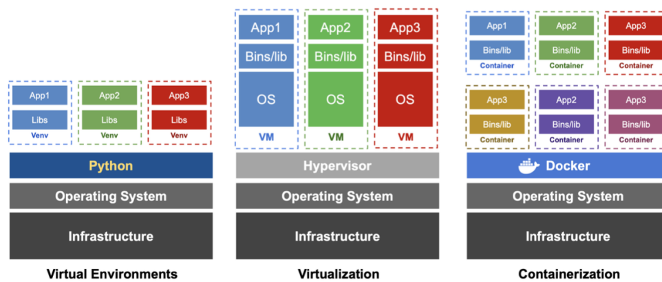
Figure 6.1: Comparison between Venvs, VMs and Containers
