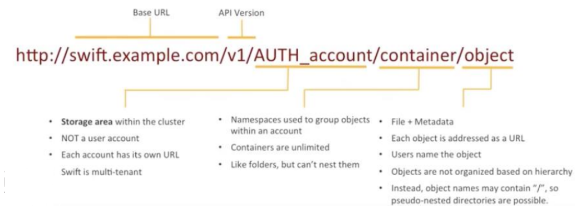
Figure 7.7: manage Object with HTTP
