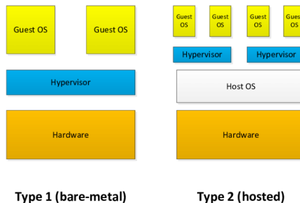
Figure 4.3: Virtualization models
