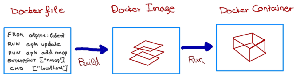
Figure 6.5: Dockerfile
