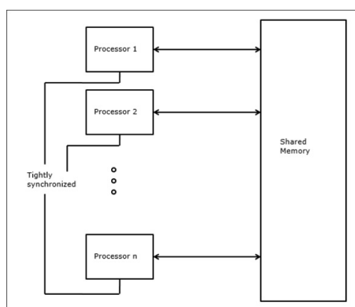
Figure 3.2: Parallel Computer
