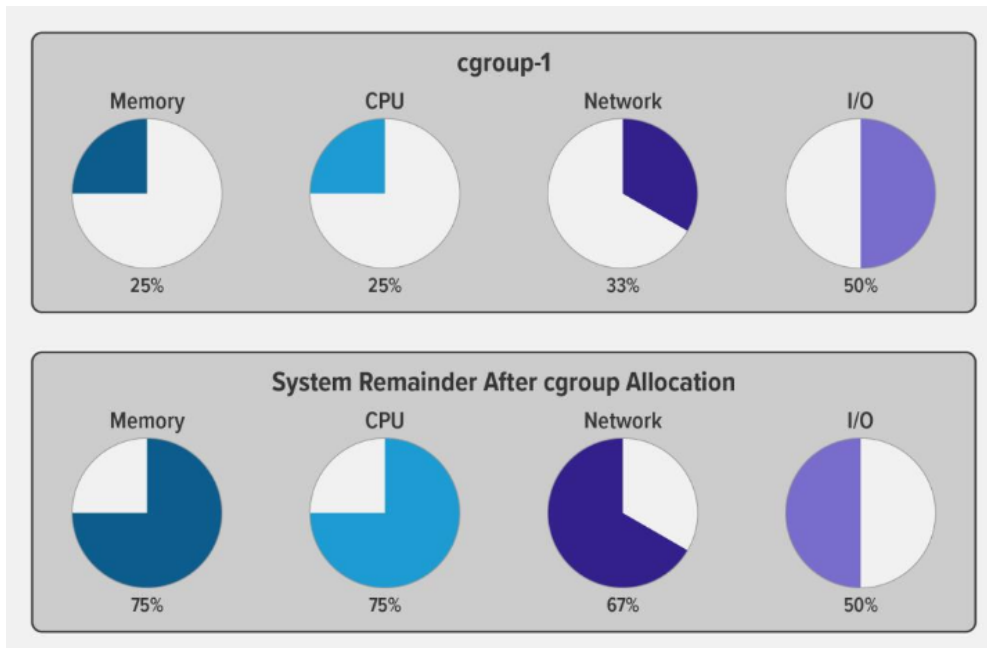
Figure 6.4: CGroups
