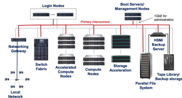
Figure 3.11: HPC cluster
