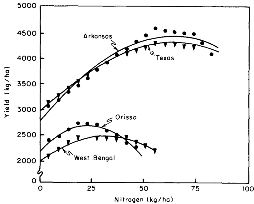
Figure 6.1. Yield response of rice to nitrogen fertilizer in two states of India and two states in the United States (Source: R. Herdt and J. Mellor, "The Contrasting Response of Rice to Nitrogen: India and the United States," American Journal of Agricultural Economics vol. 46, no. 1 [1964] p. 152, reprinted by permission of the publisher)
