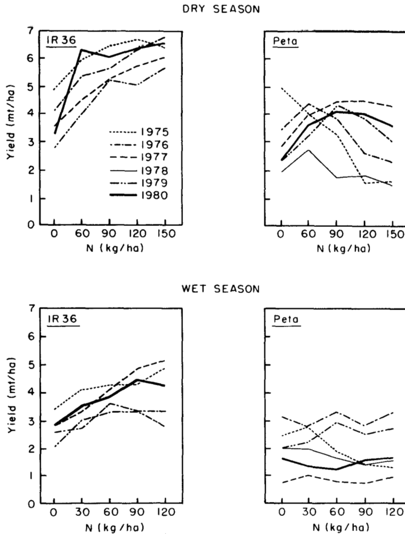
Figure 6.3. Nitrogen response of one modern (IR36) and one traditional rice variety (Peta) in trials at IRRI, 1975–80
