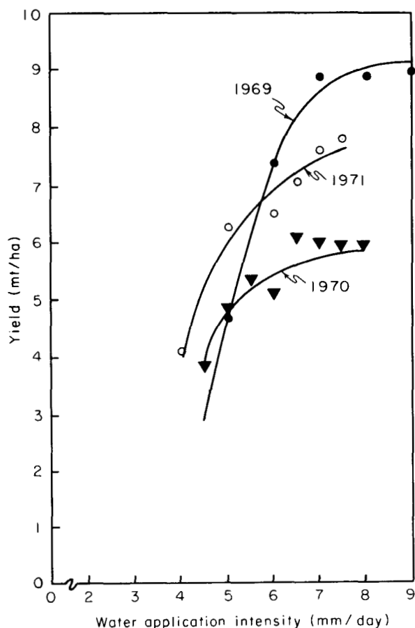
Figure 7.2. Functional relations (logistic functions) between rice yield and water application intensity for IR8 (100 kg/ha N) IRRRI, 1969, 1970, and 1971 dry seasons (Source: International Rice Research Institute, Annual Report for 1972 [Los Banos, Philippines, 1973] p. 58, reprinted by permission of the publisher)
