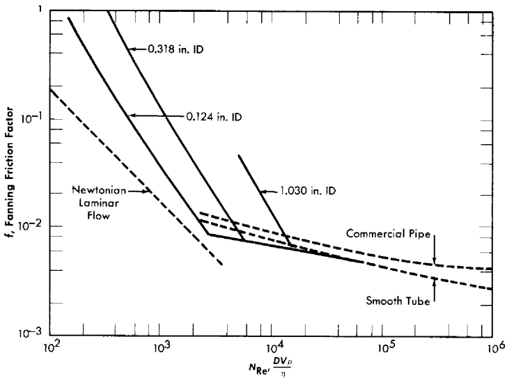
FIG. 4-19. Friction factor-Reynolds number data for \text{ThO}_2 slurries in turbulent flow. \tau_v = 0.075 \text{ lb/ft}^2 , \eta = 2.9 \text{ cp} .
