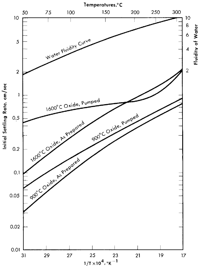
FIG. 4-11. Effect of firing temperature on high-temperature settling rates. 250 g Th/kg H_2O ; particle size 1 micron; prepared from 10^\circ C precipitated oxalate.
