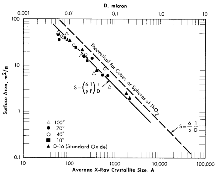
FIG. 4-5. Relationship between average crystallite size and specific surface area for thorium oxide prepared by the thermal decomposition of thorium oxalate (400 to 900°C firings).
