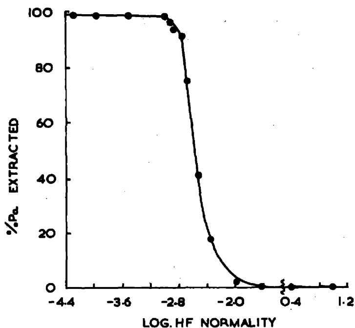
Fig. 2. Effect of HF on solvent extraction of Pa from hydrochloric acid (shown for di-isopropylcarbinol and 5.79 N HCl). (Nairn, J. S., Collins, D. A., McKay, H. A. C., and Maddock, A. G., Second U. N. Intl. Conf. on Peaceful Uses of Atomic Energy, A/CONF.15/P/1458).
