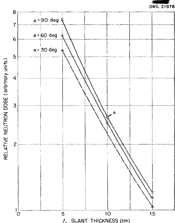
Fig. 12.2. Slant Penetration of Neutrons in Water.
