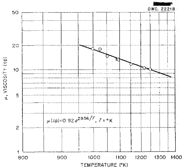
Fig. 8.2. Viscosity of Na 2 UF 6 as a Function of Temperature.
