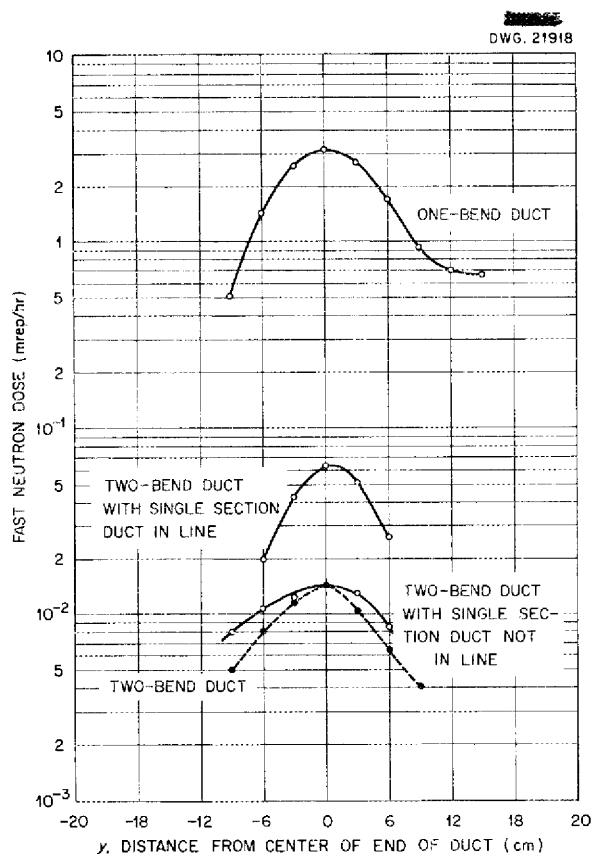
Fig. 12.3. Fast-Neutron Dose Beyond Various Configurations of Ducts with 45-deg Bends.
