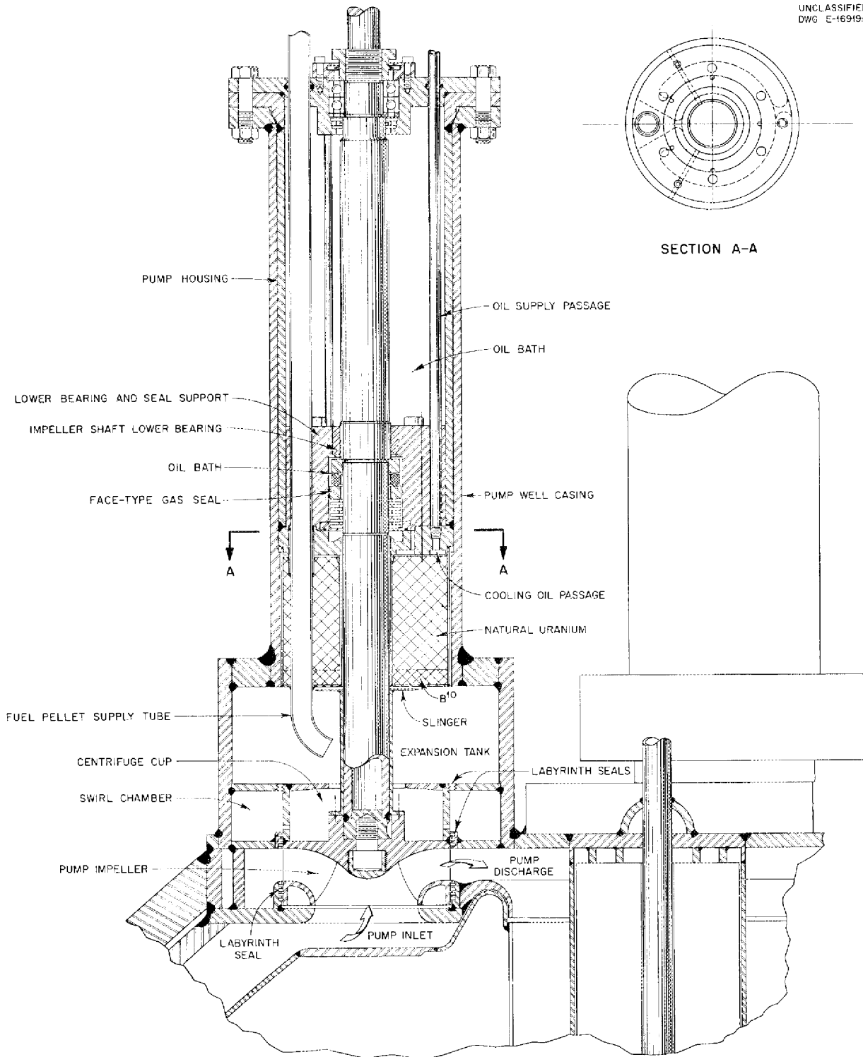
Fig. 3.4. Gas-Sealed Aircraft Pump.
