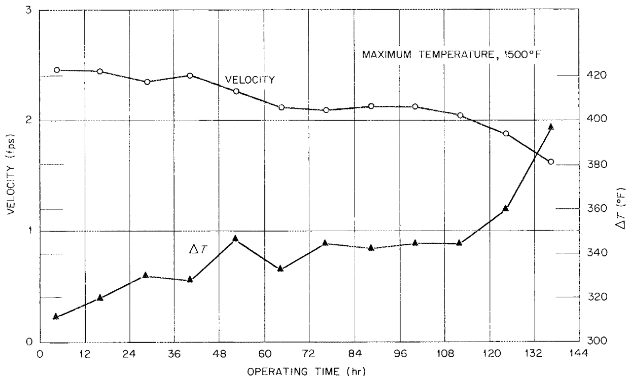
Fig. 2.3. Velocity and Temperature Difference as a Function of Operating Time for \text{NaF-ZrF}_4\text{-UF}_4 in an Inconel Forced-Circulation Corrosion Loop.
