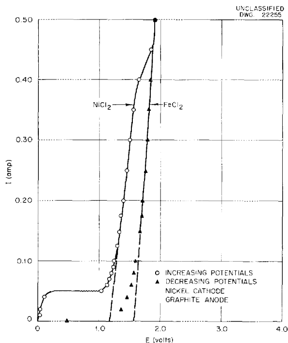
Fig. 5.5. Electrolysis at 850^\circ\text{C} of Mixture Containing 2 wt % of \text{NiCl}_2 and 2 wt % of \text{FeCl}_2 in KCl.
