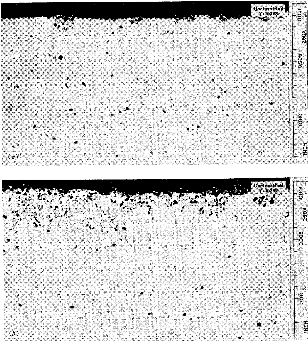
Fig. 6.1. Corrosion of Inconel after a 100-hr Seesaw Test at 815°C in the Fluoride \text{NaF-ZrF}_4\text{-UF}_4 (50-46-4 mole %) with and Without 3 wt% \text{MoS}_2 Additive. a. Tested with no additive. 250X. b. Tested with 3 wt % \text{MoS}_2 added. 250X.
