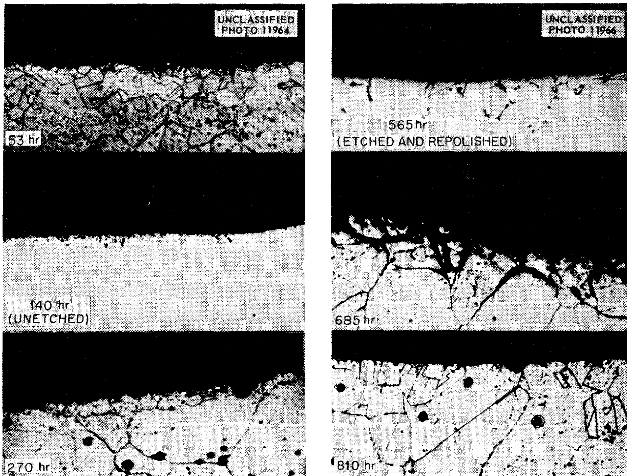
Fig. 9.1. Static Corrosion of Inconel by NaF-ZrF 4 -UF 4 (50-46-4 mole %) After Exposure at 1500°F in the LITR to 230 watts/cm 3 for Various Irradiation Times.
