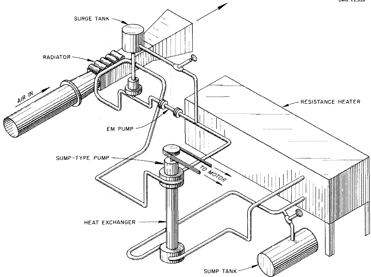
Fig. 2.2. Heat Exchanger Test Apparatus.
