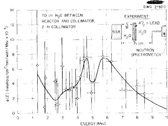
Fig. 11.5. Neutron Spectrum 70 cm from BSR.
