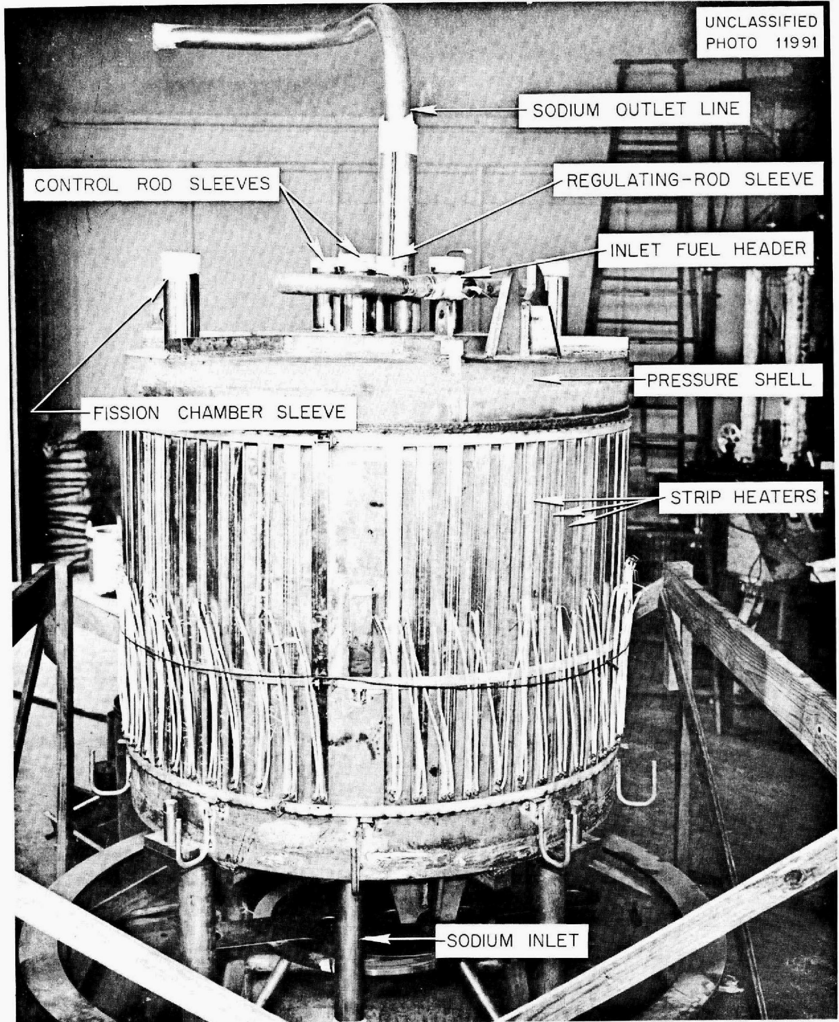
Fig. 1.1. Photograph of the Experimental Reactor.
