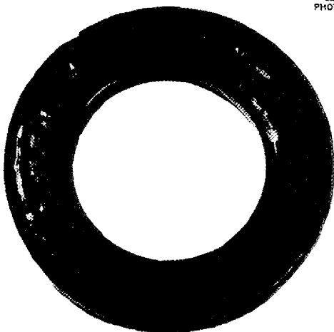
Fig. 7.10. Glass-Type Pump Seal. Composition (by weight): BeF 2 , 50%; KF, 25%; MgF 2 , 16%; AlF 3 , 9%.
