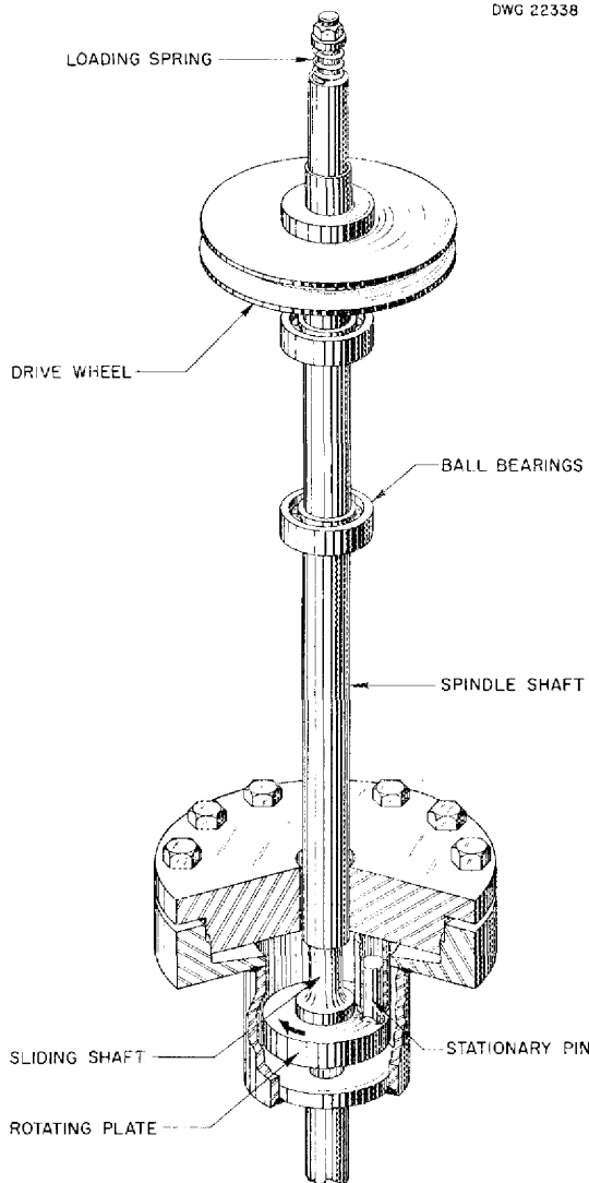
Fig. 2.1. Bearing Materials Compatibility Tester.
