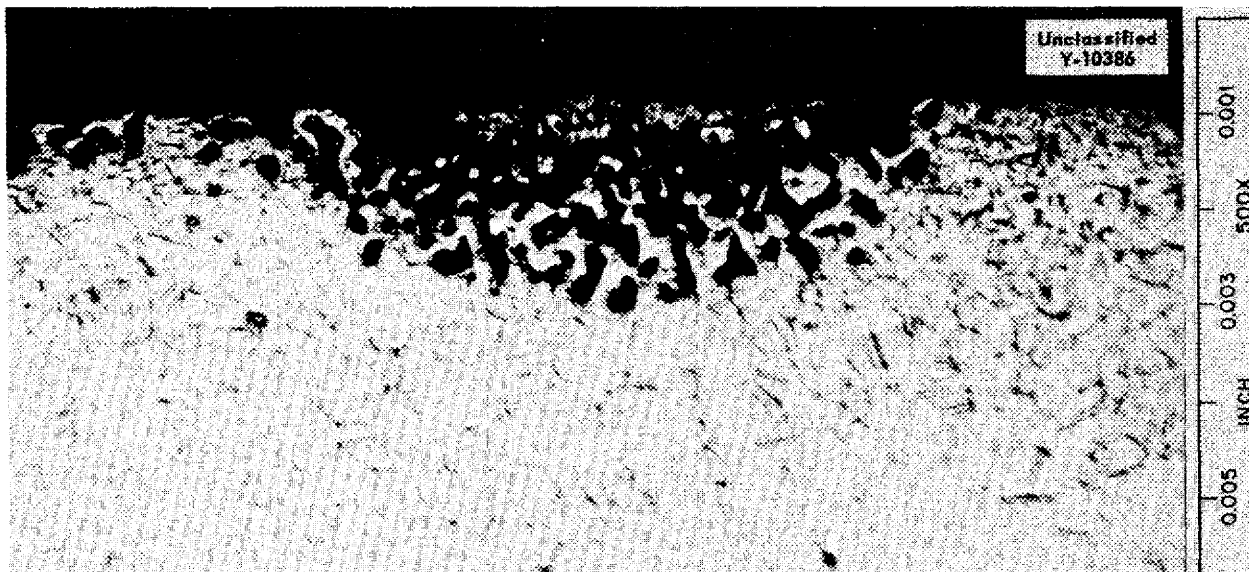
Fig. 6.7. Corrosion on Outer Surface of a Tubular Type 347 Stainless Steel Specimen Exposed to Circulating Lead in a Quartz Convection Loop for 550 hr at 815°C. 500X.
