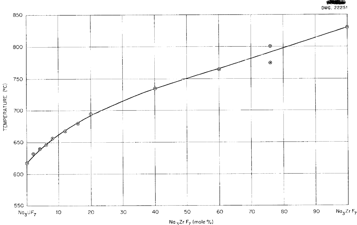
Fig. 5.1. The System \text{Na}_3\text{UF}_7 - \text{Na}_3\text{ZrF}_7
