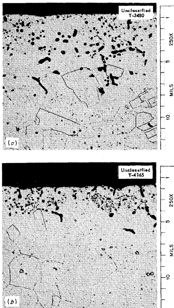
Fig. 6.3. Effect of Fluoride Batch Purity on the Corrosion of Inconel Exposed in Thermal Convection Loops to \text{NaF-ZrF}_4\text{-UF}_4 (50-46-4 mole %) for 500 hr at 1500^\circ\text{F} . a. Exposed to standard production batch. 250X. b. Exposed to high-purity batch. 250X. Reduced 17%.
