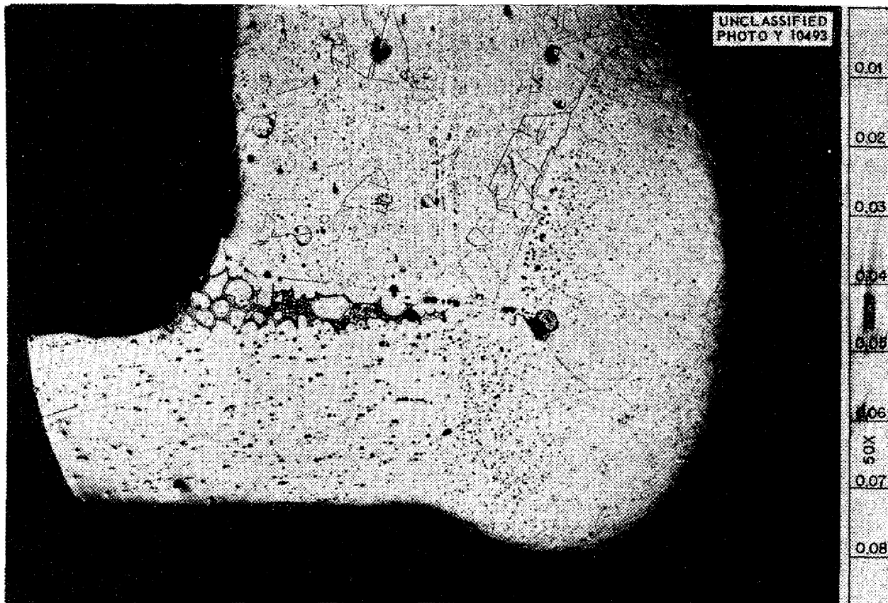
Fig. 7.3. Inconel Tube-to-Header Heliarc Welded Joint Backed Up with G-E No. 62 Brazing Alloy. Etchant: glyceria regia. 50X
