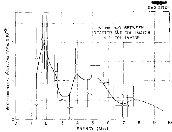
Fig. 11.4. Neutron Spectrum 50 cm from the BSR.
