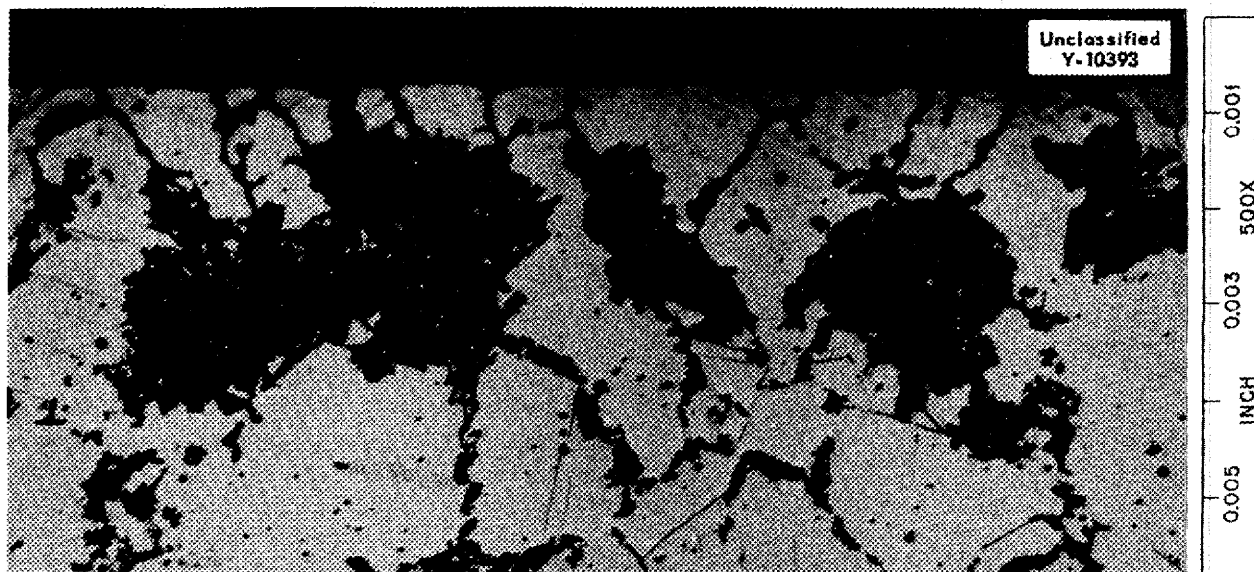
Fig. 6.6. Corrosion of a Molybdenum-Nickel (25% Mo-75% Ni) Alloy Specimen in a Quartz Thermal Convection Loop After Circulation of Lead for 672 hr at 820°C. 500X.
