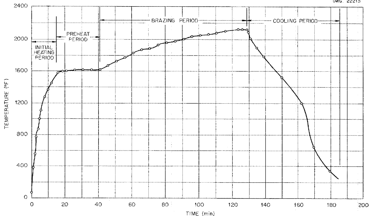
Fig. 7.4. Thermal Cycle Employed in Furnace Brazing a Heat Exchanger with G-E No. 62 Alloy. Temperatures were obtained with a chromel-alumel thermocouple secured to the heat exchanger.
