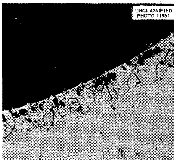
Fig. 9.3. Static Corrosion of Inconel by NaF-ZrF 4 -UF 4 (50-46-4 mole %) After Irradiation in the MTR at 2500 watts/cm 3 for 575 hr at 1500°F.
