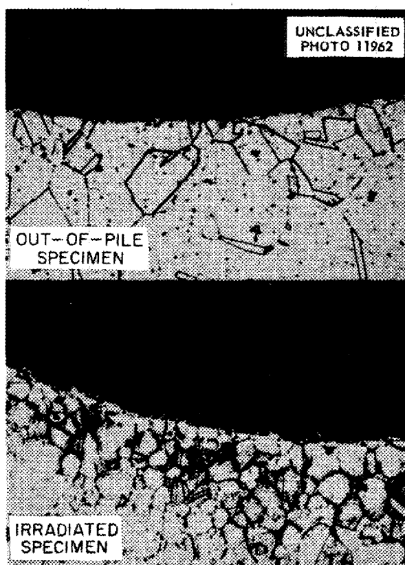
Fig. 9.4. Static Corrosion of Inconel by NaF-ZrF 4 -UF 4 (53.5-40-6.5 mole %) After 419 hr at 1500°F With and Without Irradiation in the MTR at 3900 watts/cm 3 .
