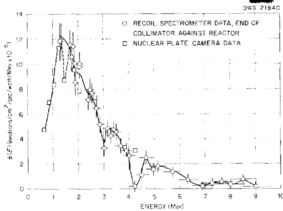
Fig. 11.3. Neutron Spectrum at the Face of the BSR.
