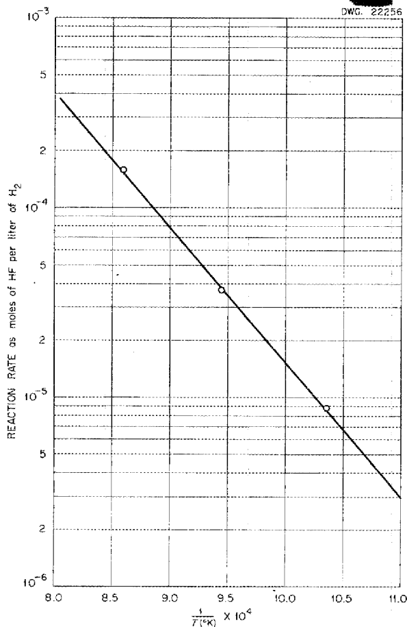
Fig. 5.6. Reaction Rate vs. Reciprocal Temperature According to the Equation UF_4 + \frac{1}{2} H_2 = UF_3 + HF .
