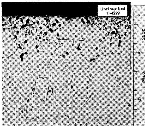
Fig. 6.4. Corrosion of Inconel Thermal Convection Loop by High-Purity NaF-ZrF 4 -UF 4 (53.5-40.0-6.5 mole %) After 500 hr at 1500°F. 250X. Reduced 15%.
