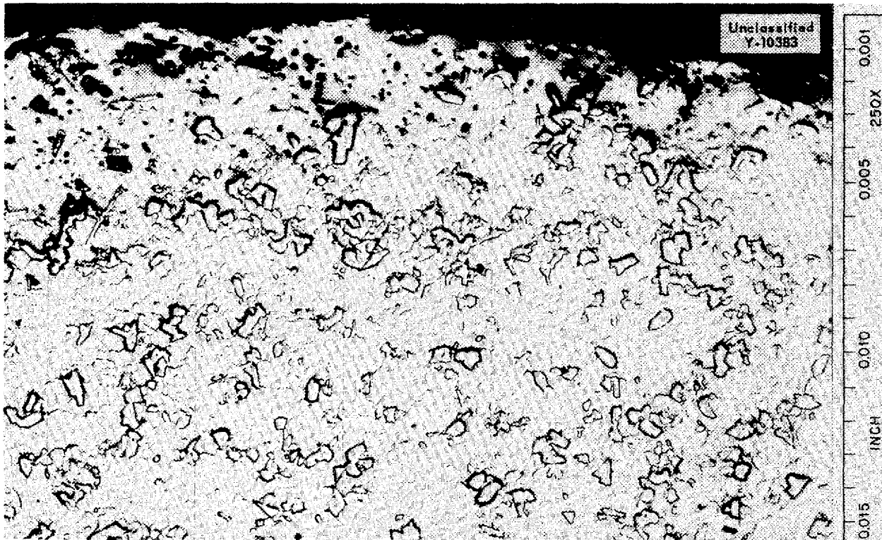
Fig. 6.2. Stellite 40 After Static Testing in NaF-ZrF 4 -UF 4 (50-46-4 mole %) for 100 hr at 816°C.
