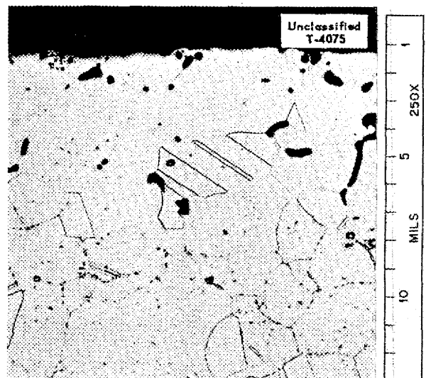
Fig. 6.5. Corrosion of Inconel Thermal Convection Loop by NaZrF 5 After 500 hr at 1500°F. 250X. Reduced 12%.
