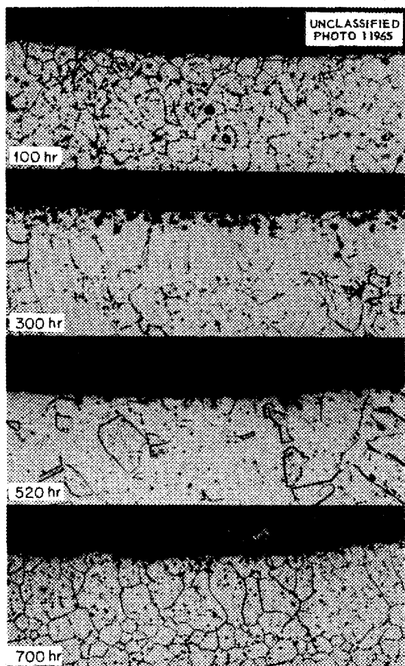
Fig. 9.2. Static Corrosion of Inconel Exposed to NaF-ZrF 4 -UF 4 (50-46-4 mole %) at 1500°F for Various Times.
