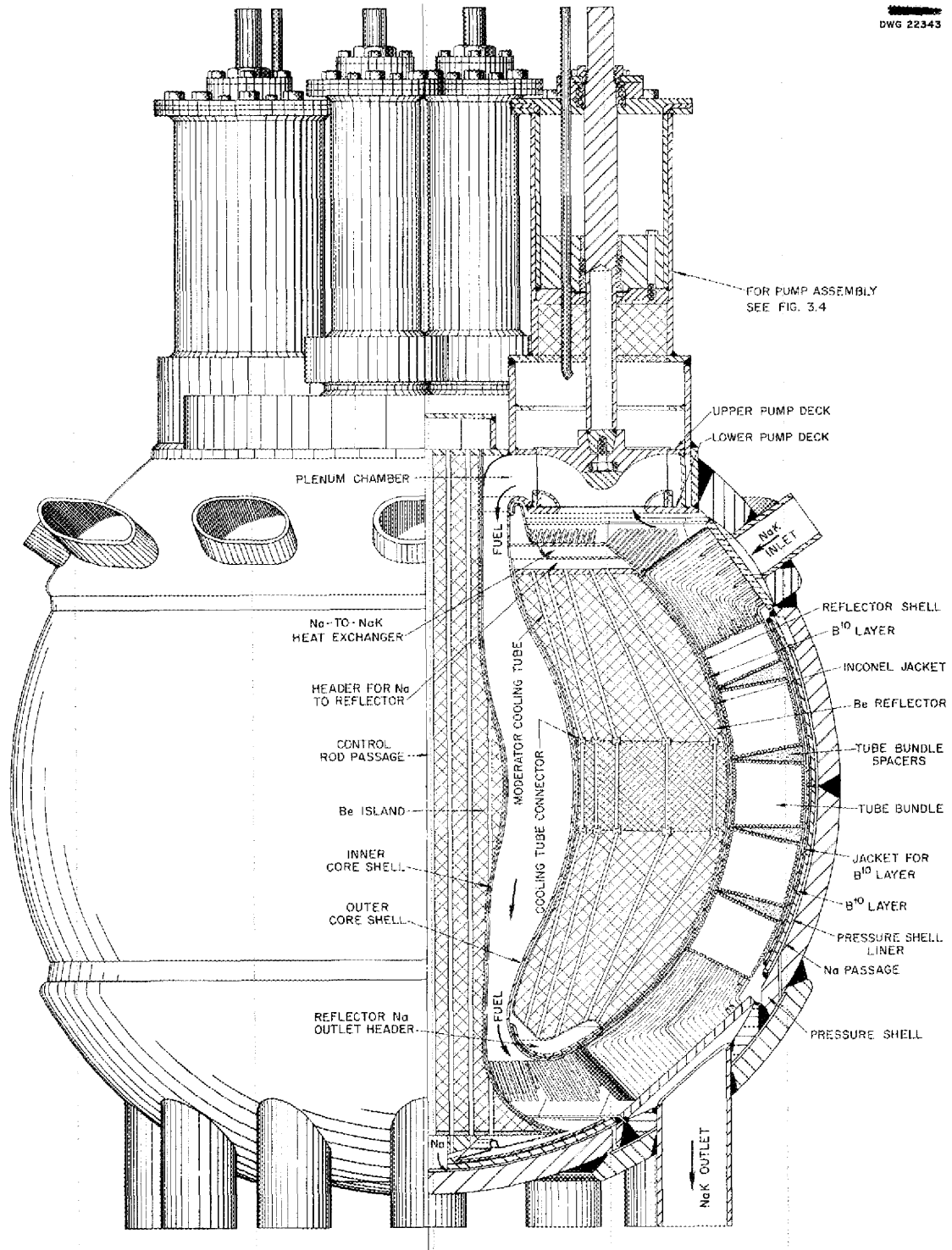
Fig. 3.3. 300-Megawatt Reflector-Moderated Reactor.
