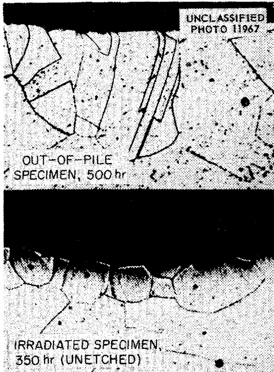
Fig. 9.5. Static Corrosion of Inconel by NaF-ZrF 4 -UF 4 (63-25-12 mole %) at 1500°F With and Without Irradiation in the MTR at 8000 watts/cm 3 .
