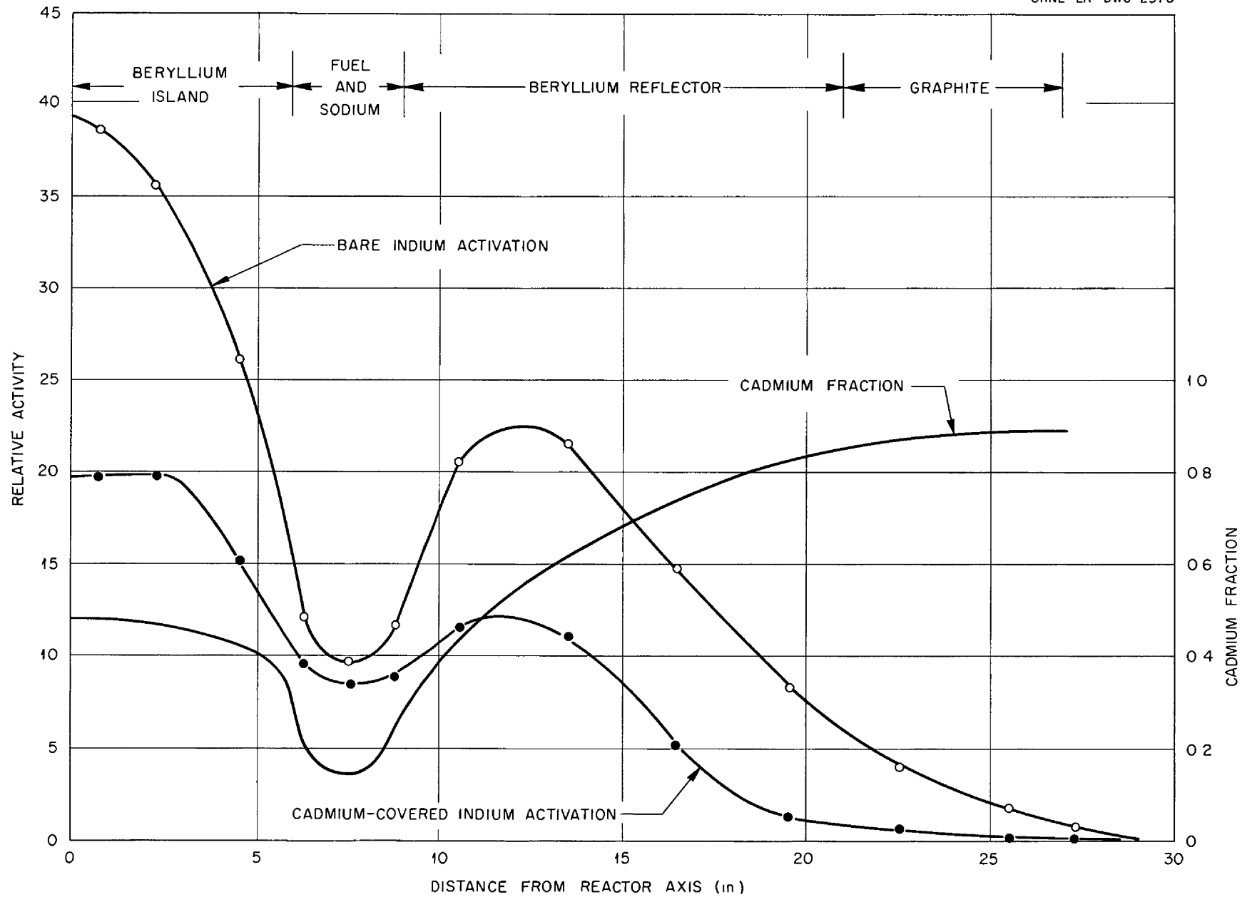
Fig III-10 Indium Traverse Radially in Midplane of Reactor Cell O-12 to X-12
