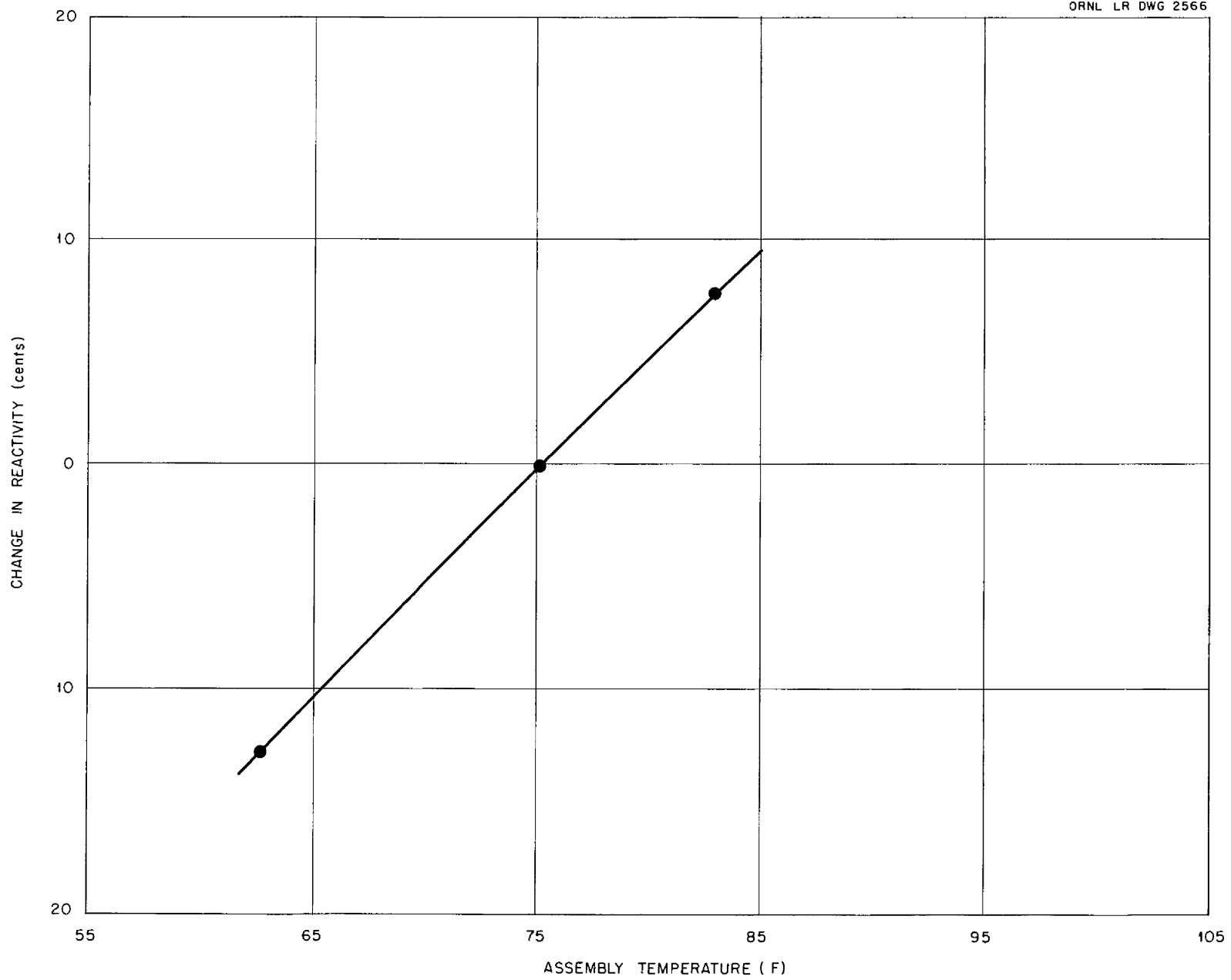
Fig III 6 Change in Reactivity vs Temperature
