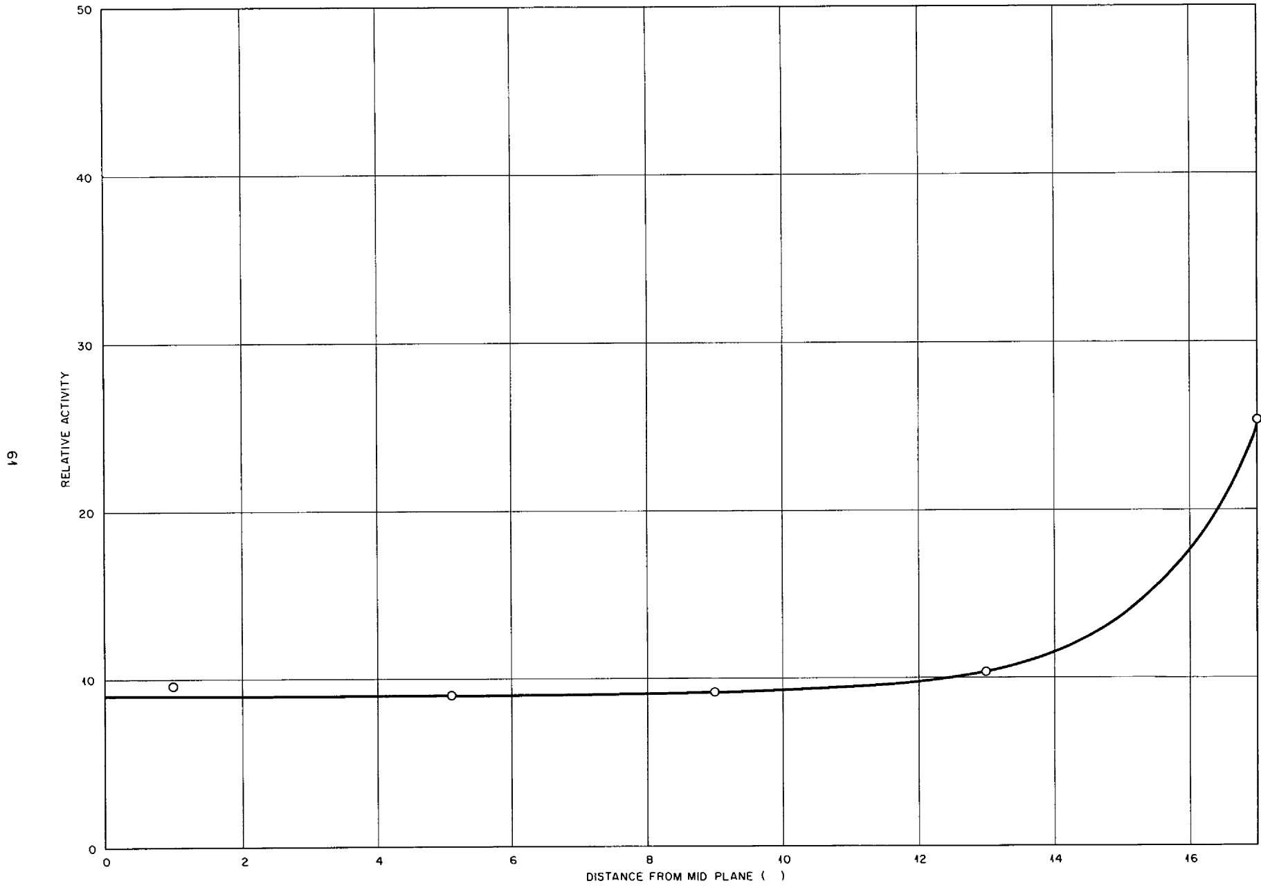
Fig VI 4 Axial Power Distribution Through M 12
