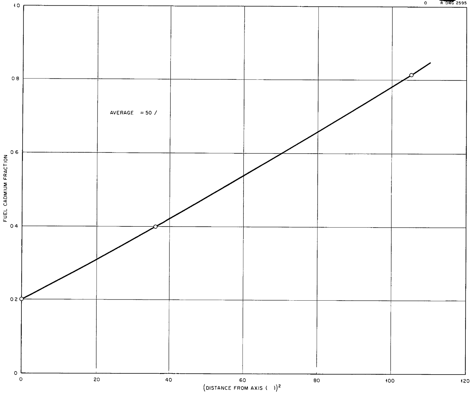
F g VI 5 Radial Fuel Cadmium Fractions
