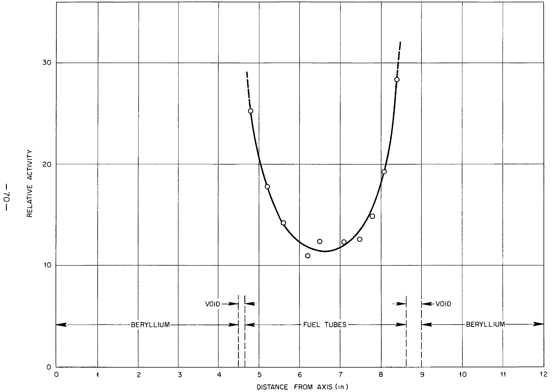
Fig VII-5 Power Distribution across Fuel Annulus at Mid-plane
