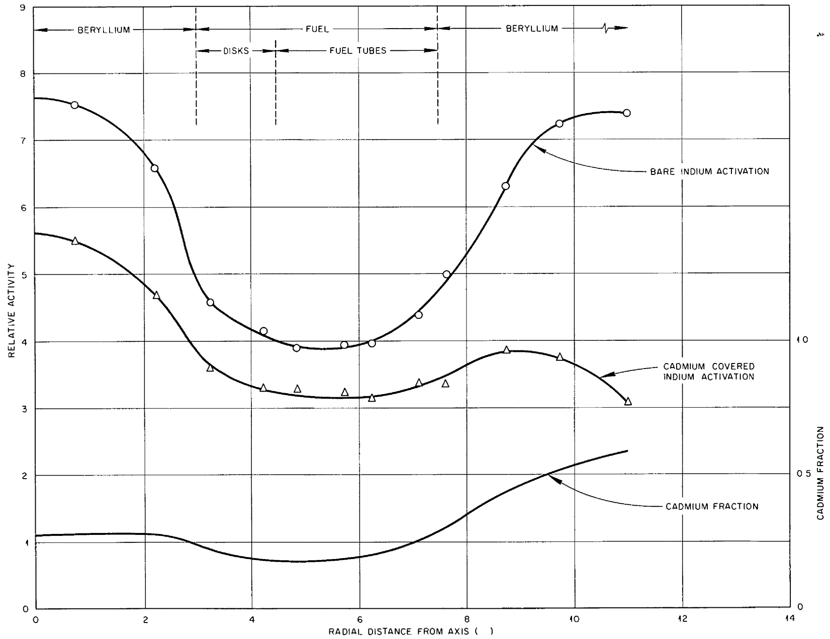
Fig IV 6 Radial Flux Distribution 6 1/4 in from Mid plane
