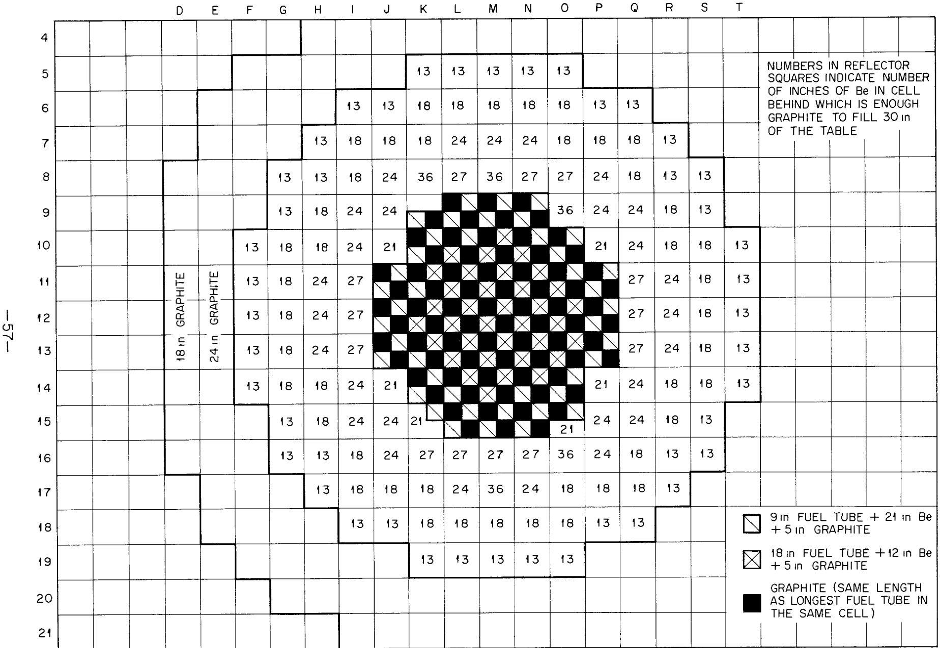
Fig VI-1 Assembly Loading at Mid-plane
