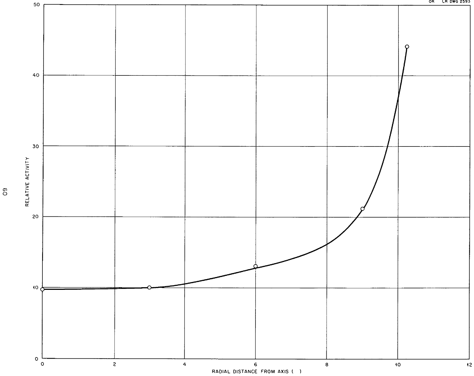
Fig VI 3 Rad al Power Distribution in Mid plane
