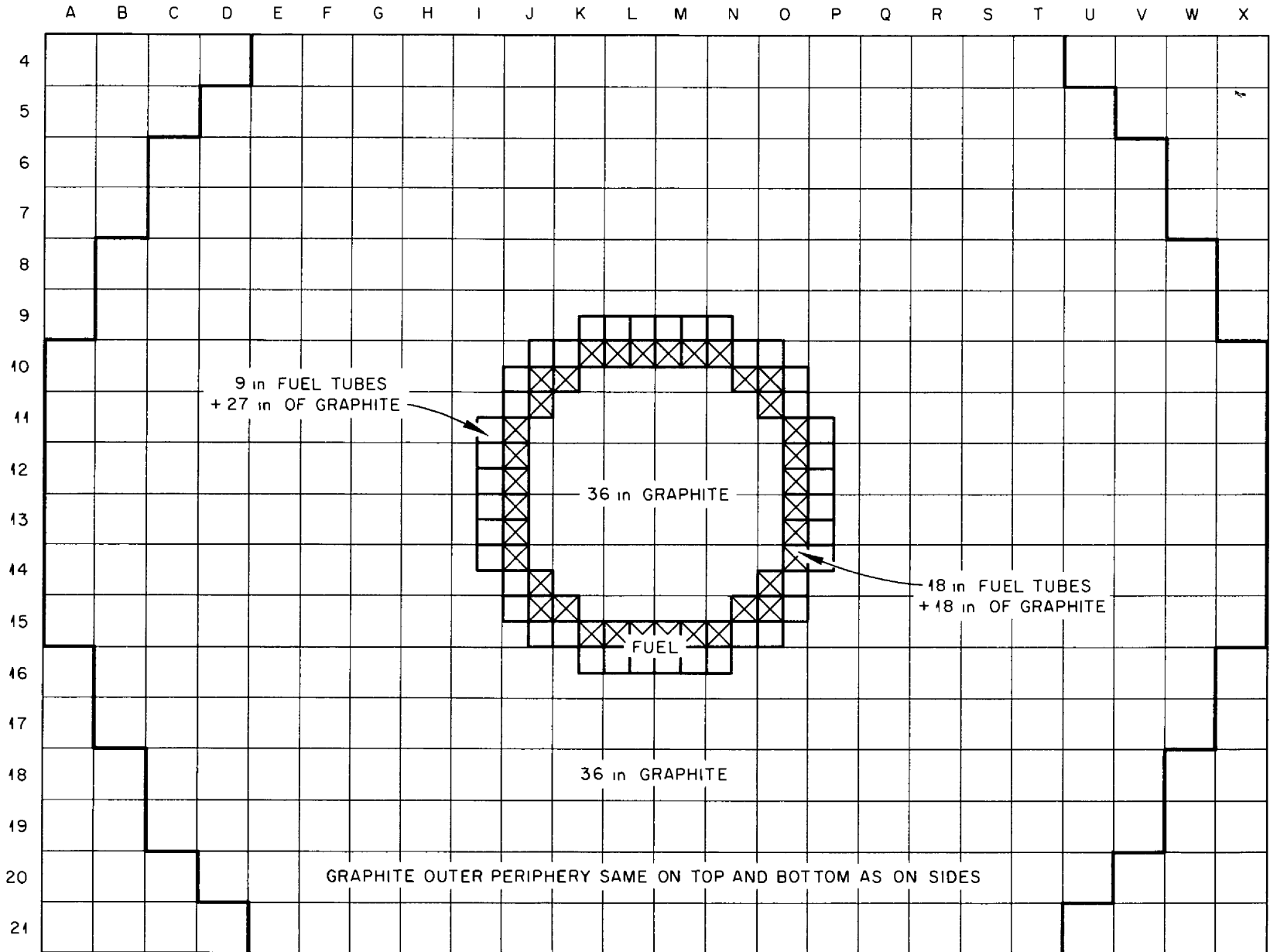
Fig V-1 Assembly Loading at Mid-plane
