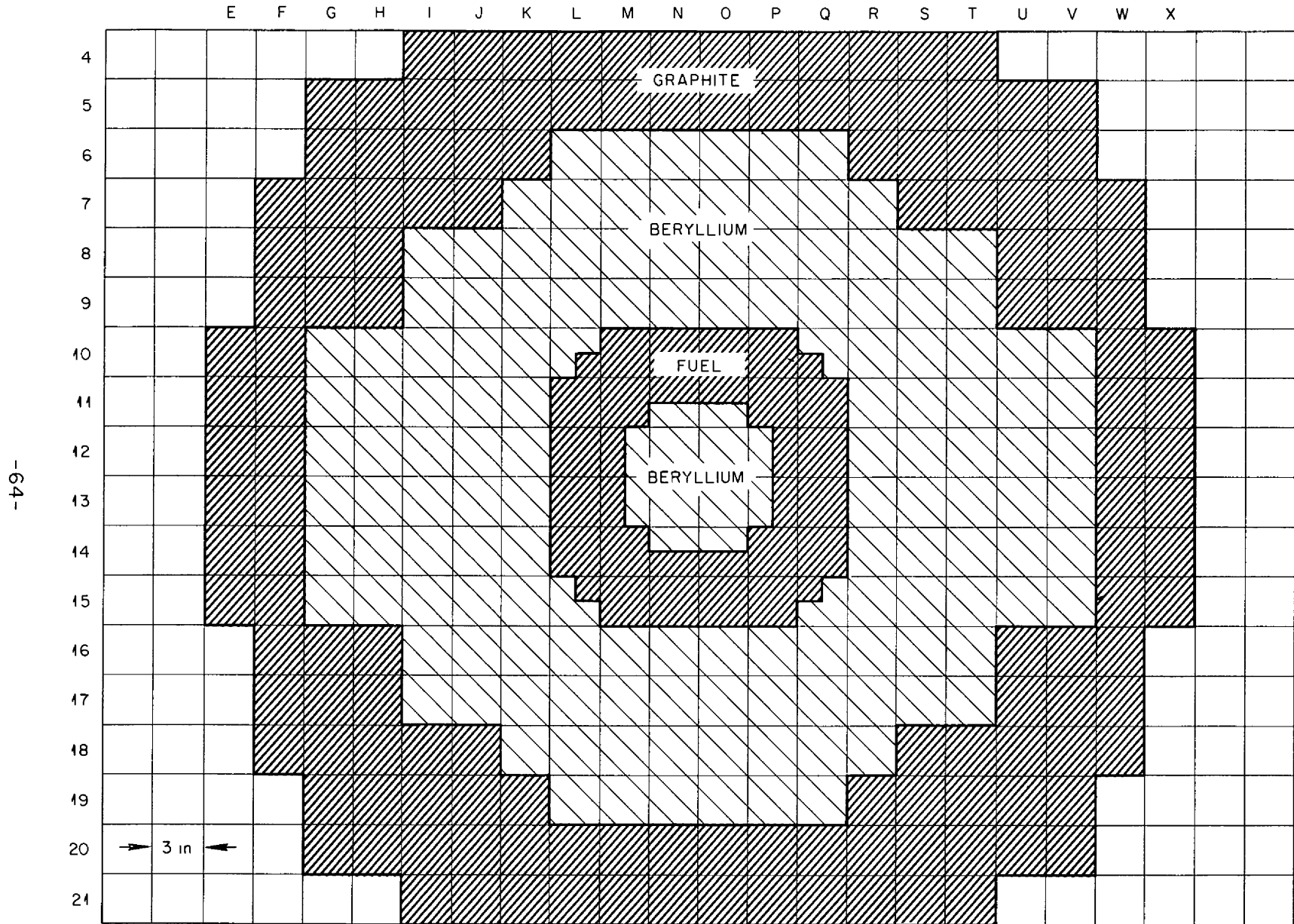
Fig VII-1 Assembly Loading at Mid-plane (No Structure Shown)
