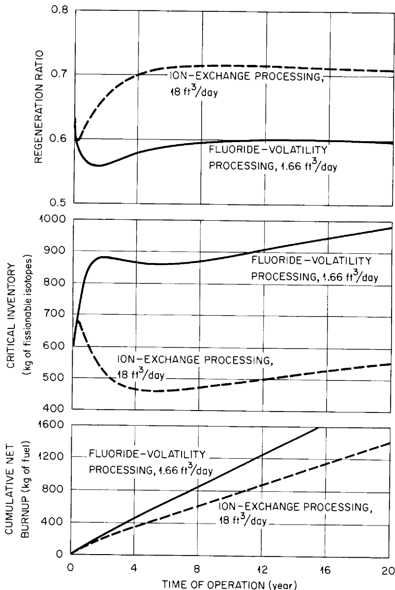
Fig. 1.1.13. Long-Term Performance of Spherical, Homogeneous, Two-Region, Molten-Fluoride-Salt Reactor Fueled With U 235 .
