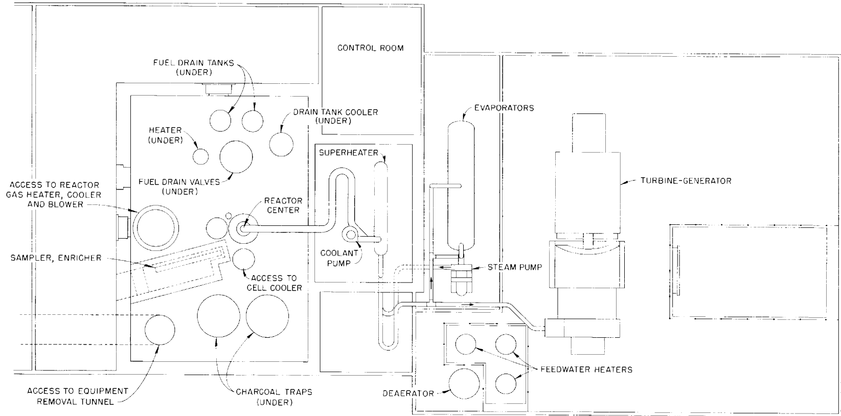
Fig. 1.1.3. Plan Drawing of Power Plant for 30-Mw, Experimental, Molten-Salt Reactor.
