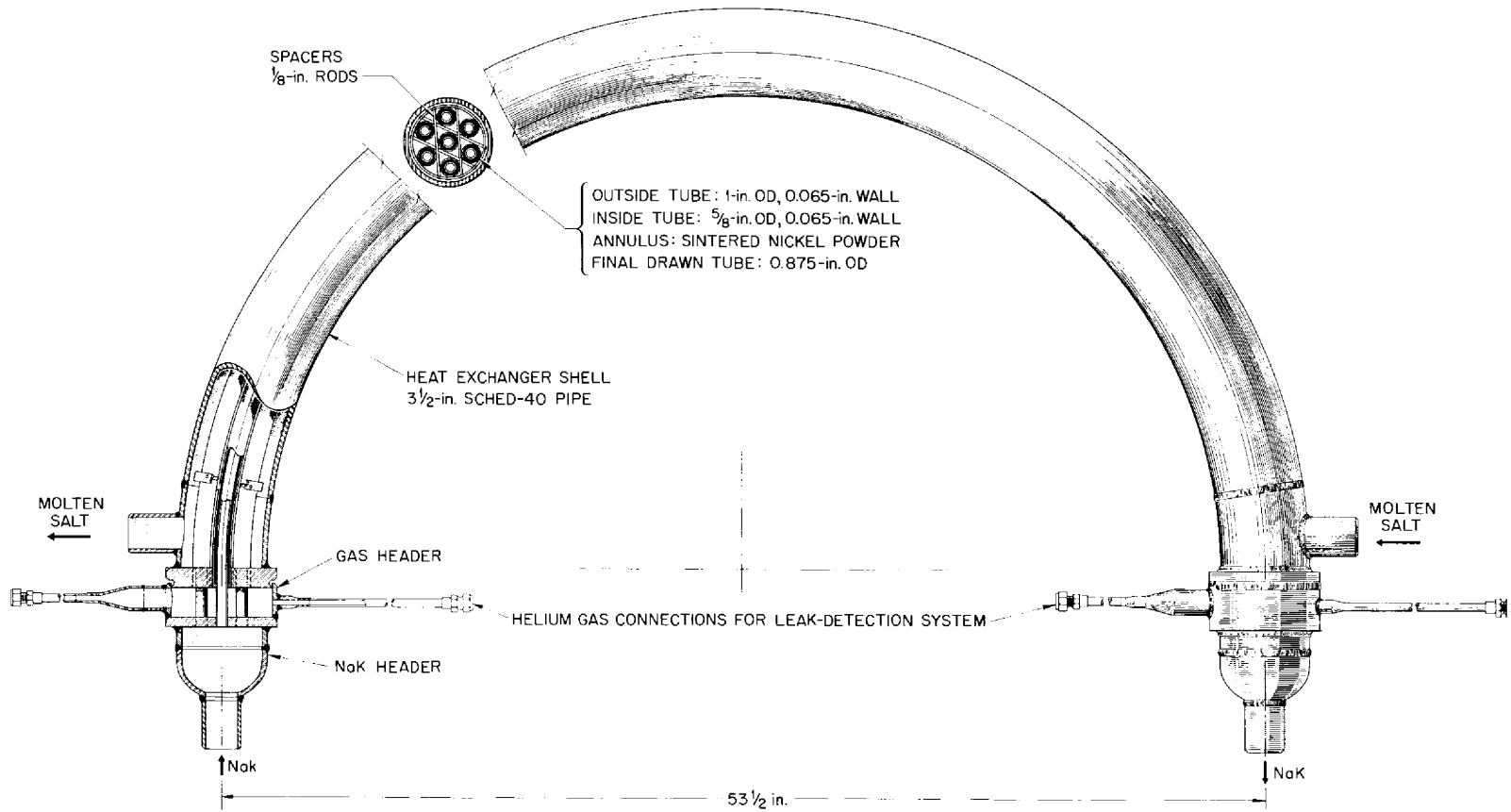
Fig. 1.2.8. Triplex Tubing Heat Exchanger.
