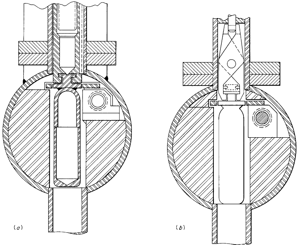
Fig. 1.1.6. (a) Sampling-Pot Elevator Showing Plunger Under a Sampling Can. (b) Sample-Depositing Elevator Showing Tongs.
