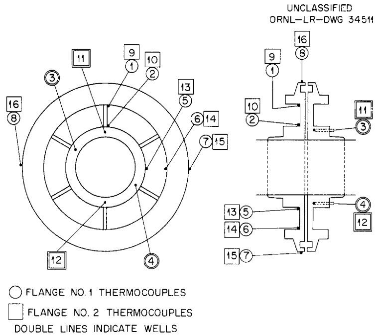
Fig. 1.2.5. Diagram of Large Freeze-Flange Mechanical Joint Showing Location of Thermocouples.
