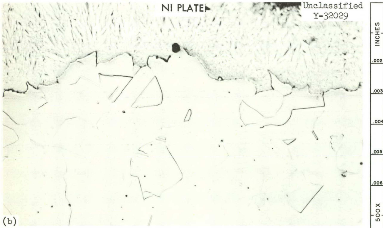
Fig. 93. Cross Sections of Gas Disposal Unit Inlet Pipe (a) Photomicrograph Showing Severe Pitting Attack. 15X. (b) Portion of Fig. 93A showing typical surface at base of pit. 500X. Etchant: Acetic-nitric-hydrochloric acid.
