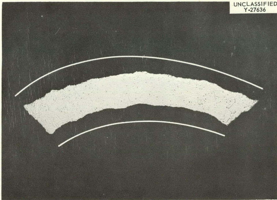
Fig. 77A. Cross Section of Salt Region Sample from Nimonic 80 Corrosion Specimen (Runs L-5-L-9:7). Interior of white lines indicates original thickness. As-polished. 10X.
