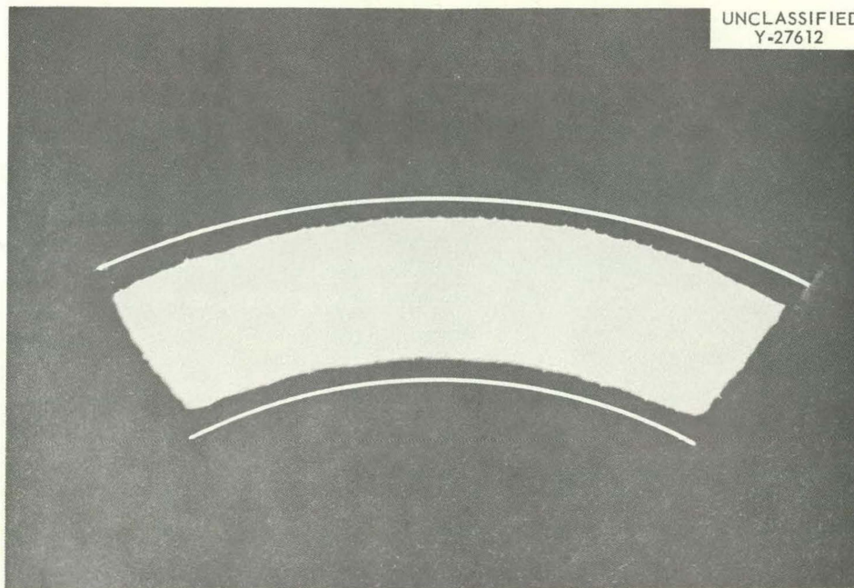
Fig. 75A. Cross Section of Interface Region Sample from Hastelloy X Corrosion Specimen (Runs L-5-L-9:5). Interior of white lines indicates original thickness. As-polished. 10X.
