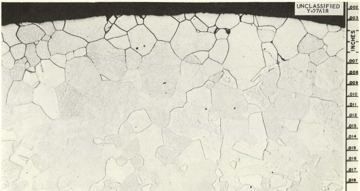
Fig. 59B. Portion of Fig. 59A. Typical Surface and Microstructure. Note intergranular attack. Etchant: \text{KCN}-(\text{NH}_4)_2\text{S}_2\text{O}_8 . 200X.
