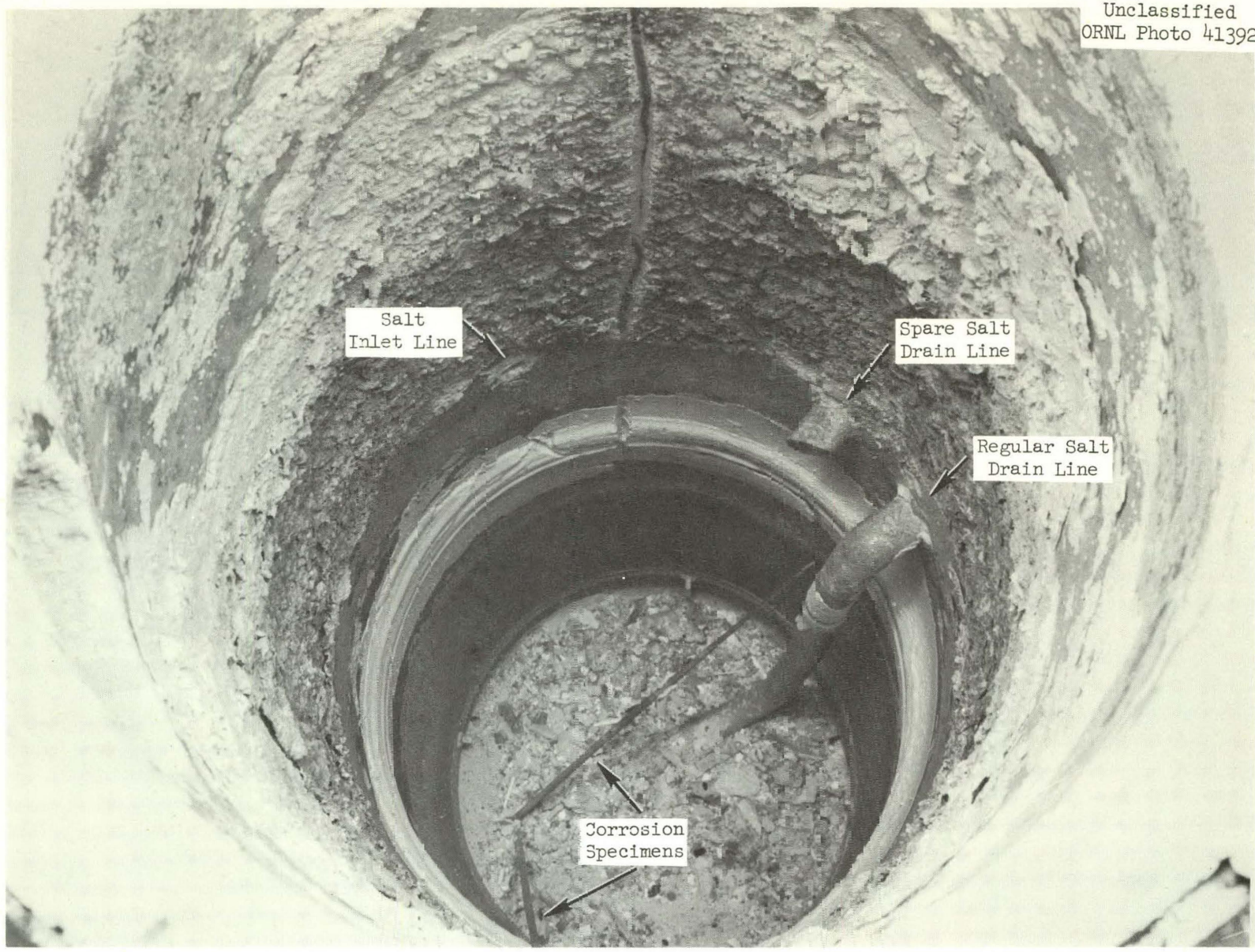
Fig. 5. Interior of the Mark I Volatility Pilot Plant FLorinator After Run C-15.
