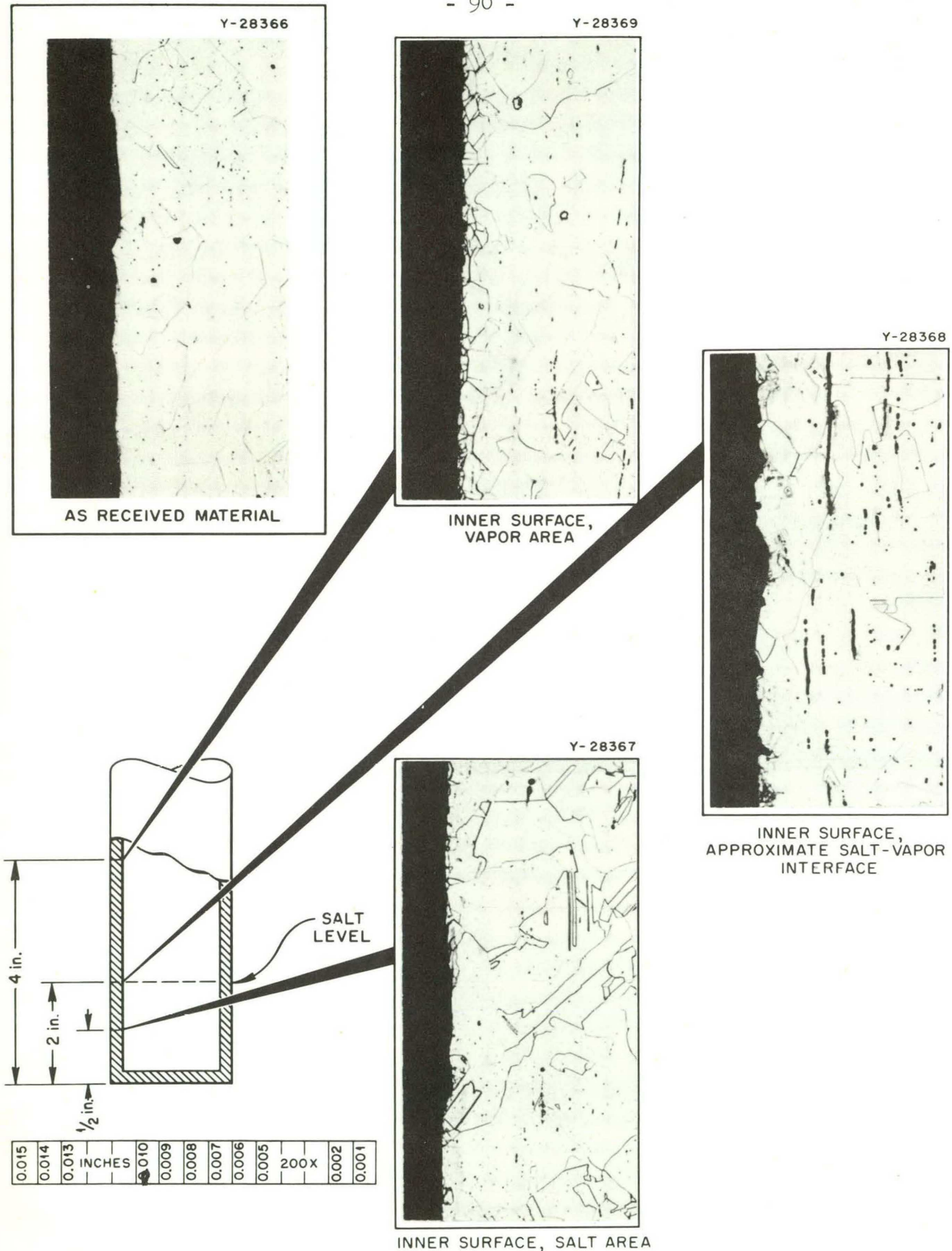
Fig. 38. Typical Microstructures of Samples from A Nickel Miniature Test Fluorinator No. 1. Etchant: Acetic-nitric-hydrochloric acid. 200X.
