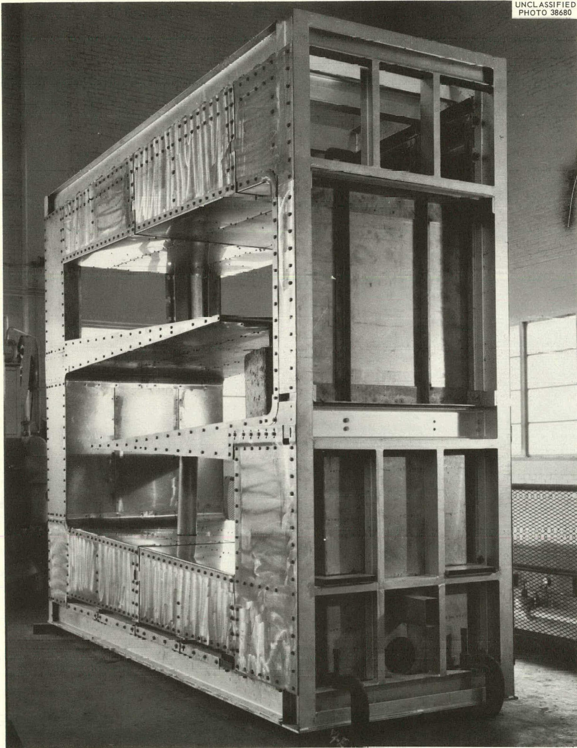
Fig. 1.7. Coolant Salt Drain Tank.
