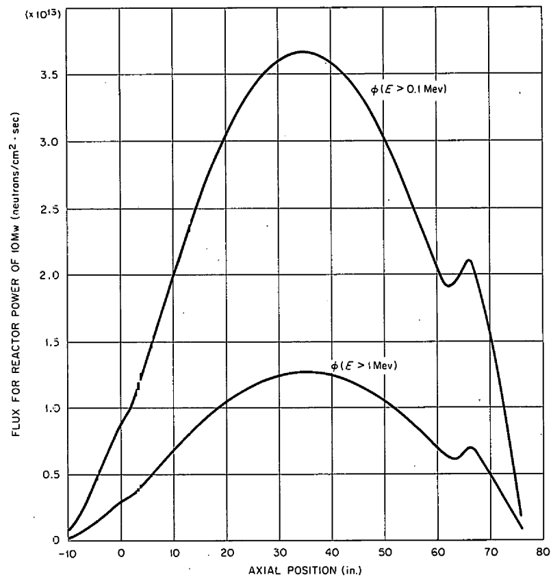
Fig. 2.8. High-Energy Neutron Fluxes 3 in. from Core Center Line Based on Modric Calculations.
