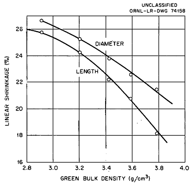
Fig. 4.8. Sintering Shrinkage of Gd_2O_3 Soaked at 1750^\circ C in Hydrogen for 3/4 hr.
