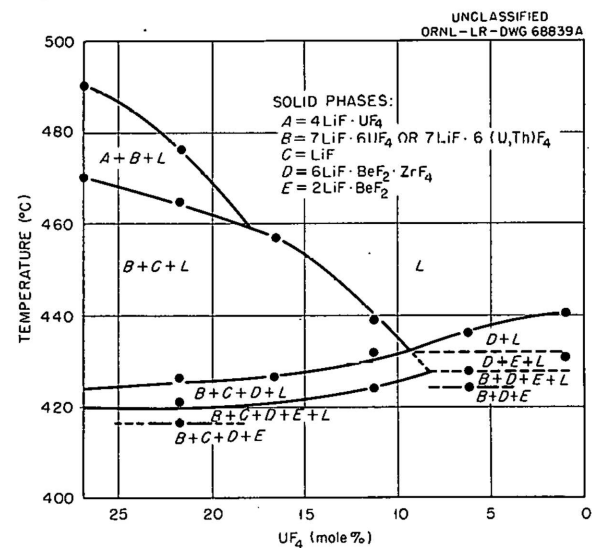
Fig. 6.2. The Section LiF-UF 4 (73-27 mole %) - LiF-BeF 2 -ZrF 4 -ThF 4 -UF 4 (70-23-5-1-1 mole %).
