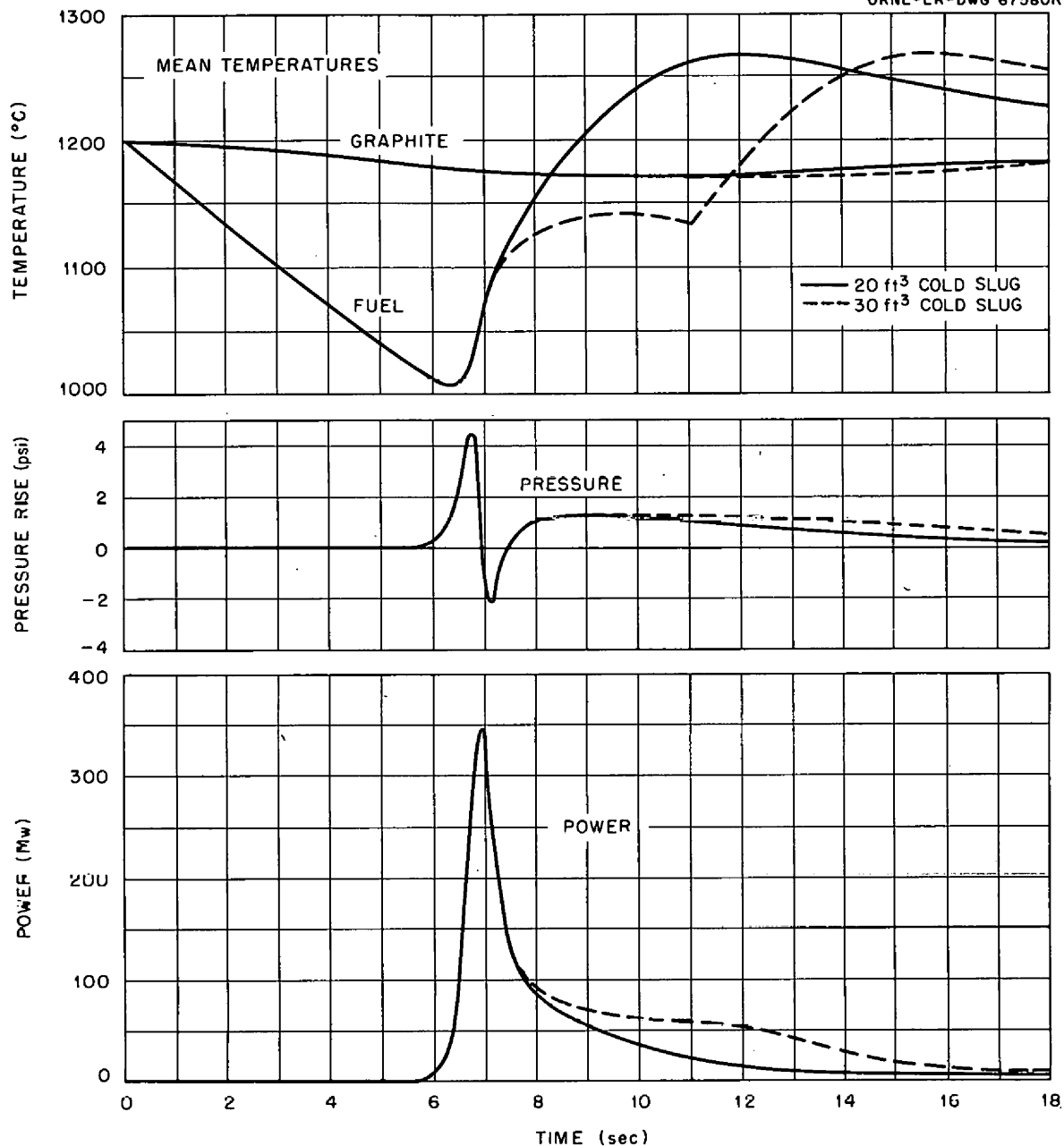
Fig. 2.3. System Behavior Associated with Passage of Cold Slugs at 900°F and a 1200-gpm Flow Rate with the Core Initially at 1200°F.
