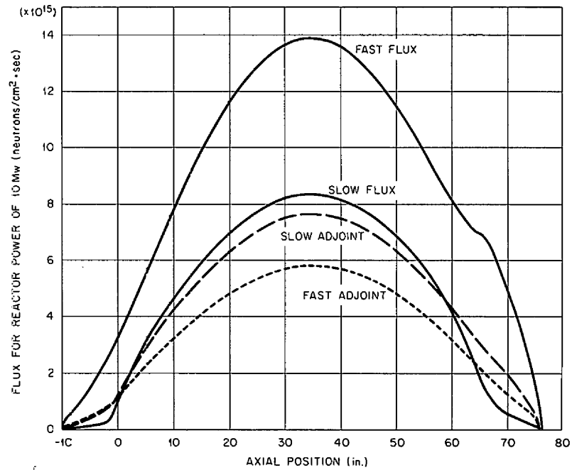
Fig. 2.6. Axial Distribution of Fluxes and Adjoint Fluxes at a Position 7 in. from Core Center Line.
