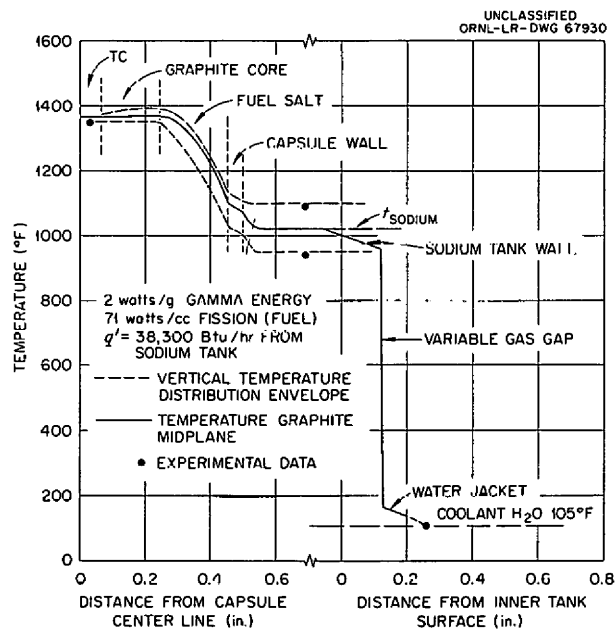
Fig. 5.1. Radial Temperature Distribution of MSRE Capsules.
