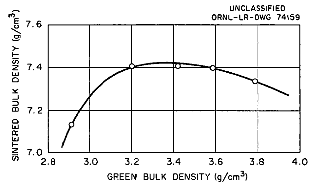
Fig. 4.9. Bulk Density Change of Gd_2O_3 Soaked at 1750^\circ C in Hydrogen for 3/4 hr.
