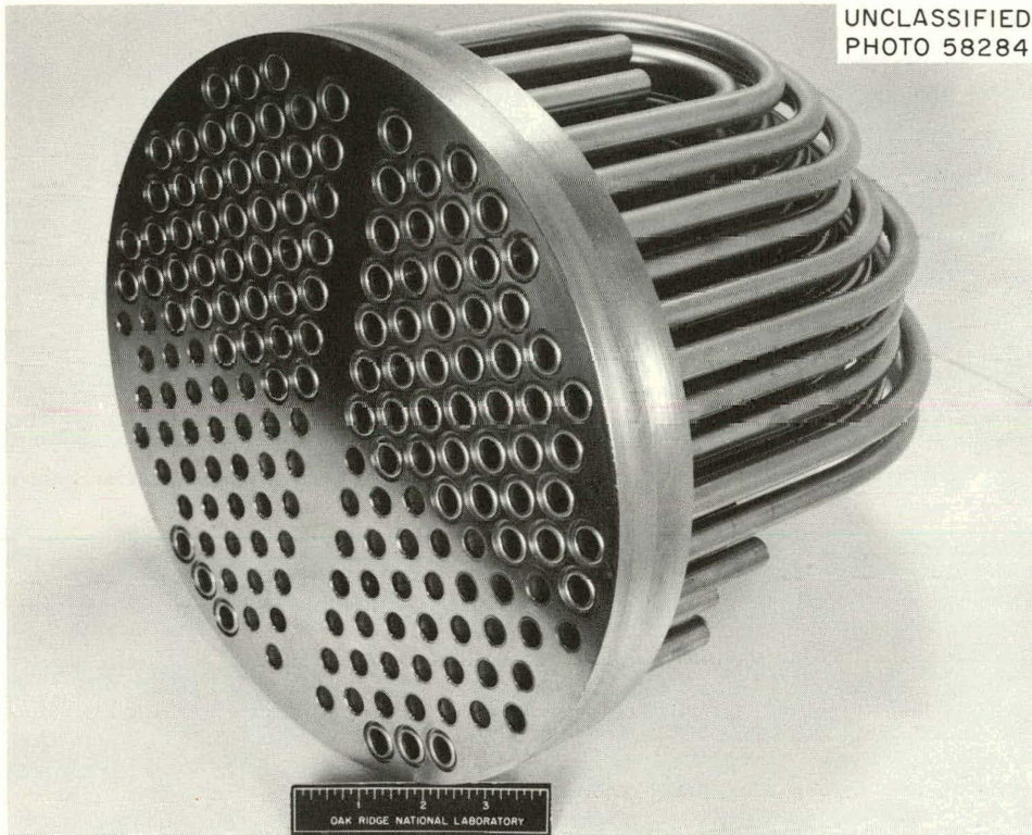
Fig. 4.3. Weld Side of Test Assembly with MSRE Heat Exchanger Type of Joint.
