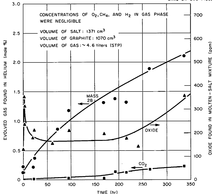
Fig. 6.7. Removal of Adsorbed Gas from AGOT Graphite Immersed in LiF-BeF_2 (66-34 mole %) at 600^\circ C .
