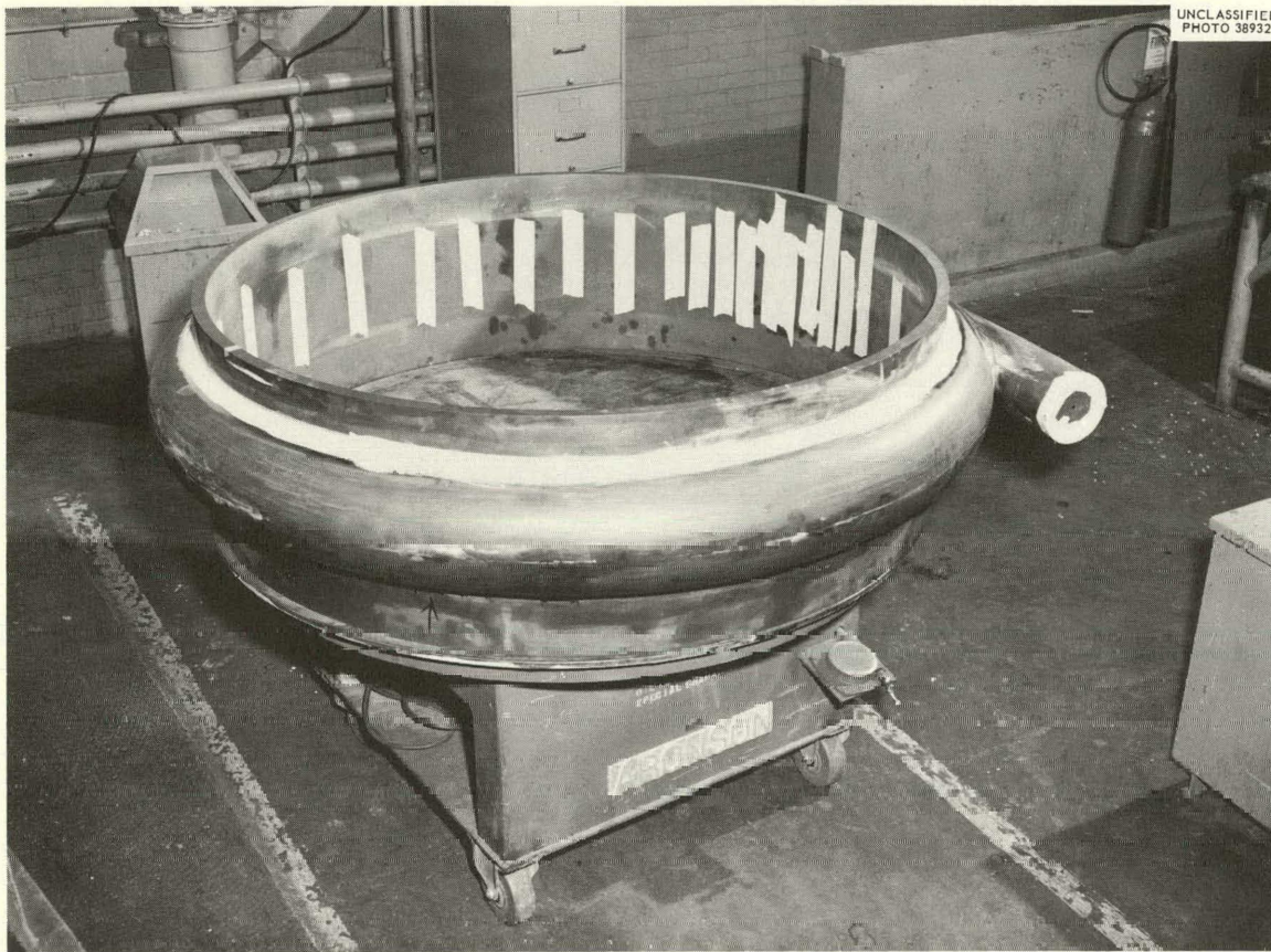
Fig. 1.4. Flow Distribution Nozzle for Reactor Vessel.
