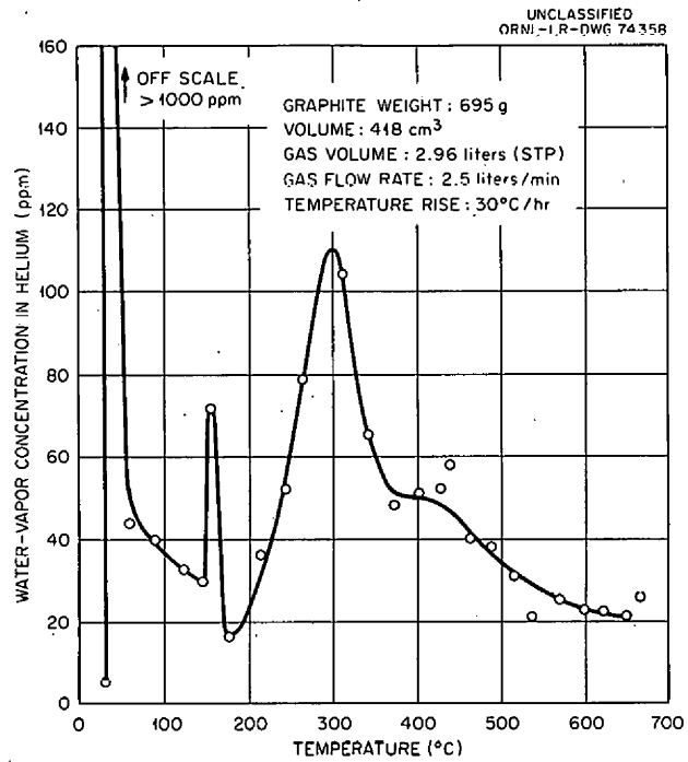
Fig. 6.3. Removal of Moisture from AGOT Graphite by Helium Purgings.
