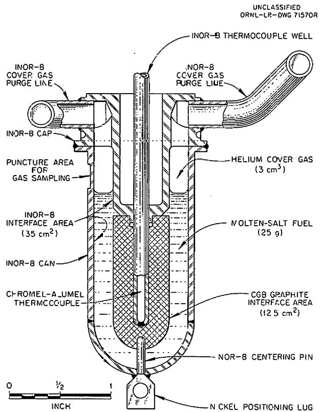
Fig. 5.2. Submerged and Purged Graphite-Molten-Salt Capsule.
