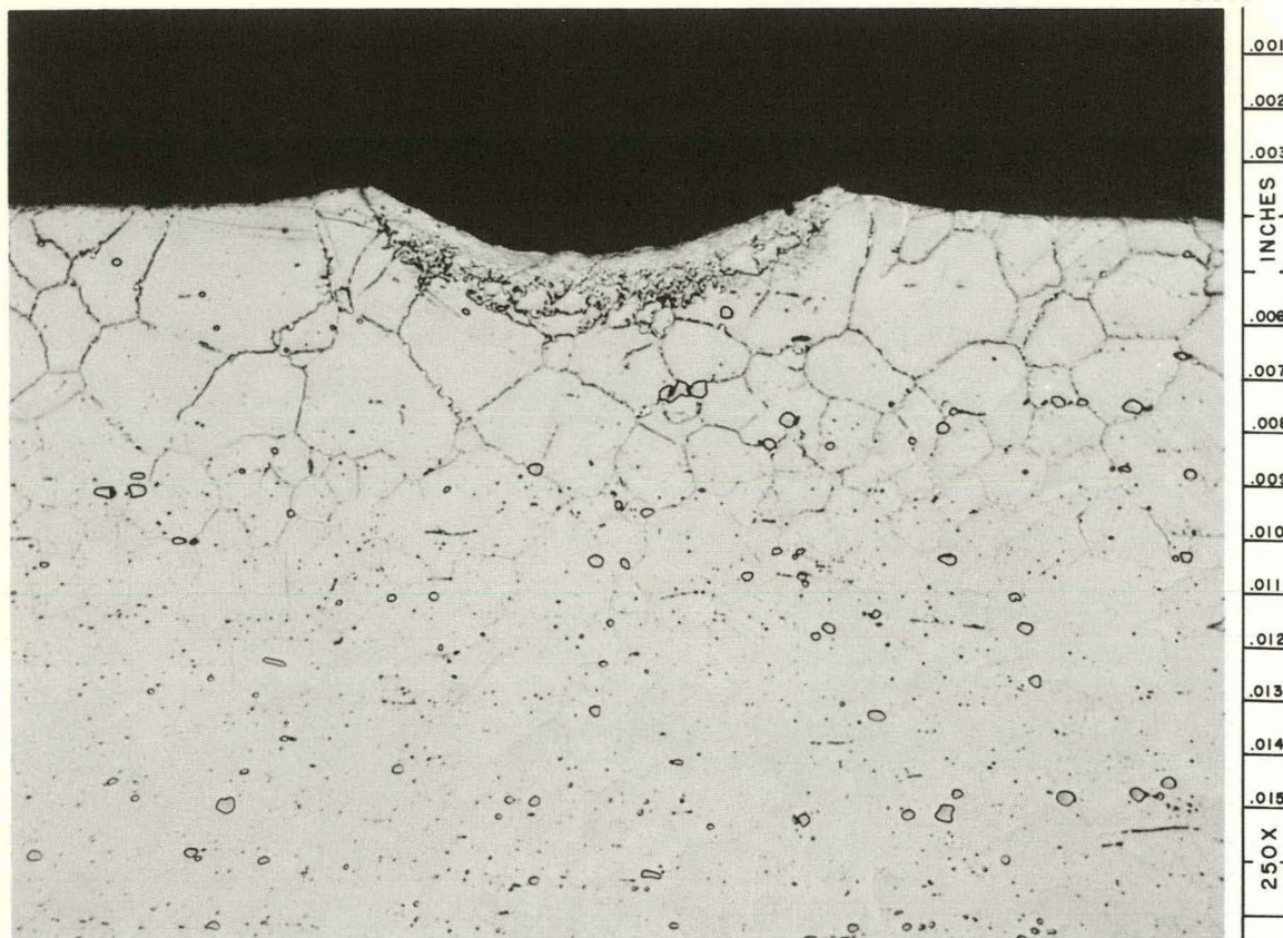
Fig. 4.1. Corrosion Effects of CF_4 on INOR-8 at 1292°F.
