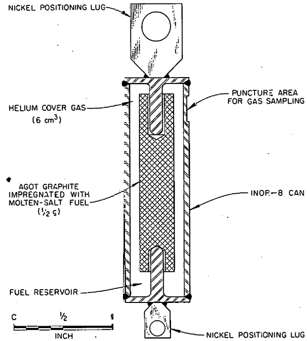
Fig. 5.5. Impregnated-Graphite-Molten-Salt Capsule.
