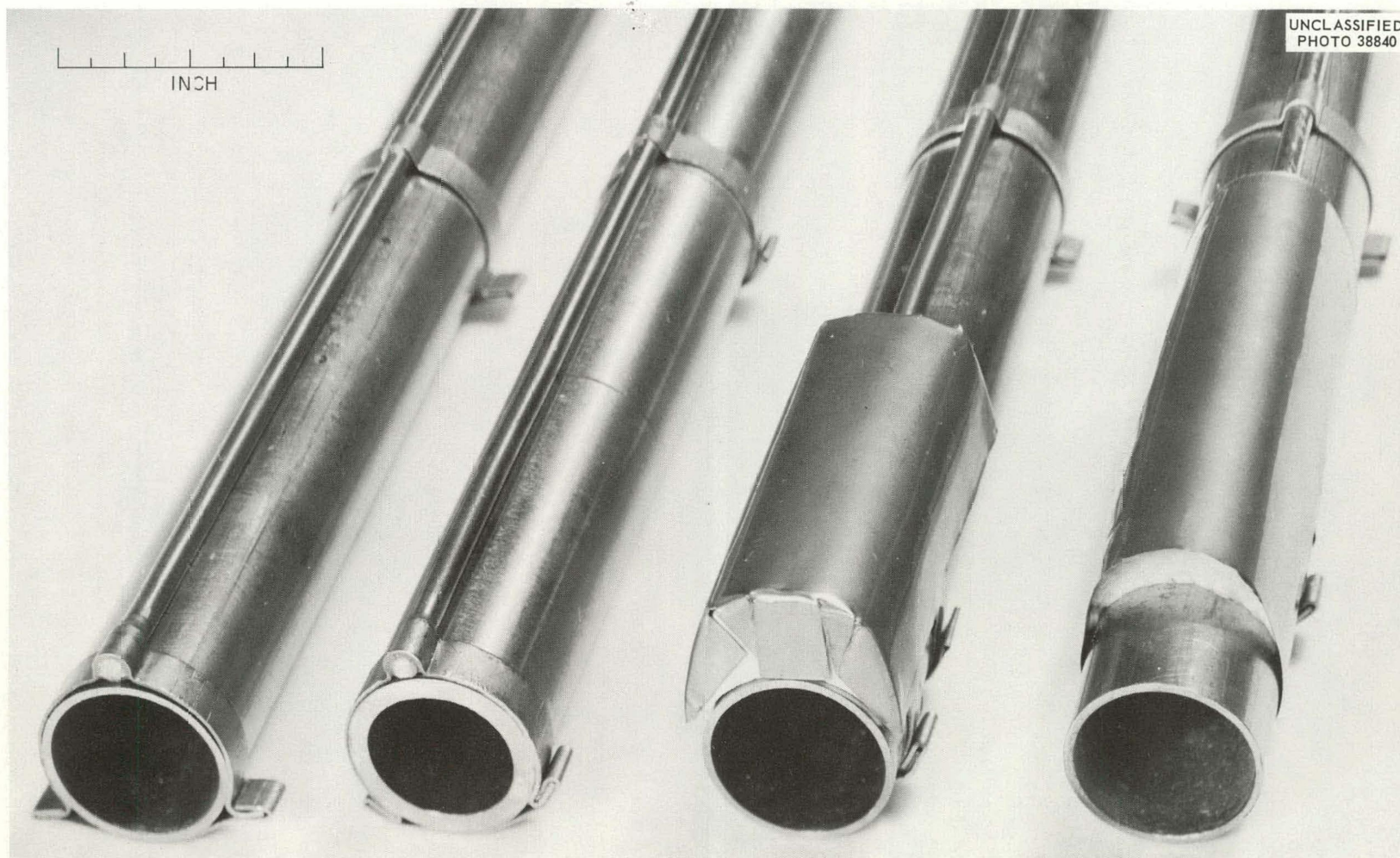
Fig. 3.22. Radiator Tube Thermocouple Attachments.
