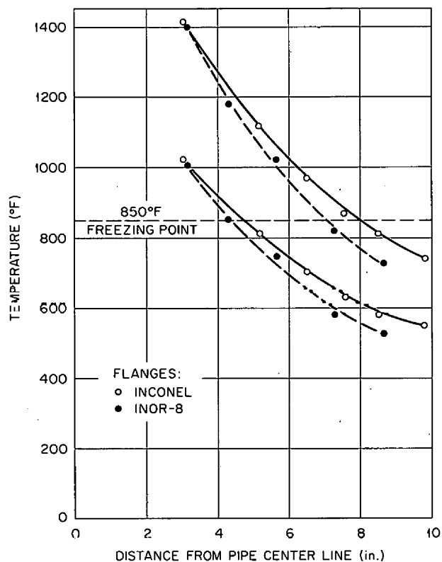
Fig. 3.1. Temperatures of Inconel and INOR-8 Freeze Flanges at Comparable Distances from Center Line of Pipe. Flanges tested in air.
