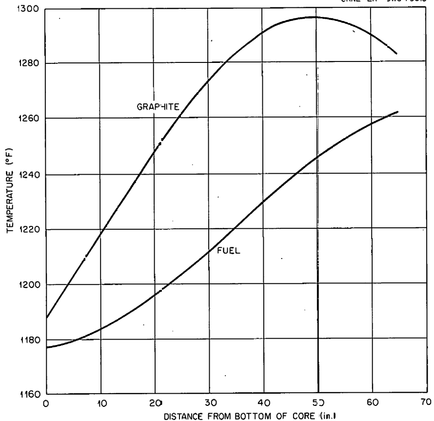
Fig. 2.9. Axial Temperature Profiles in Hottest Channel of MSRE Core (7 in. from Core Center Line).
