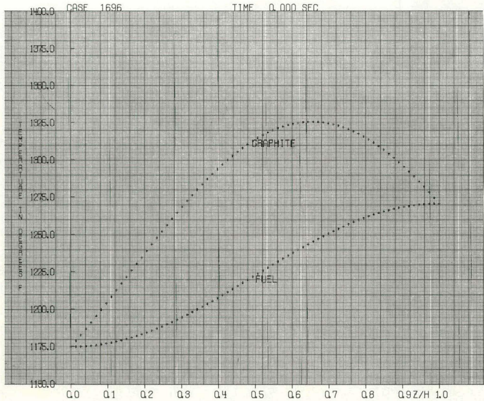
Fig. 2.16. Output of Calcomp Plotter: Fuel and Graphite Temperature Distributions in Hottest Channel with Reactor at 10 Mw.
