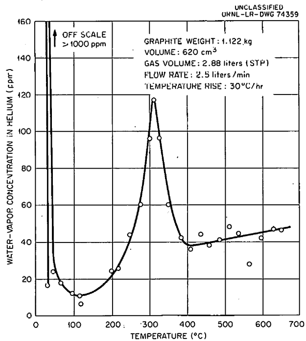
Fig. 6.4. Removal of Moisture from ETL Graphite by Helium Purgings.
