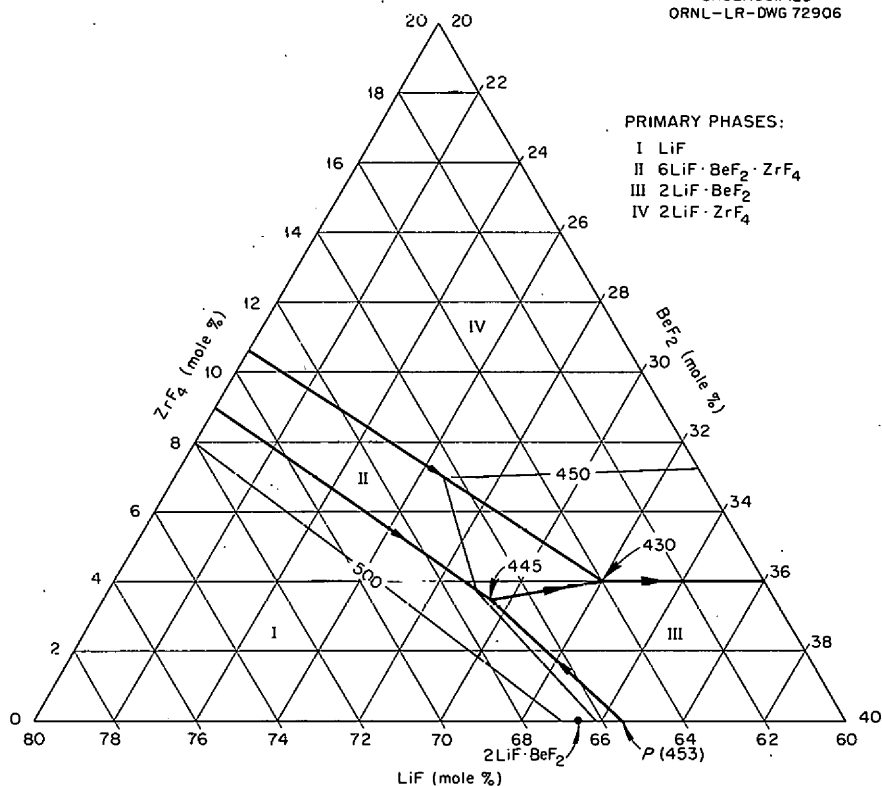
Fig. 6.1. The System LiF-BeF 2 -ZrF 4 .
