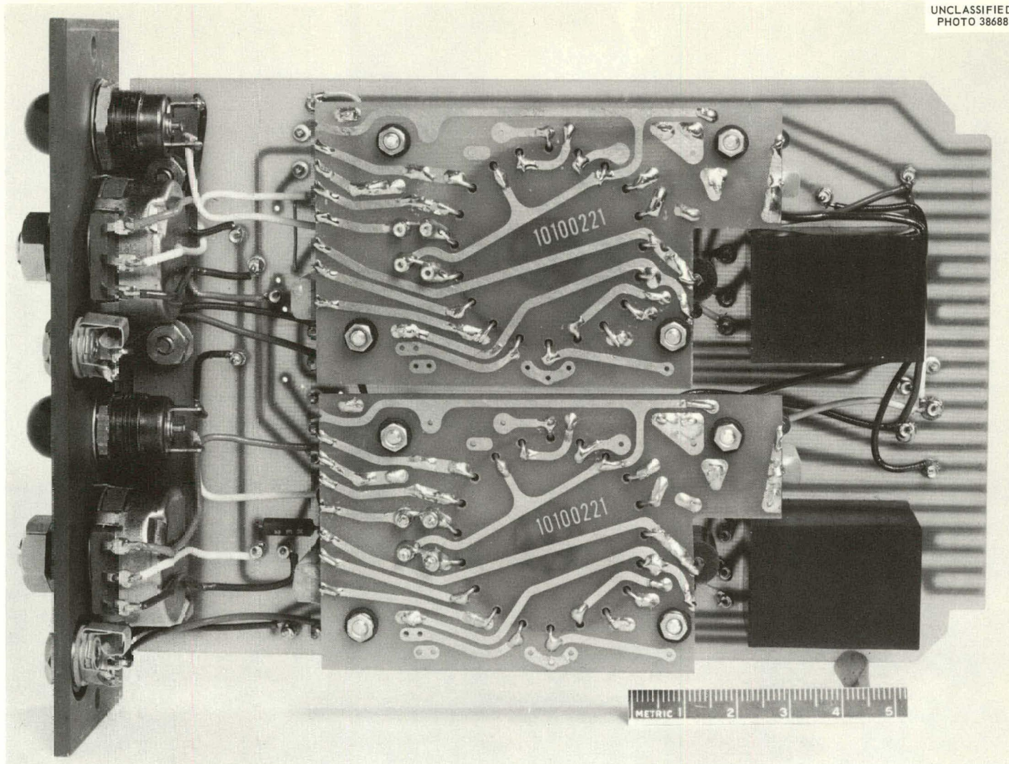
Fig. 3.16. Dual-Limit Alarm Module.
