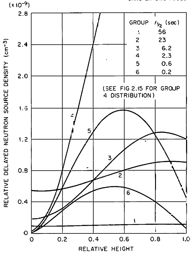
Fig. 2.14. Axial Distribution of Delayed-Neutron Source Densities in an MSRE Fuel Channel. Fuel circulating at 1200 gpm.
