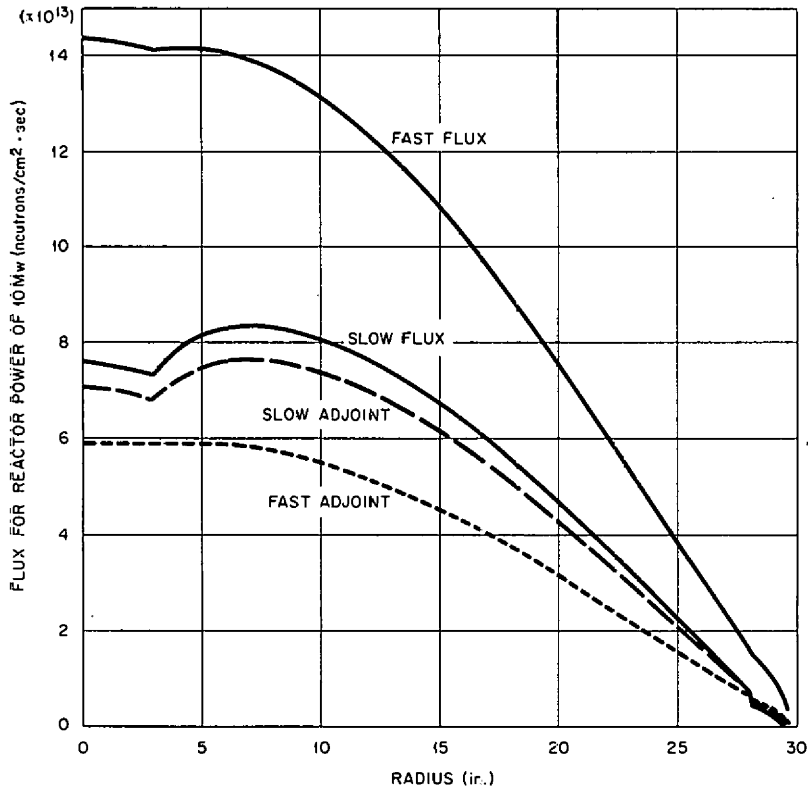
Fig. 2.5. Radial Distribution of Fluxes and Adjoint Fluxes in the Plane of Maximum Slow Flux.
