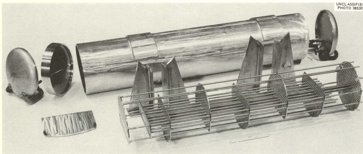
Fig. 1.5. Some Completed Components of INOR-8 Primary Heat Exchanger.
