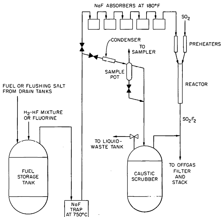
Fig. 7.1. MSRE Fuel-Processing System.
