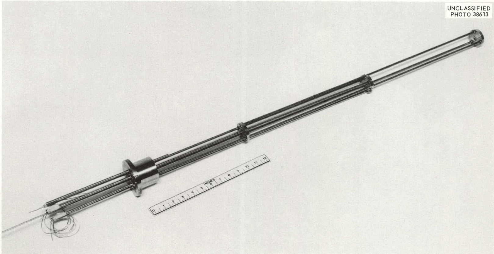
Fig. 3.13. Prototype Model of Two-Level Conductivity Probe.
