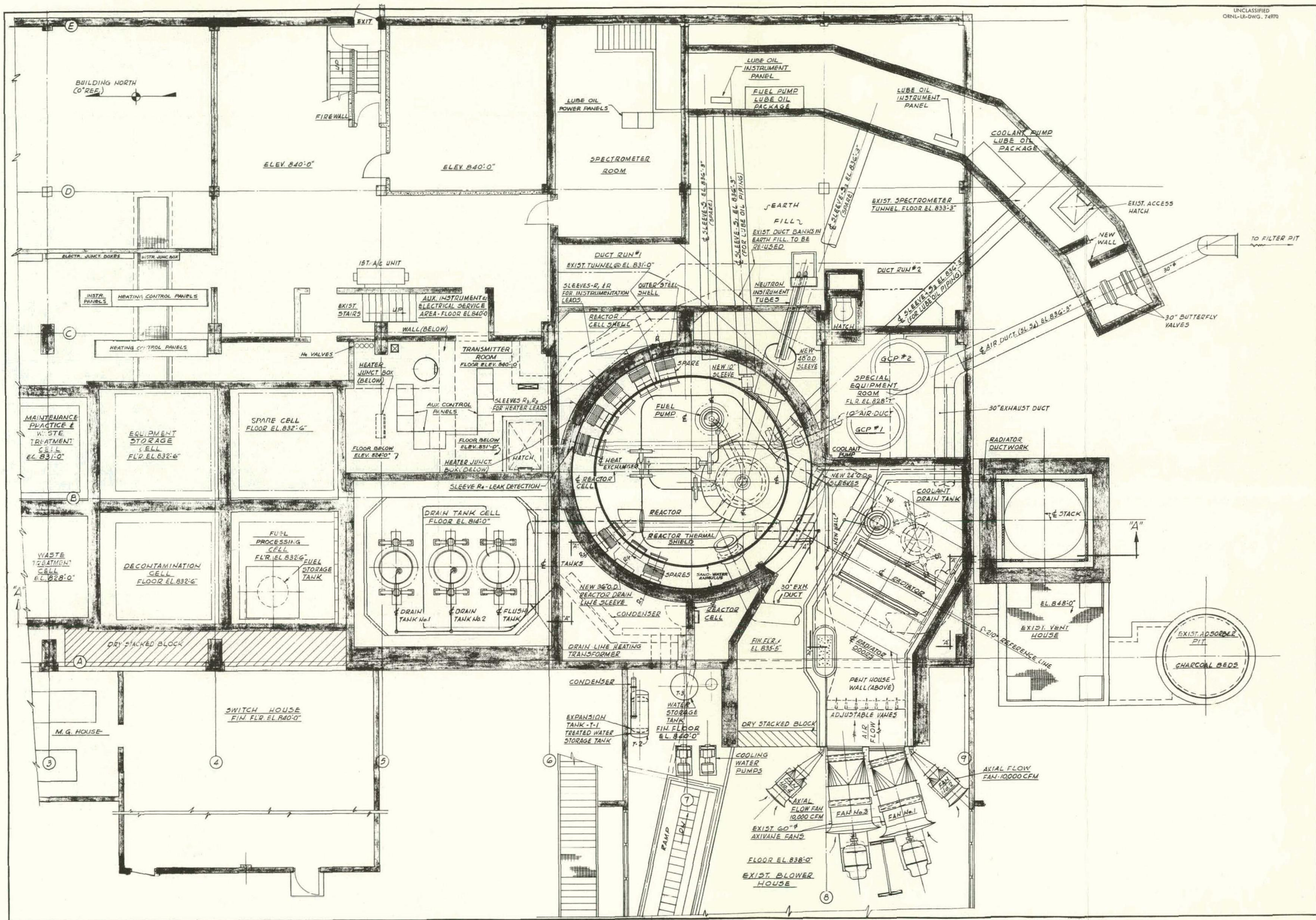
Fig. 1.1. Plan View of MSRE.
