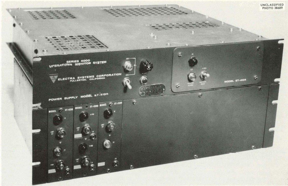
Fig. 3.17. Temperature-Monitoring System Assembly.
