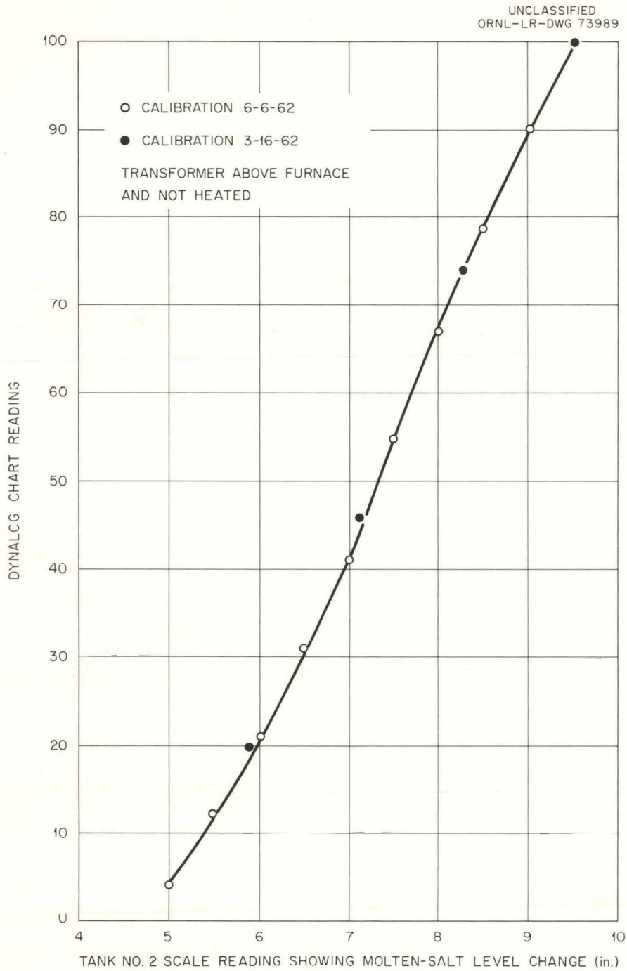
Fig. 3.15. Calibration Curve of Recorder of Pump-Dowl Liquid-Level Indicator No. 2 Before and After Three Months Operation at 1200°F.
