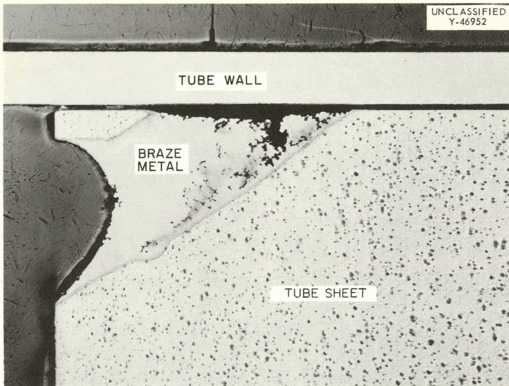
Fig. 4.5. Defective Braze Caused by Metal Chips in Feeder Holes.
