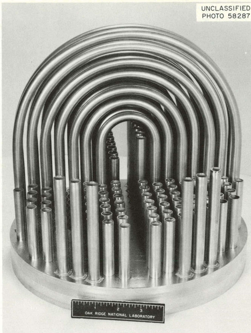
Fig. 4.4. Braze Side of Test Assembly with MSRE Heat Exchanger Type of Joint.
