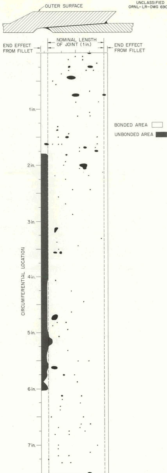
Fig. 4.6. Results of Ultrasonic Inspection of a Remotely Brazed Pipe Joint.
