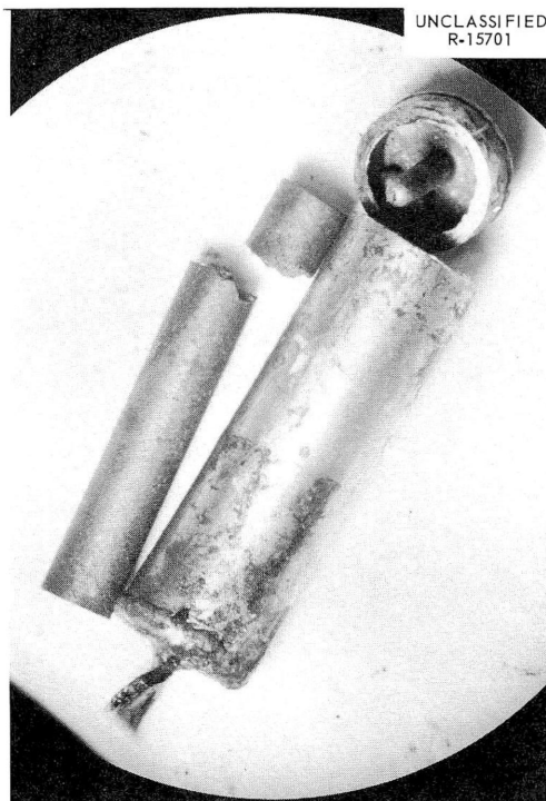
Fig. 5.17. Capsule R with Graphite Removed. Break Occurred During Segmenting.
