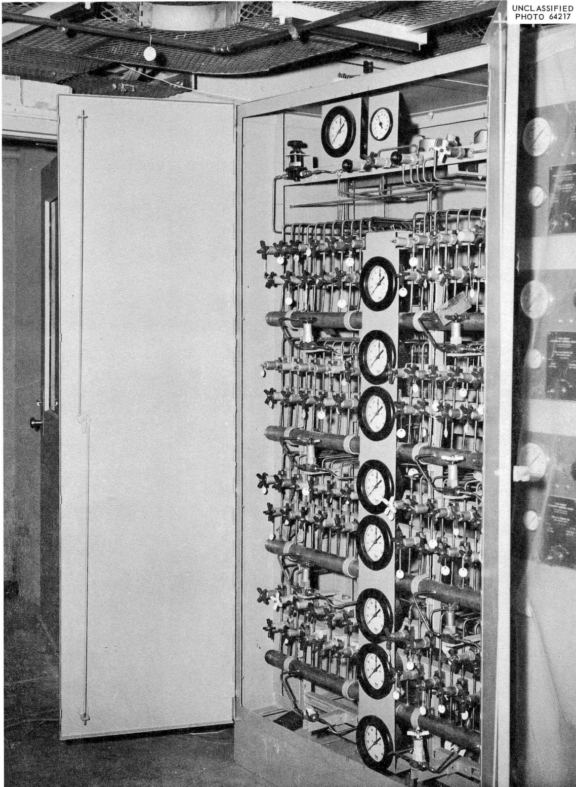
Fig. 1.7. Leak-Detector Panels.
