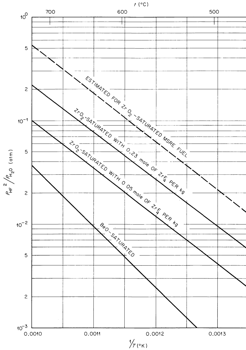
Fig. 6.16. Observed Values of \frac{P_{HF}^2}{P_{H_2O}} in Equilibrium with 2LiF-BeF_2 Melts Saturated with BeO or ZrO_2 .
