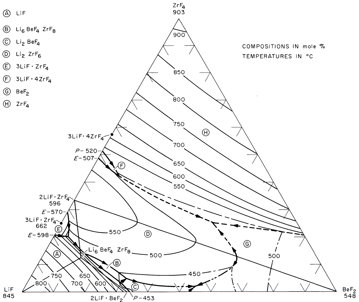
Fig. 6.1. The System LiF-BeF 2 -ZrF 4 .
