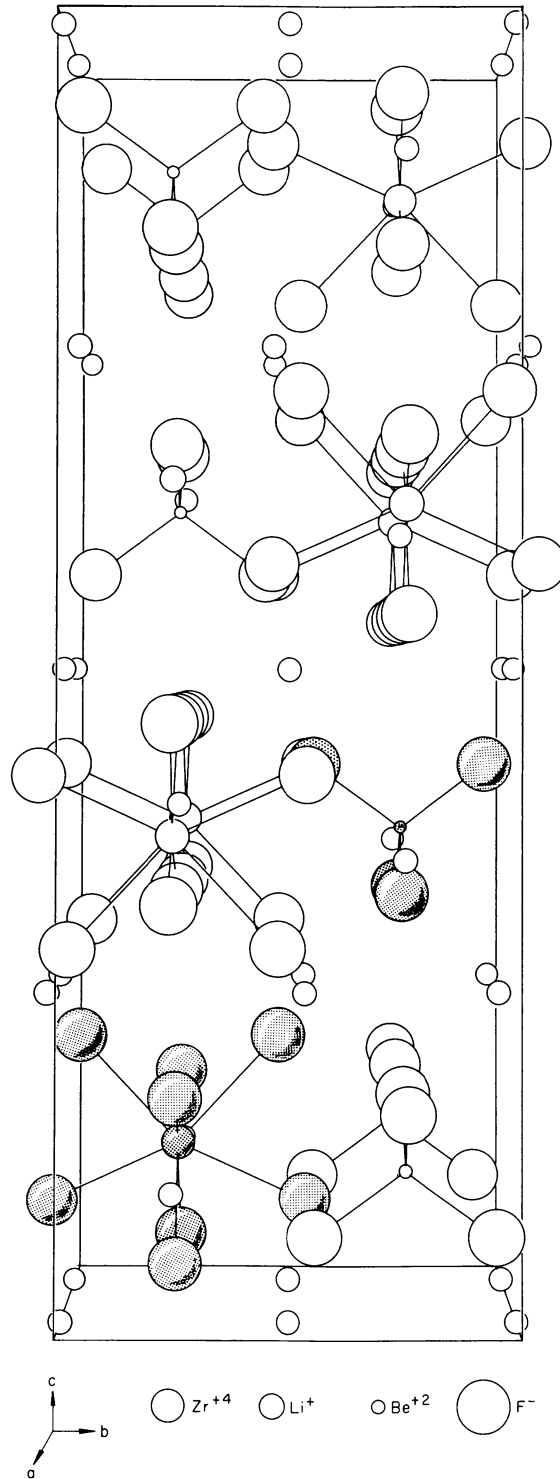
Fig. 6.4. Perspective Drawing of the Structure of Li_6BeF_4ZrF_8 .
