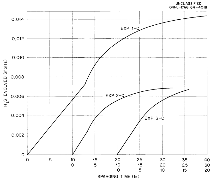
Fig. 6.17. Removal of Sulfur from 2\text{LiF}\text{-BeF}_2 by HF- \text{H}_2 Sparging After Reduction by Beryllium Metal. The conditions of these tests are listed in Table 6.7.
