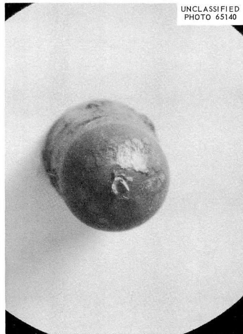
Fig. 5.13. Scale on Bottom of Graphite Core from Capsule 3. Projection from Center is Part of the Metal Supporting Pin.
