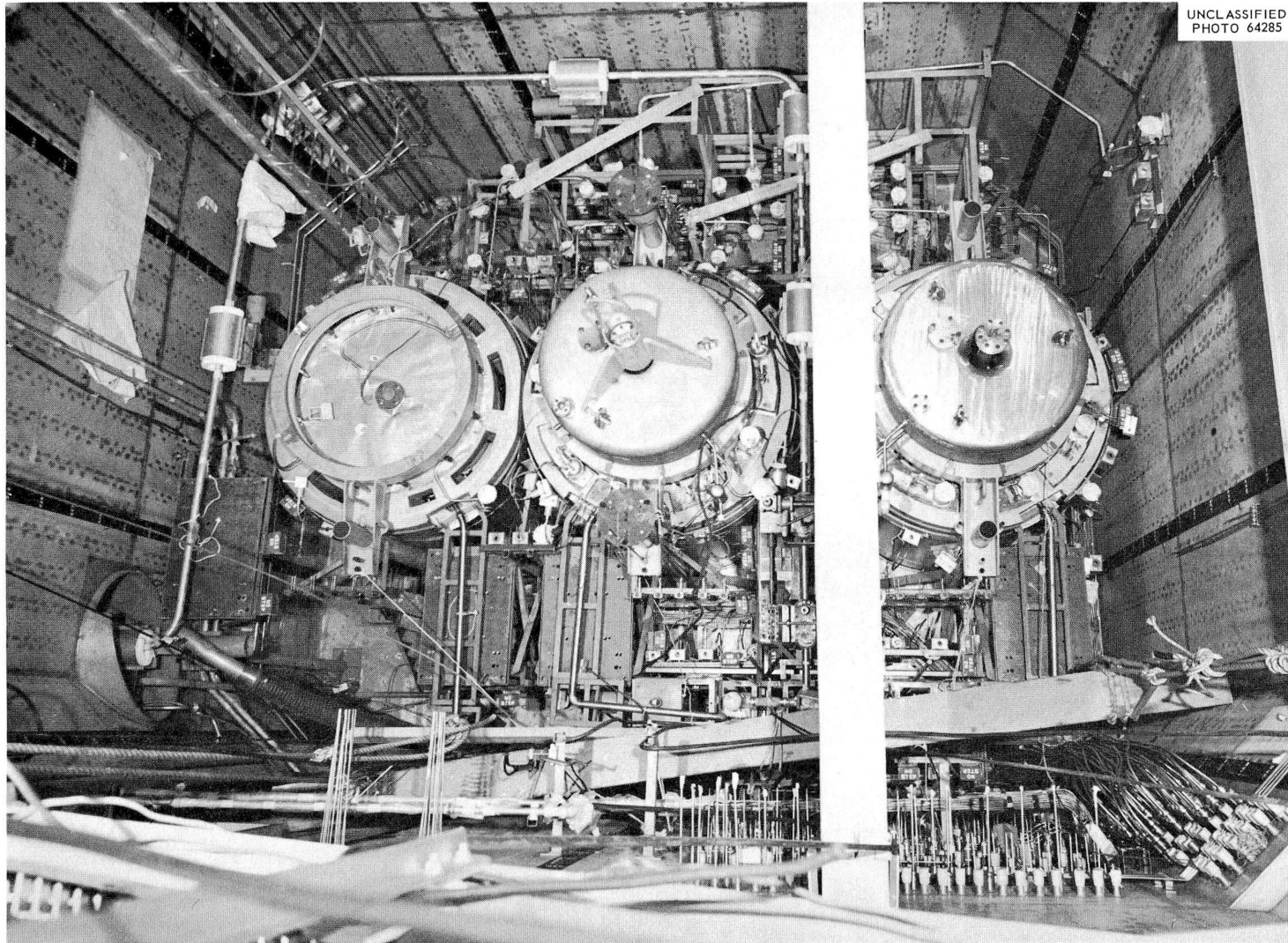
Fig. 1.6. Drain Tank Cell Installation.
