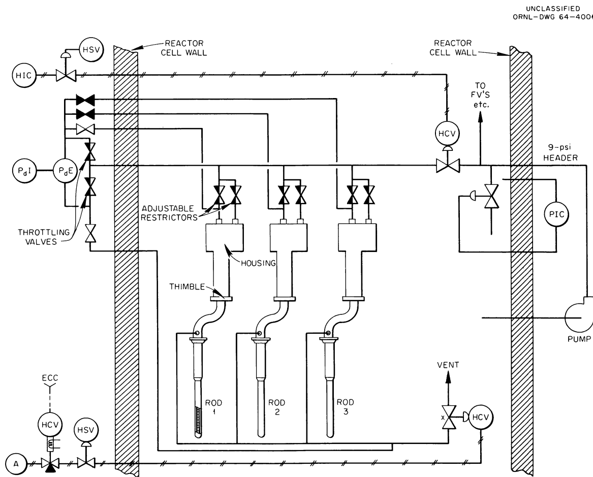
Fig. 2.13. Positive-Position Indicator System for MSRE Control Rod.
