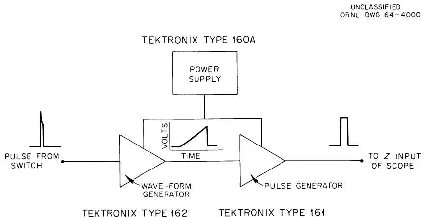
Fig. 2.12. Marker Generator for Temperature Scanner.
