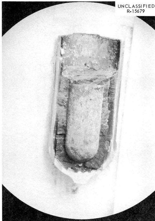
Fig. 5.14. Capsule 4, Showing Graphite Bearing Shiny Film.
