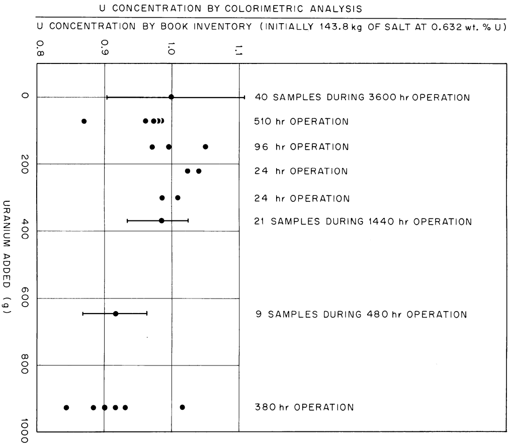
Fig. 2.6. Ratio of Uranium Concentration from Chemical Analysis to Uranium Concentration as Calculated from Uranium Additions.
