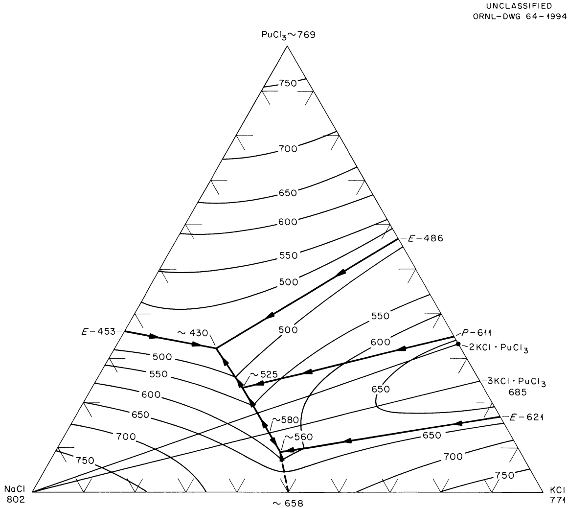
Fig. 6.5. Predicted Phase Behavior for the System NaCl-KCl-PuCl 3 .
