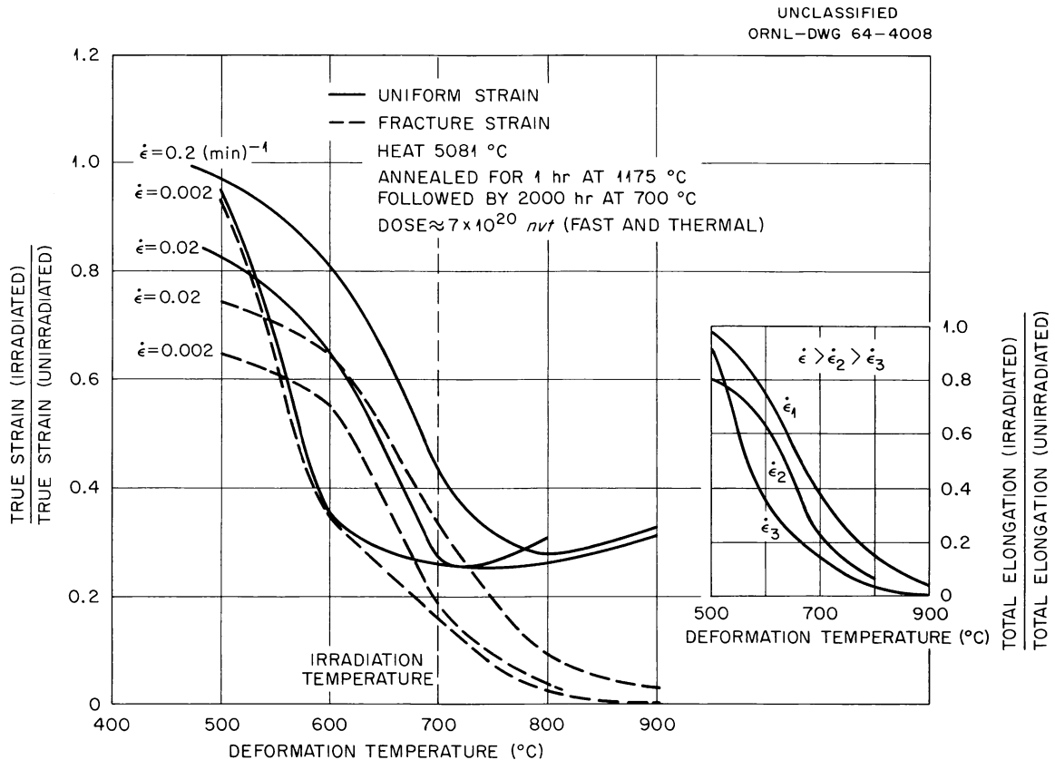
Fig. 4.4. Effect of Irradiation on the Ductility of INOR-8 at Elevated Temperatures.
