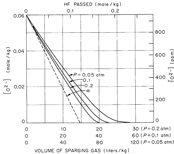
Fig. 6.15. Predicted Efficiency of HF Sparging for Removal of Dissolved Oxide from 2\text{LiF}\cdot\text{BeF}_2 at 600^\circ\text{C} . P is the initial partial pressure of HF. The dashed line represents 100% concentration of HF to produce \text{H}_2\text{O} .
