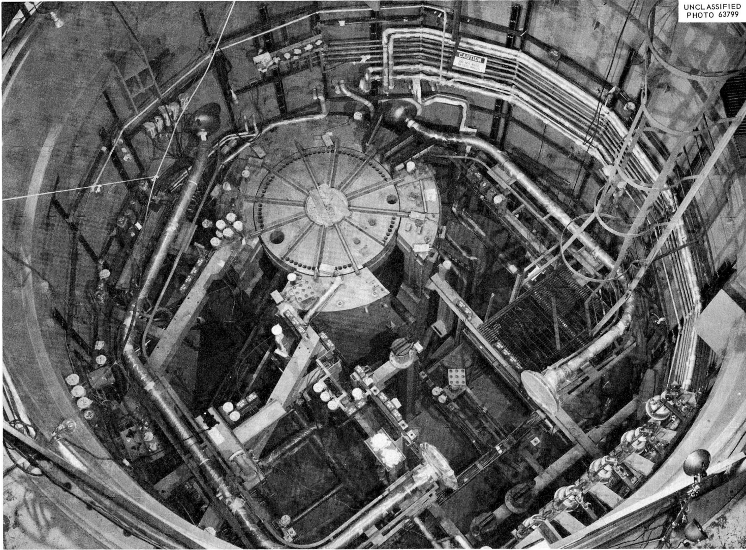
Fig. 1.5. Reactor Cell Installation.
