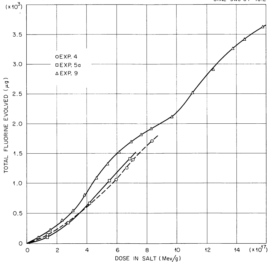
Fig. 5.22. Total Fluorine Evolved During Electron Irradiations.
