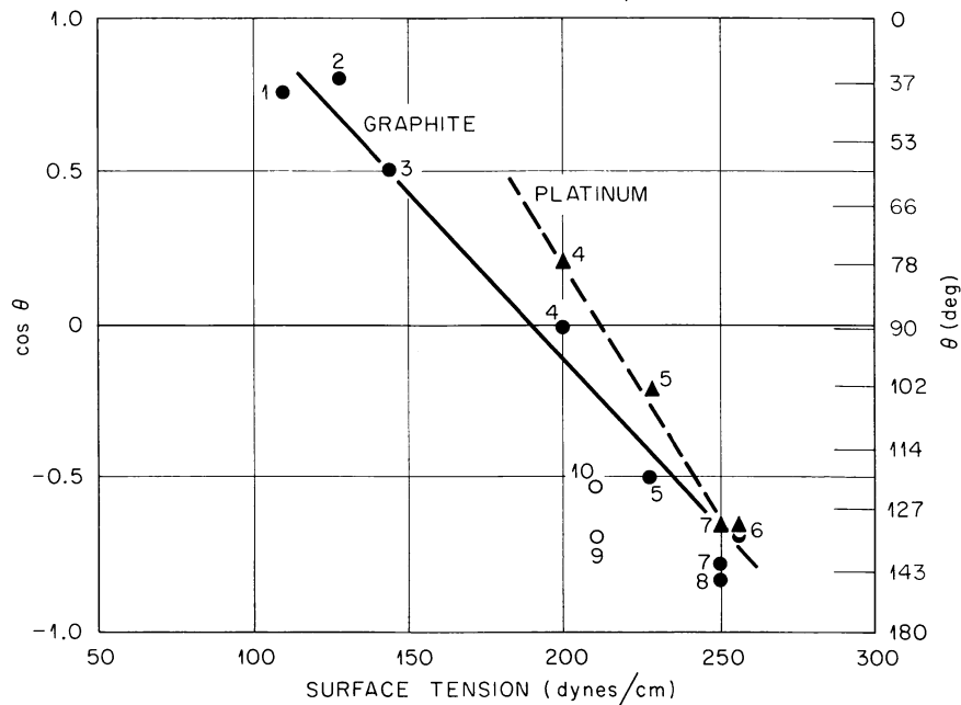
Fig. 6.12. Contact Angle Between Molten Fluorides, Graphite, and Platinum vs Surface Tension at the Melting Point of the Salt.
