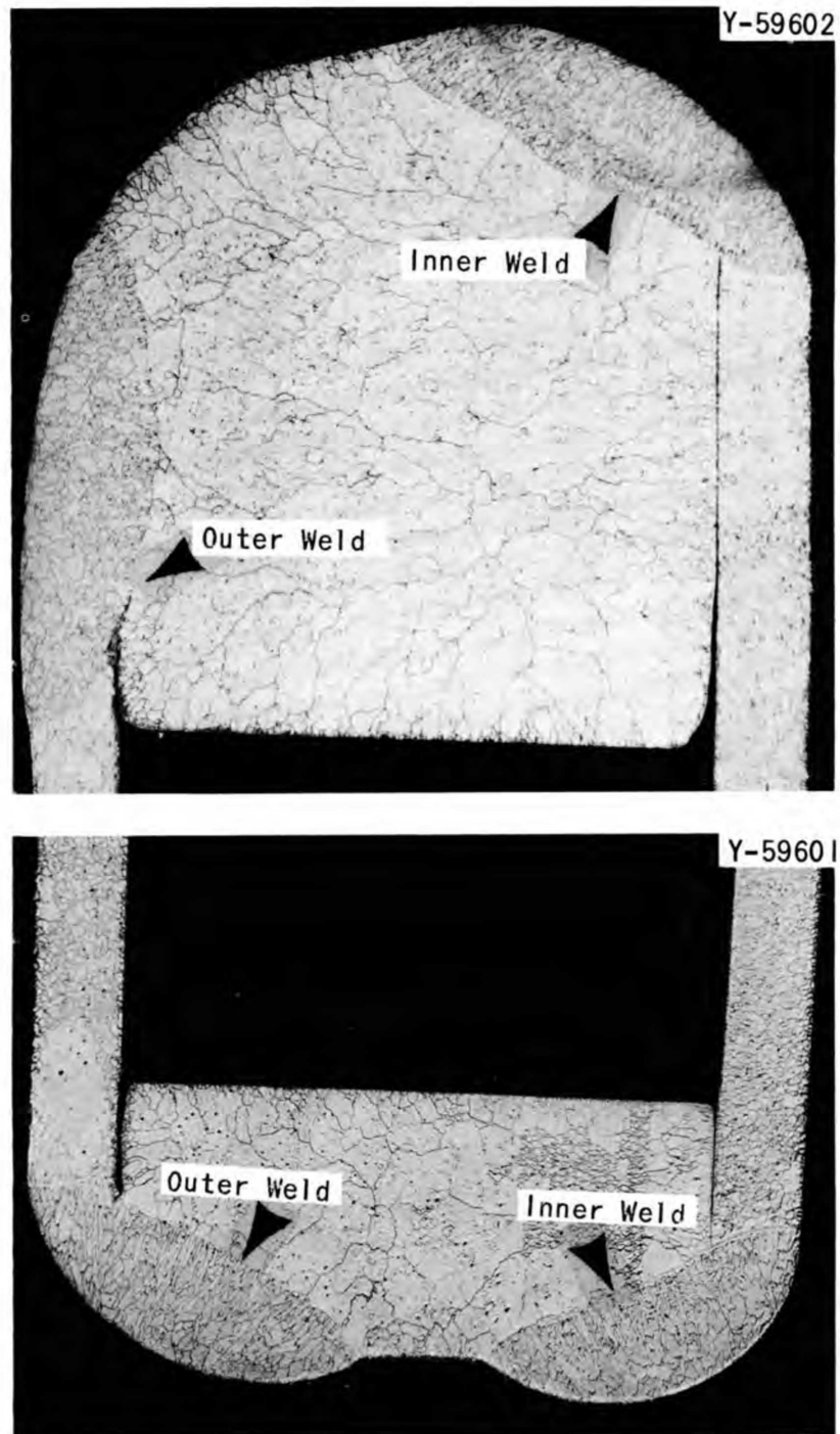
Fig. 2. Sections Through Closure Welds on MSRE Control Elements. (a) Top closure. (b) Bottom closure.
