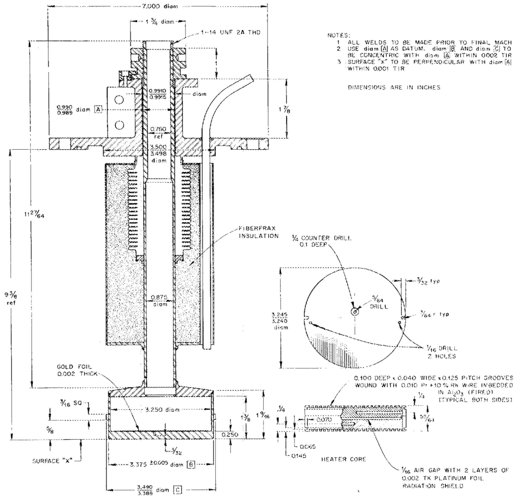
Fig. A-2. Detail of movable piston assembly of the conductivity cell.
