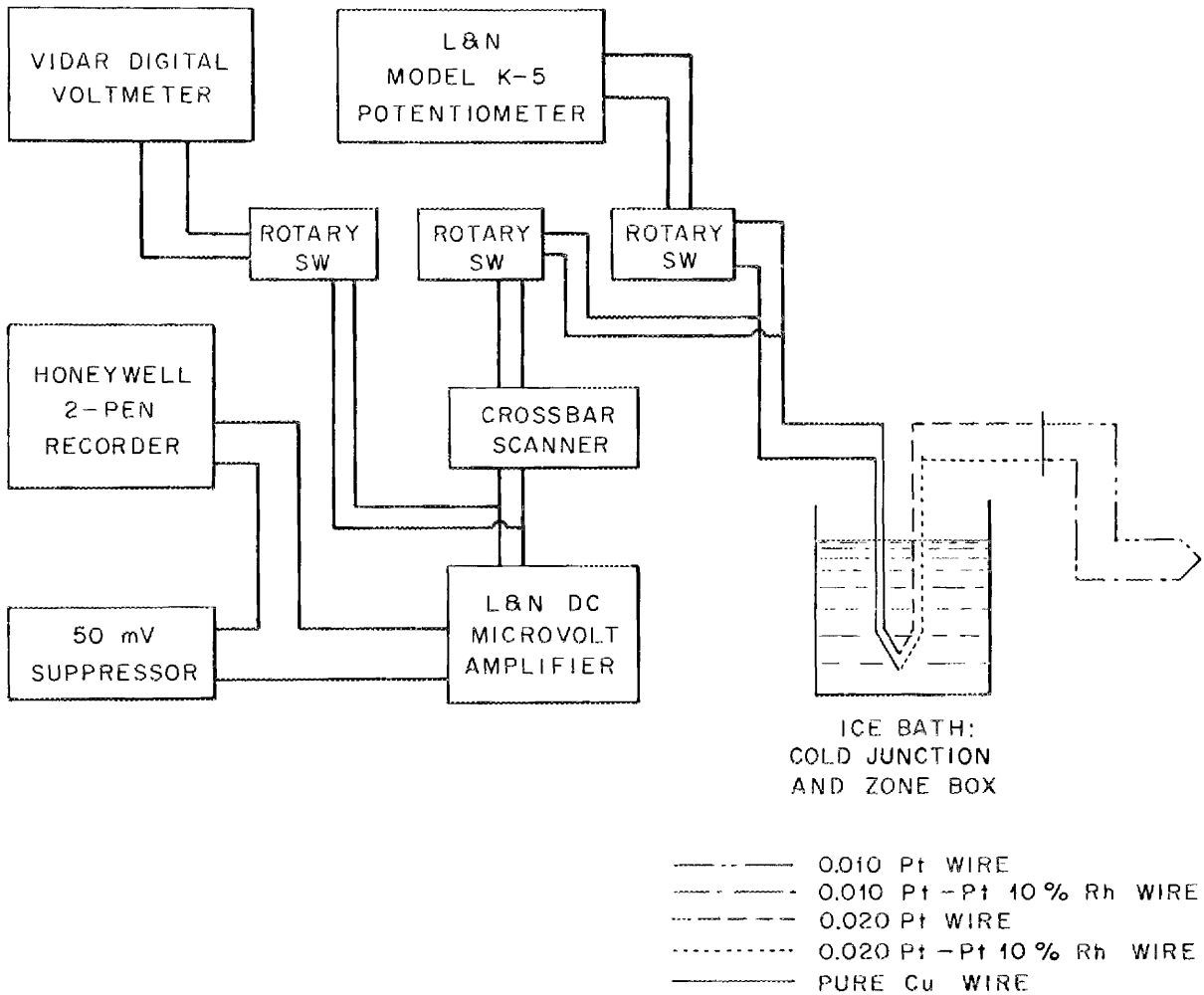
Fig. 15. Thermocouple circuit diagram.
