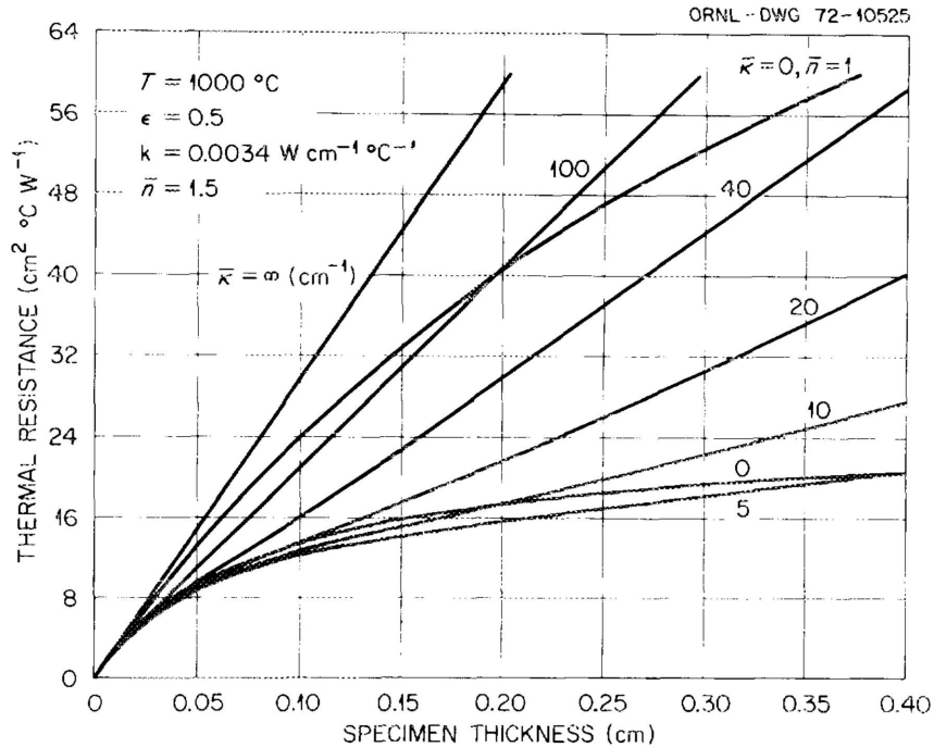
Fig. 3. Thermal resistance of an infrared absorbing fluid having assumed properties at various values of absorptivity, \bar{\kappa} (cm -1 ) vs specimen thickness.
