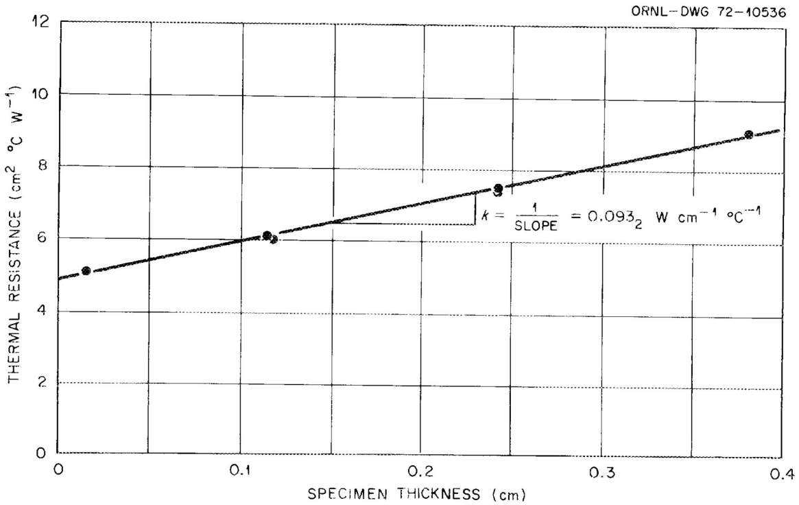
Fig. 16. Total thermal resistance vs specimen thickness of mercury at 60.8°C (Run 2, Apparatus I-A).
