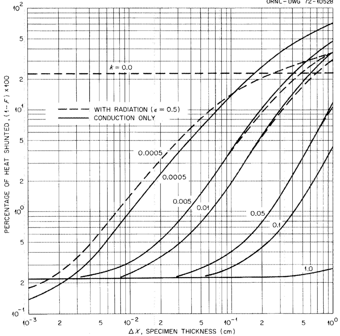
Fig. 6. Percent of heat shunted around specimen vs specimen thickness for various specimen conductivities with and without radiative heat transfer at 300^{\circ}\text{C} for G = 0.5 .
