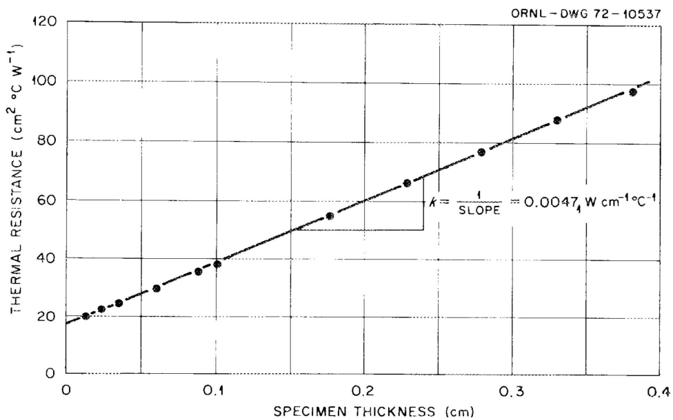
Fig. 17. Total thermal resistance vs specimen thickness of HTS at 197°C (Run 10, Apparatus I-A).
