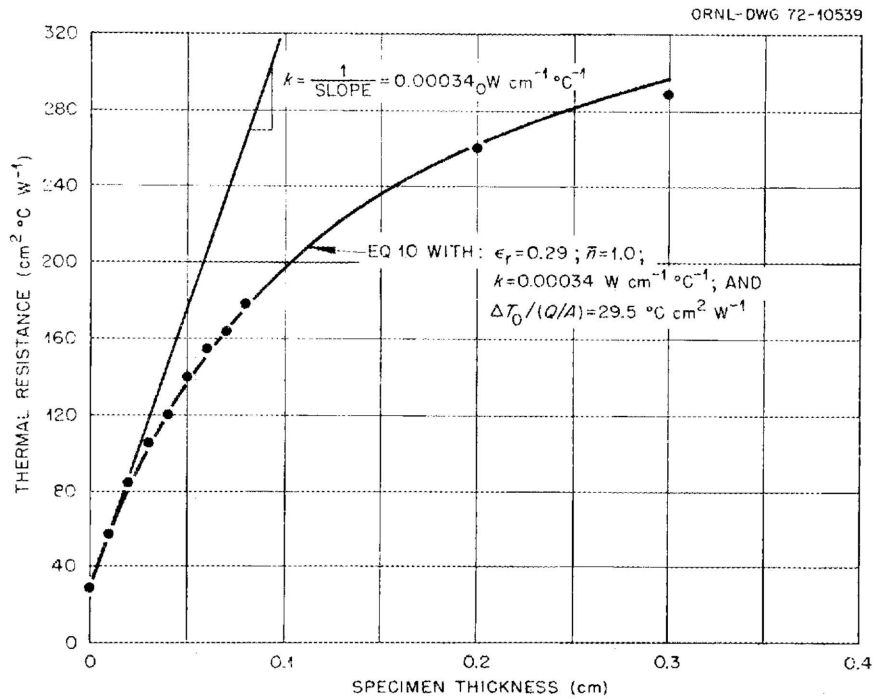
Fig. 19. Total thermal resistance vs specimen thickness of argon at 503^\circ\text{C} (Run 1, Apparatus II-B).
