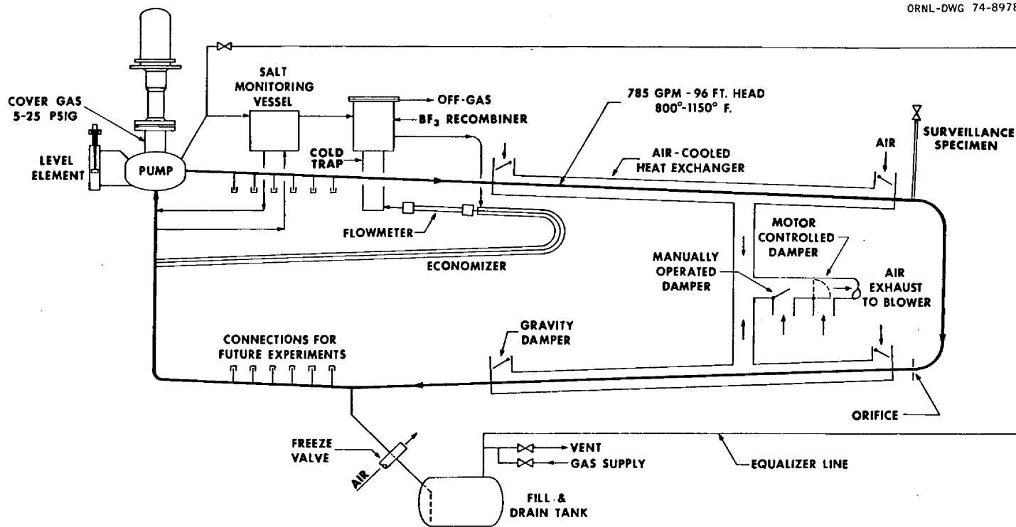
Fig. 10.5.4. CSTF schematic.
