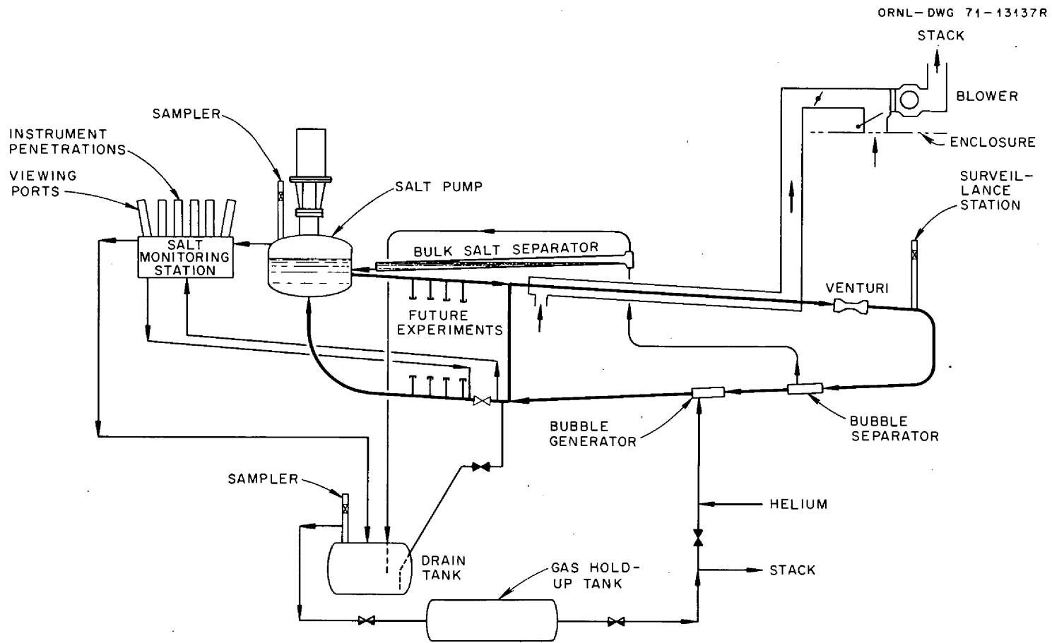
Fig. 10.4.4. GSTF schematic.
