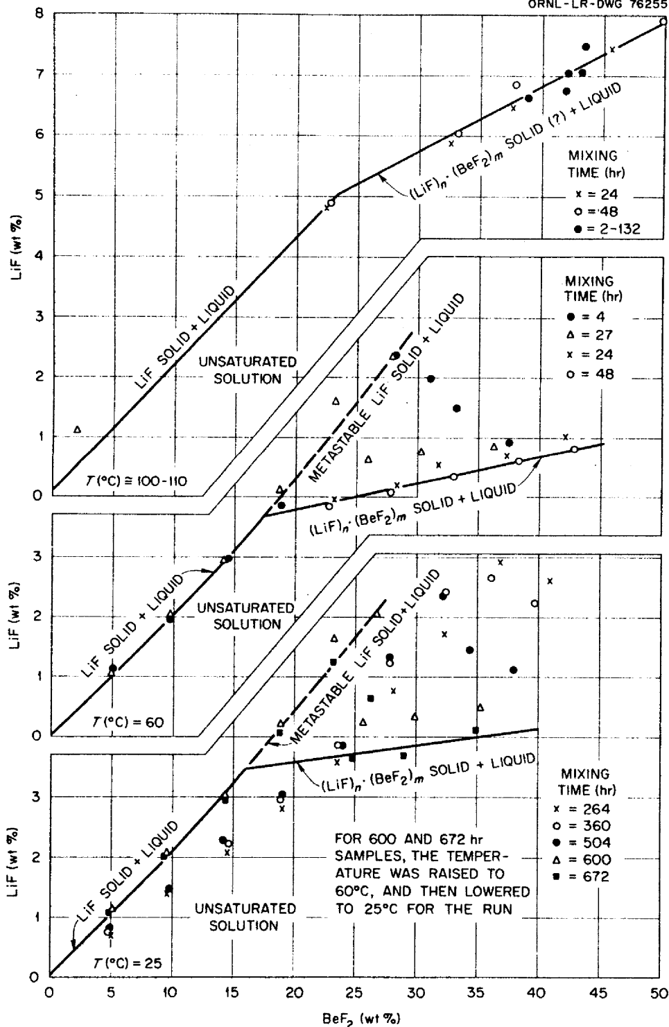
Fig. 5. Some Solubility Behavior in the System LiF-BeF 2 -H 2 O, 25,100°C.
