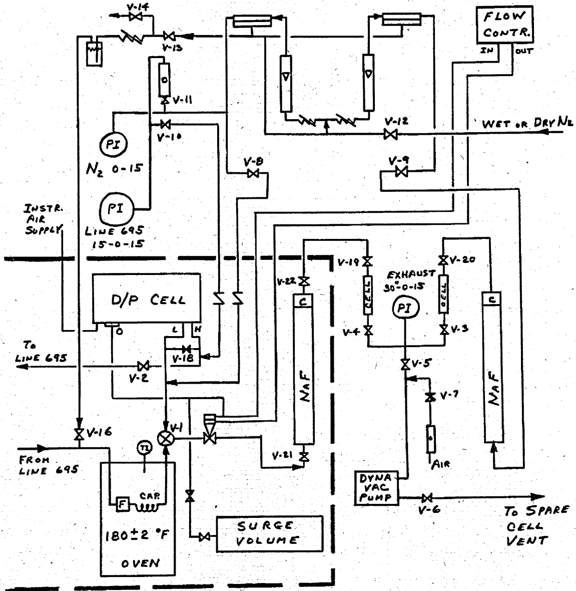
Figure 2.3. Water Analyzer.
