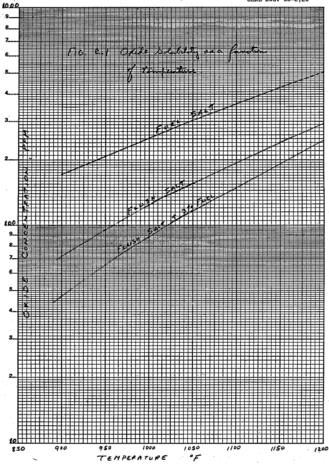
Figure 2.1. Oxide Solubility as a Function of Temperature.
