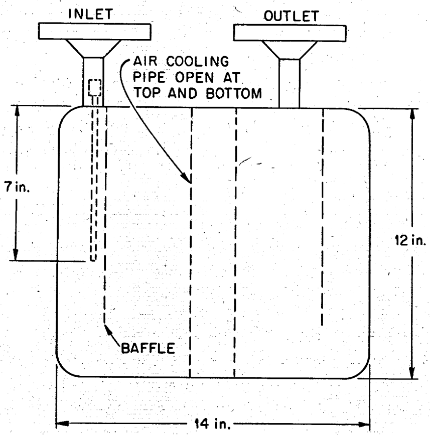
Figure 3.9. NaF Absorbers.
