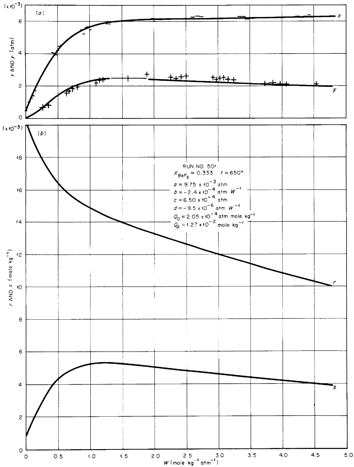
Fig. 11. (a) Dependence of x and y on W , and (b) Variation of r and s with W . Run No. 501.
