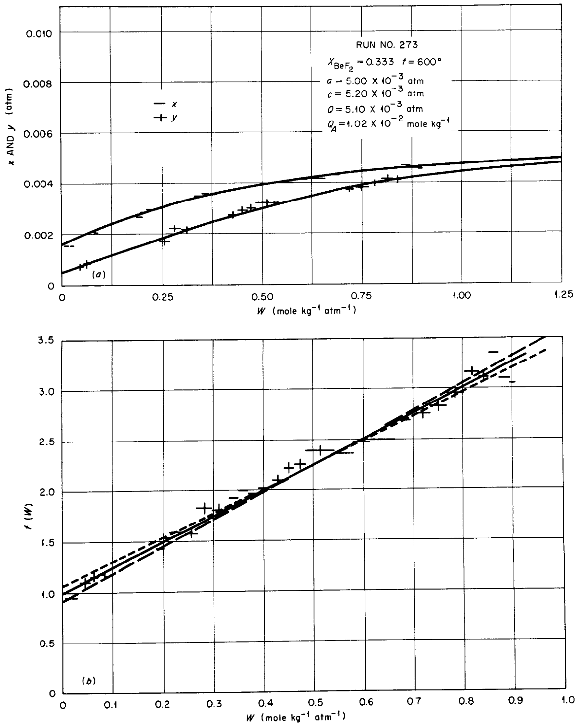
Fig. 3. BeO-saturated 0.333 BeF 2 Showing (a) Calculated and Observed Partial Pressures, and (b) Linear Correlation of Pressures.
