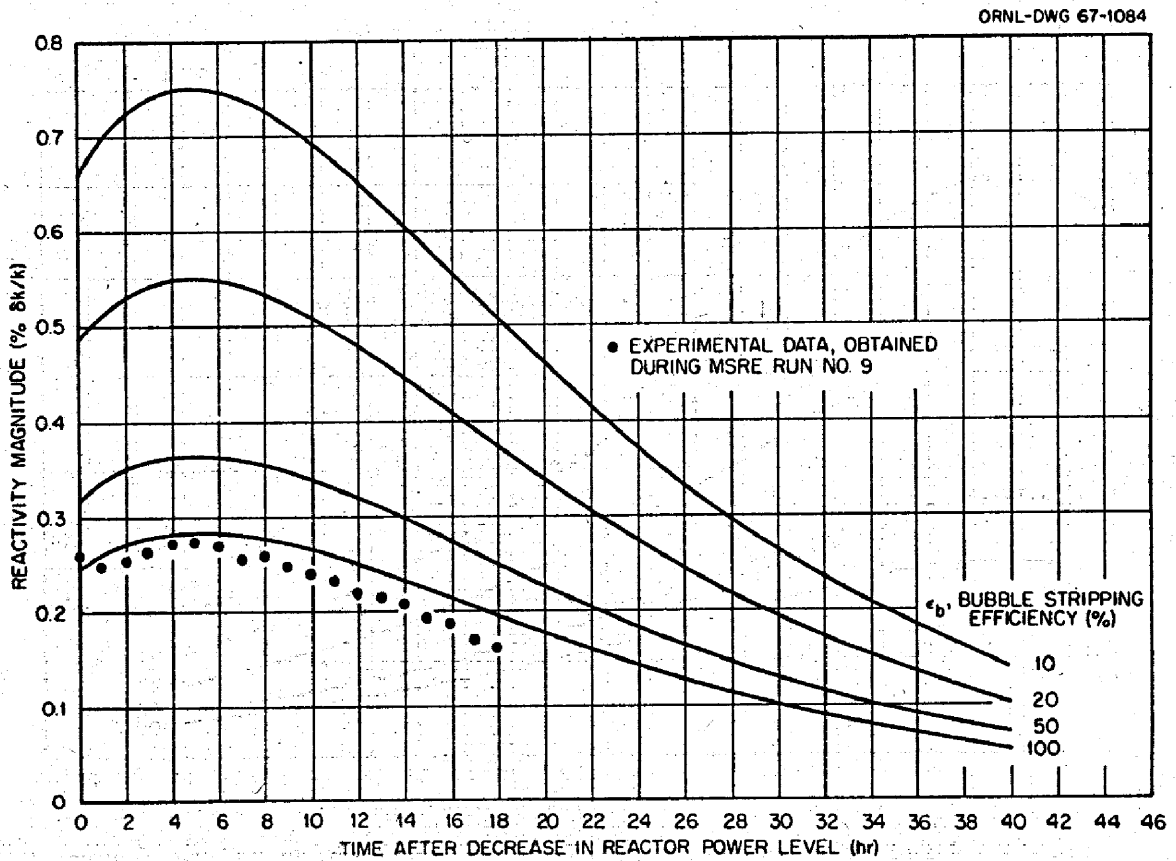
Fig. 10. Effect of Bubble-Stripping Efficiency on Transient Decay of ^{135}\text{Xe} Reactivity. Step decrease in power level from 7.4 Mw to 0; volume percent circulating bubbles, 0.10; MSRE Run No. 9.
