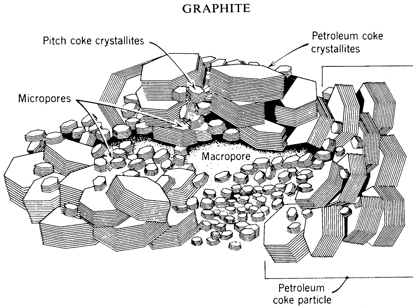
Fig. 8. Proposed Arrangement of Crystallites in Graphitized Stock. (Reprinted from High-Temperature Materials and Technology , ed. by I. E. Campbell and E. M. Sherwood, Wiley, New York, 1967, p. 195).
