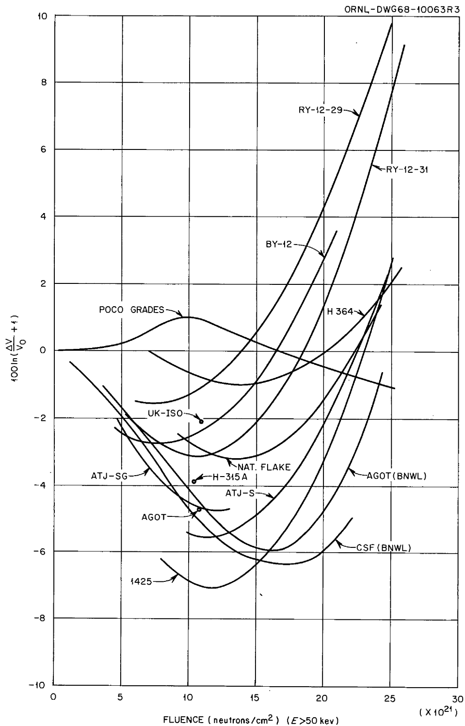
Fig. 9. Volume Changes of Graphite Irradiated at 705°C.
