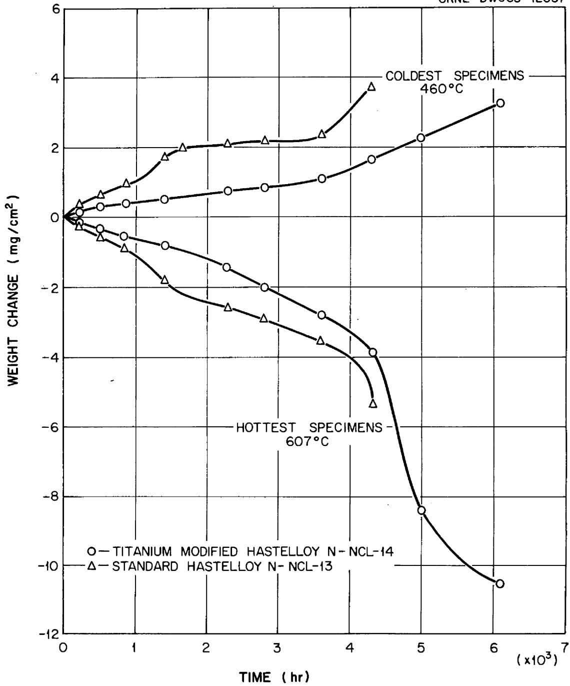
Fig. 12. Comparison of the Weight Changes of Hastelloy N Specimens Inserted in NaBF 4 -NaF (92-8 mole %) Thermal Convection Loops.
