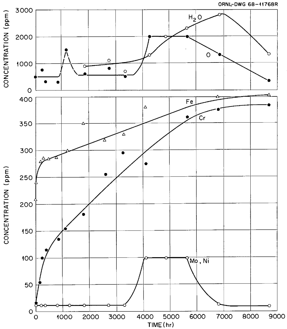
Fig. 13. Variation of Impurities with Time in NaBF 4 -NaF (92-8 mole %) Thermal Convection Loop NCL-14.
