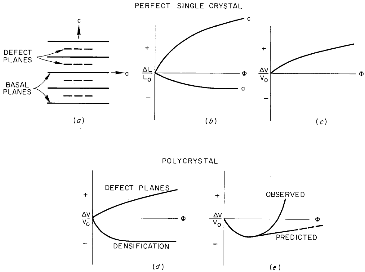
Fig. 7. Graphite Dimensional Changes Due to Irradiation.
