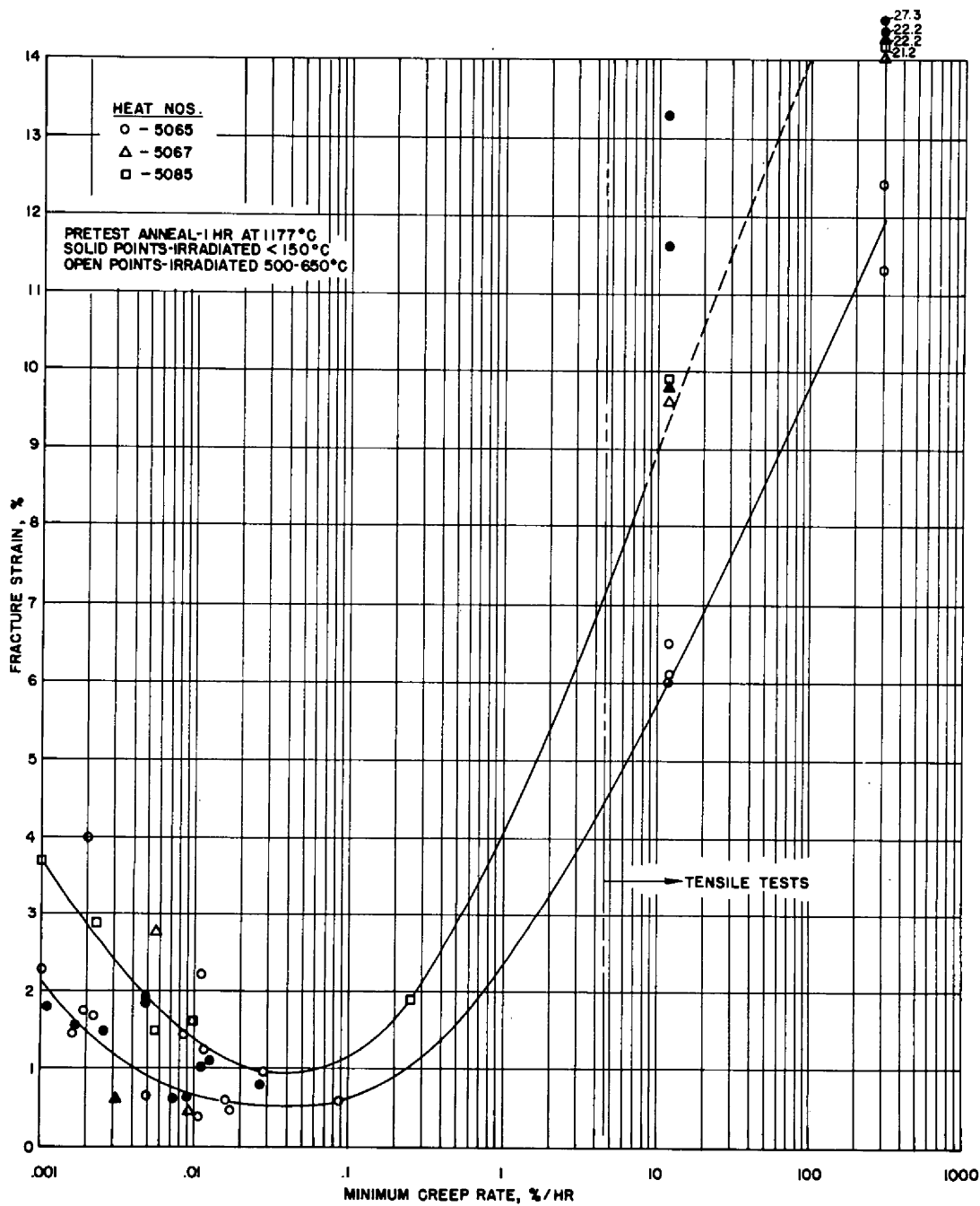
Fig. 3. Fracture Strain of Hastelloy N at 650°C After Irradiation to a Thermal Fluence of About 5 \times 10^{20} neutrons/cm 2 .
