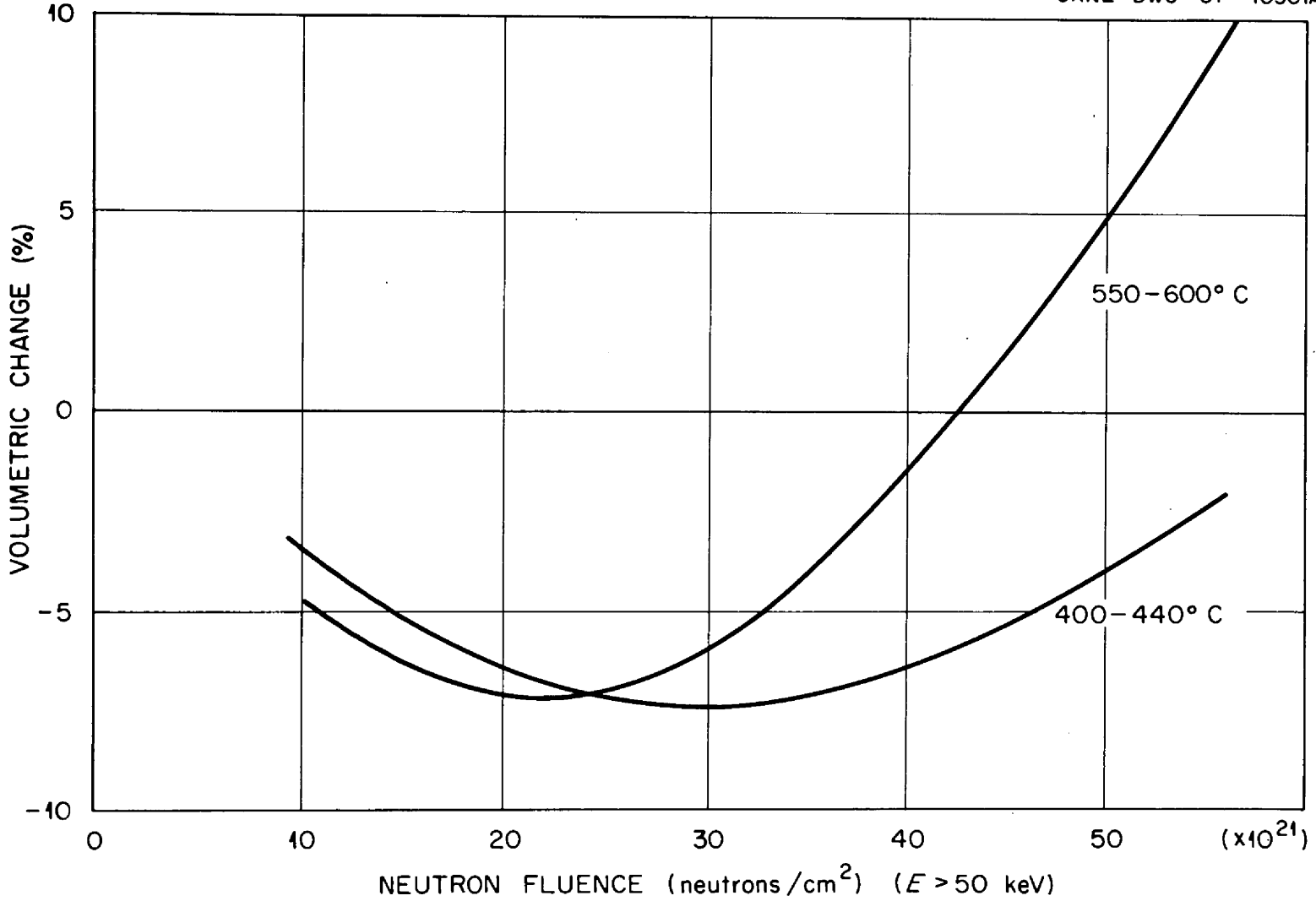
Fig. 6. Volume Change in Isotropic Graphite Dounreay Fast Reactor Irradiations.
