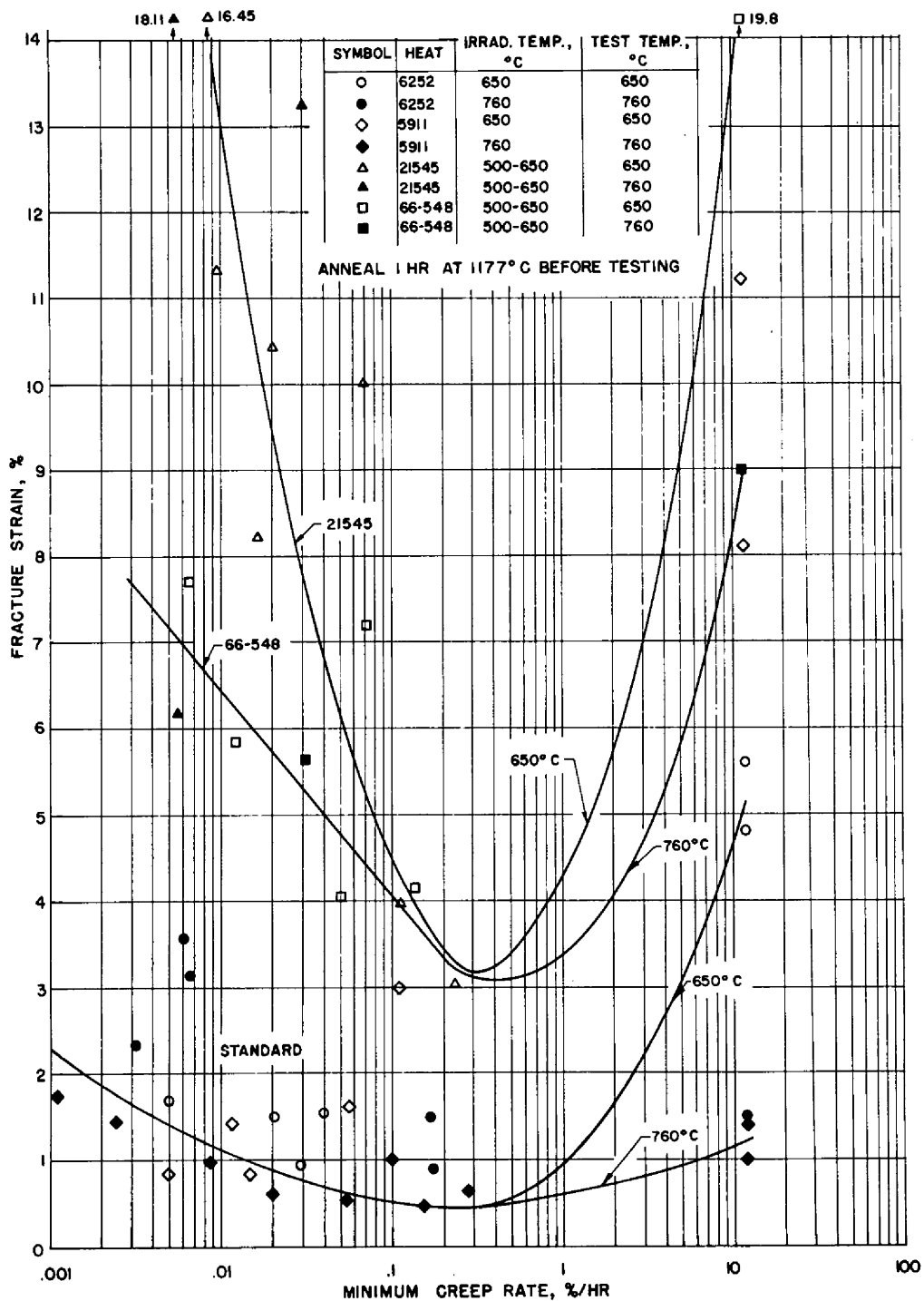
Fig. 5. Variation of Fracture Strain with Strain Rate for Several Hastelloy N Type Alloys. Samples irradiated to a fluence of about 5 \times 10^{20} neutrons/cm 2 prior to testing.
