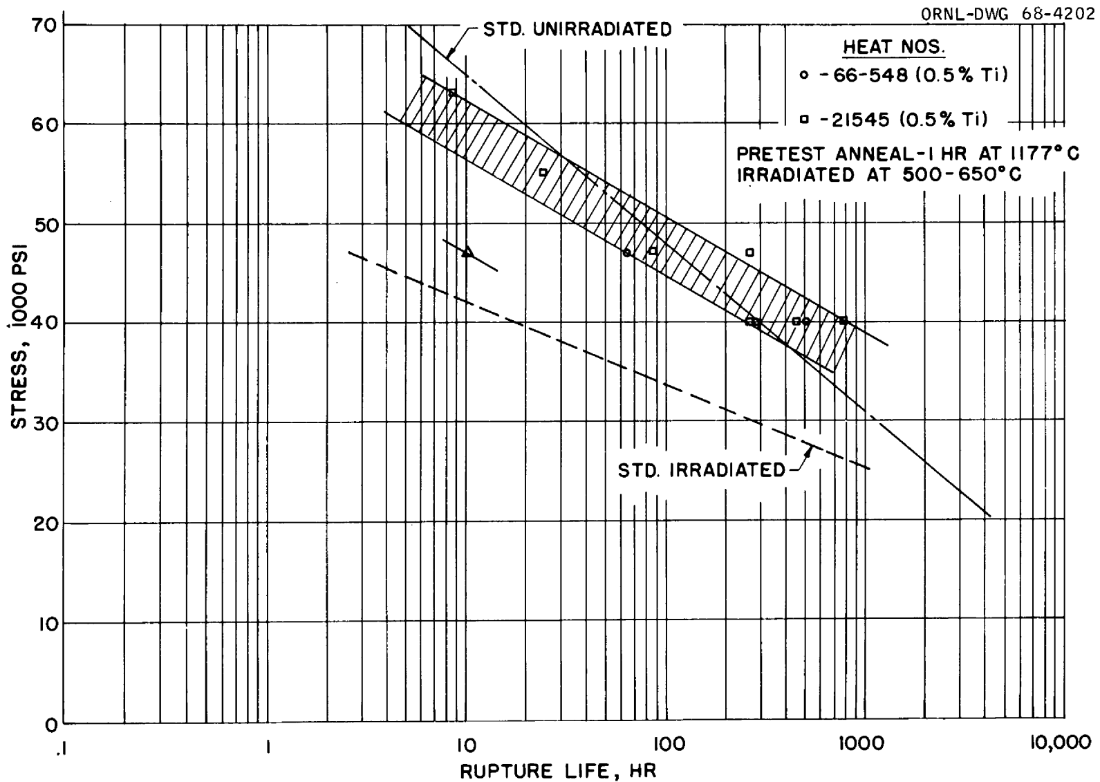
Fig. 4. Creep-Rupture Properties of Several Heats of Modified Hastelloy N at 650°C. Samples irradiated to a thermal fluence of about 5 \times 10^{20} neutrons/cm 2 .
