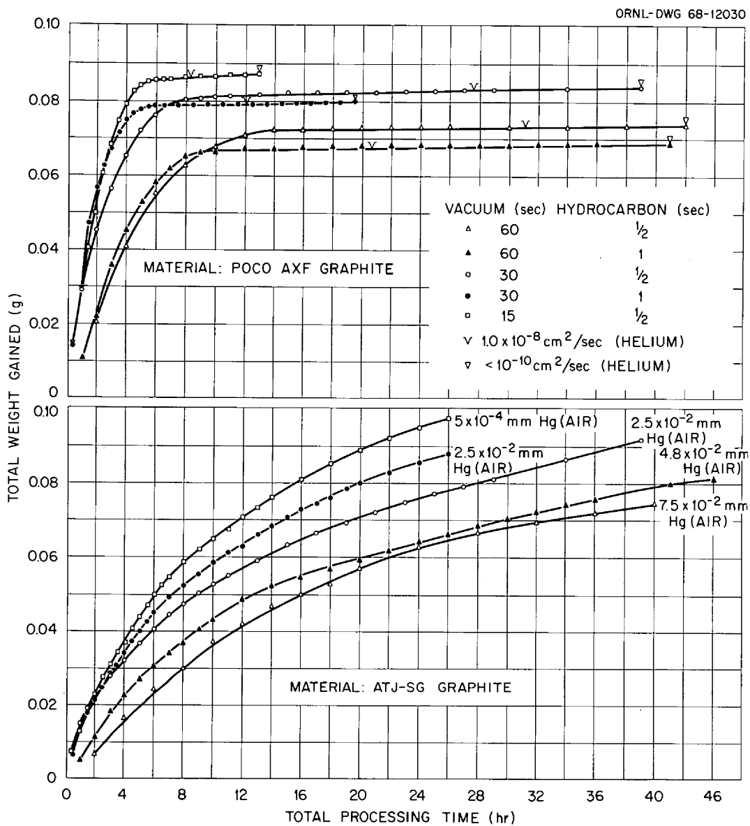
Fig. 11. Impregnation Rate of Graphite Using 1,3 Butadiene at 850°C.
