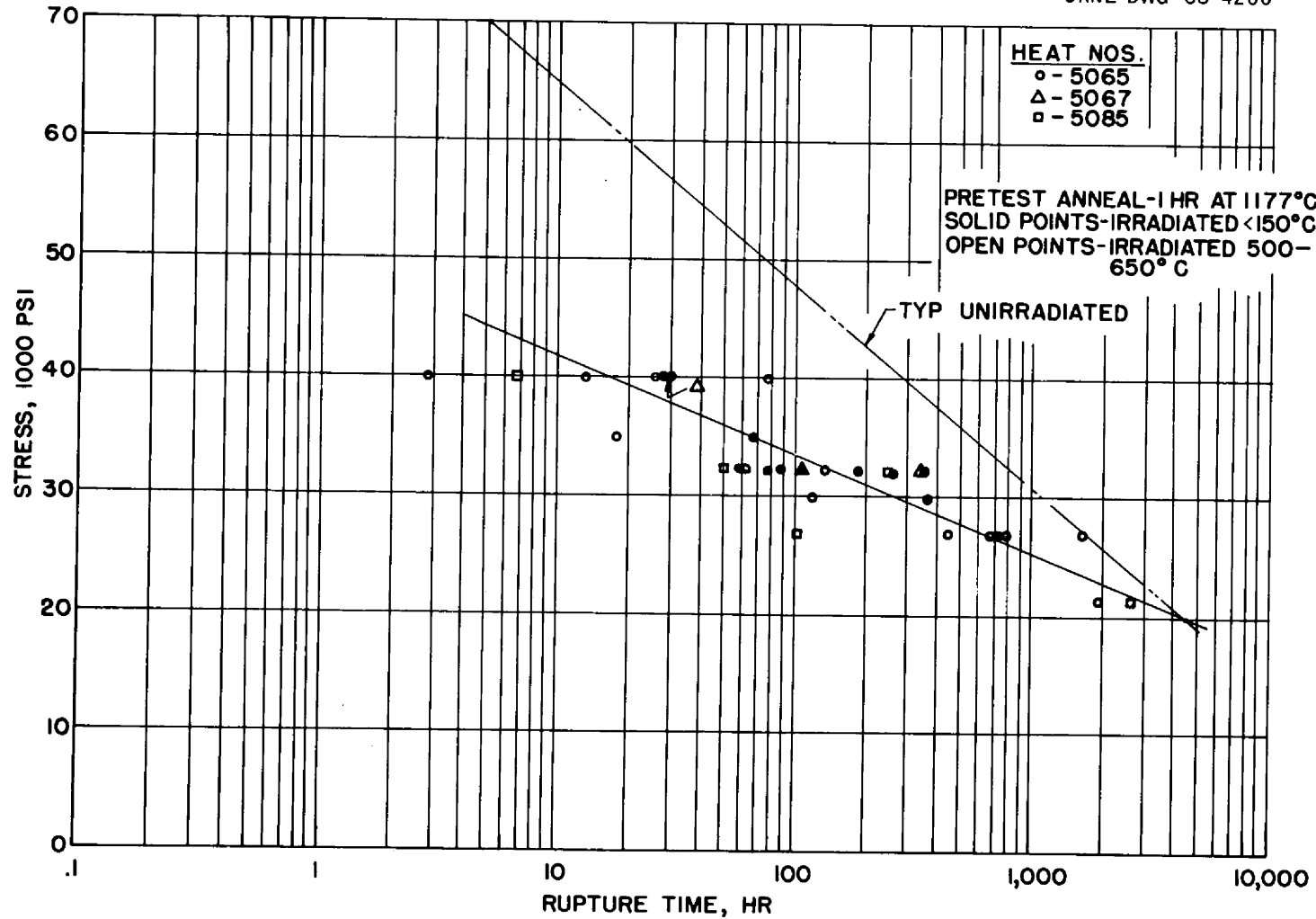
Fig. 2. Creep-Rupture Properties of Hastelloy N at 650°C After Irradiation to a Thermal Fluence of About 5 \times 10^{20} neutrons/cm 2 .
