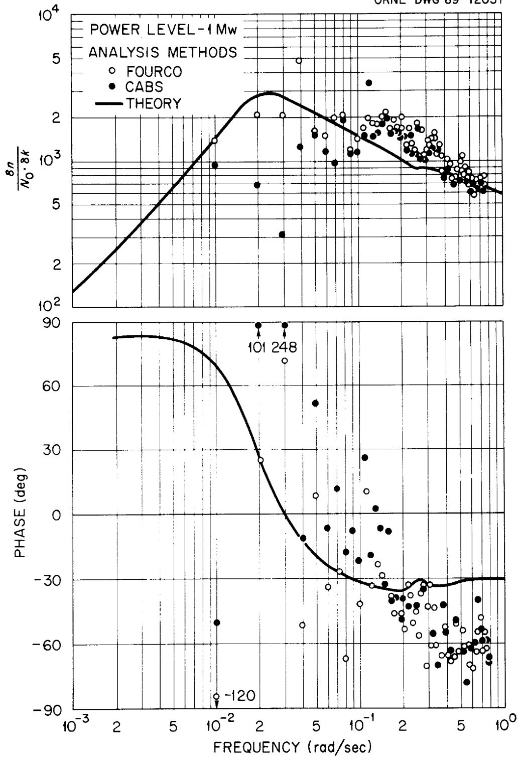
Fig. 7. Neutron Flux-to-Reactivity Frequency Response of the 233 U-Fueled MSRE at 1 MW.
