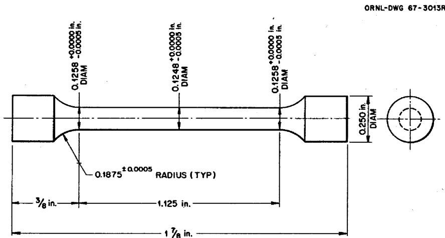
Fig. 1. Specimen Used for Tests of Mechanical Properties.
