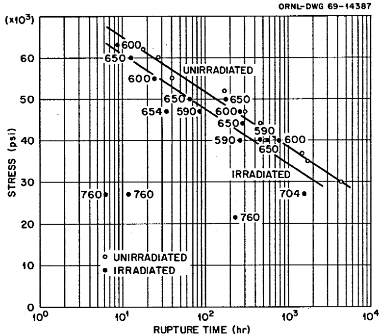
Fig. 18. Stress-Rupture Properties of Alloy 21545 (0.49% Ti) at 650°C. All material annealed 1 hr at 1177°C. Number by each datum point designates the irradiation temperature in degrees Celsius.
