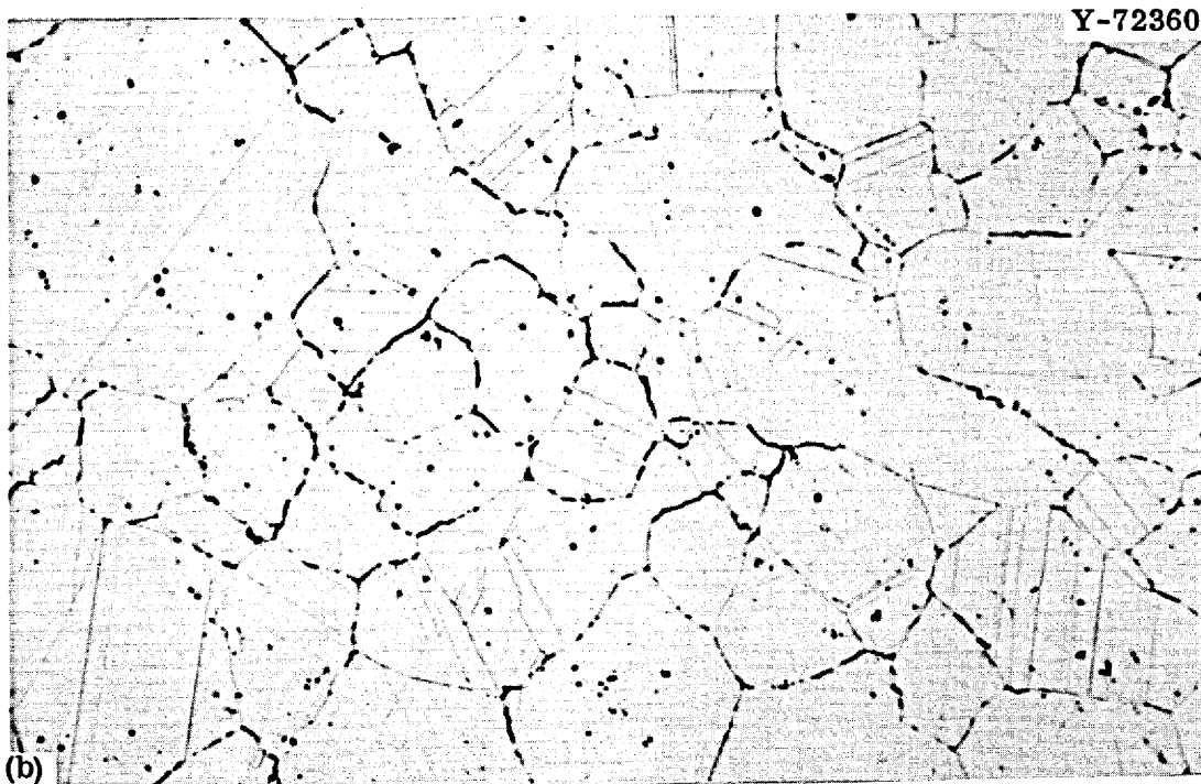
Fig. 77. Photomicrographs of Alloy 152 Modified with 0.16% Hf. Annealed 1 hr at 1177°C. (a) 100x and (b) 500x. Etchant: glyceria regia.
