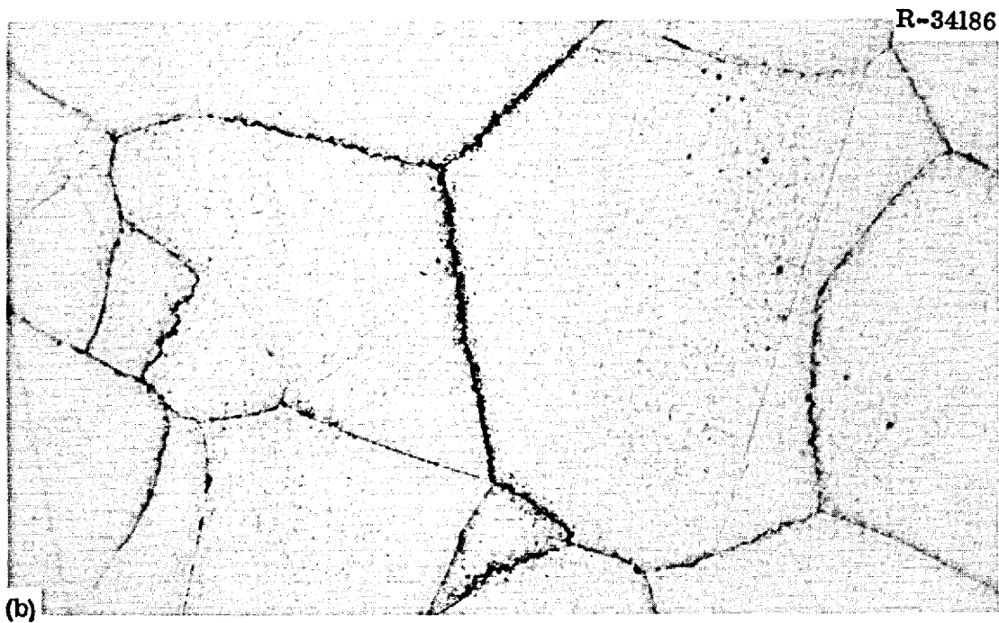
Fig. 29. Photomicrographs of Alloy 100 (< 0.01% Ti) after Annealing 1 hr at 1177°C, Irradiation for 1000 hr at 650°C to a Thermal Fluence of 2.5 \times 10^{20} neutrons/cm 2 , and Testing at a Stress of 32,400 psi at 650°C. Fractured in 105.4 hr with 1.1% strain. (a) Fracture, 100X; (b) typical, 500X. Etchant: aqua regia.
