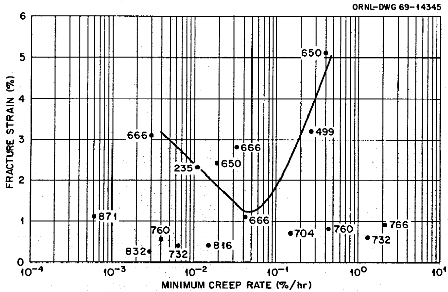
Fig. 105. Fracture Strains at 650°C of Irradiated Alloy 21546. All samples annealed 1 hr at 1177°C before testing. Number by each datum point indicates irradiation temperature.
