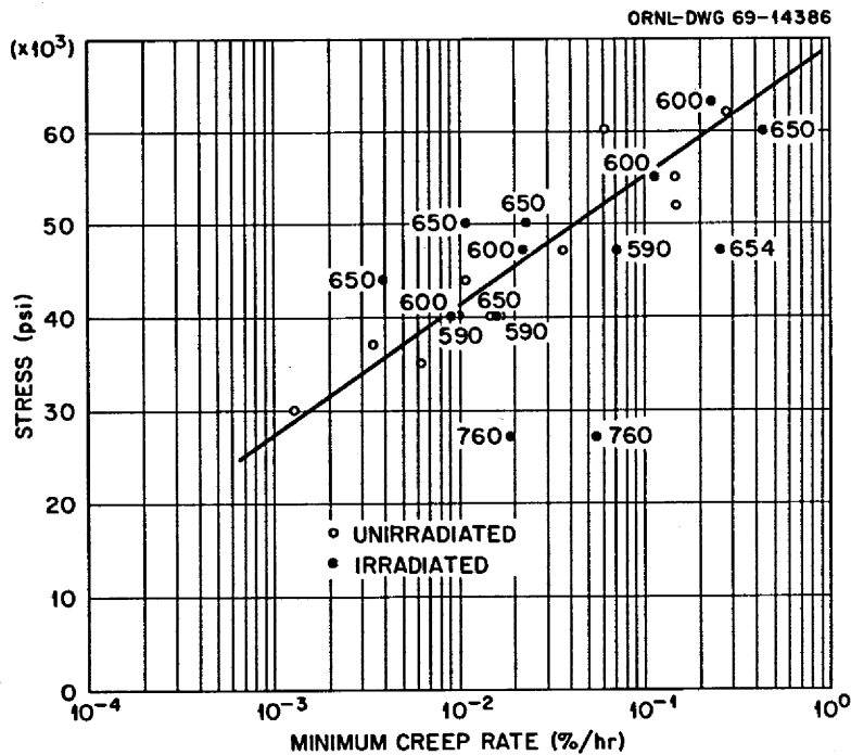
Fig. 19. Creep Properties at 650°C of Alloy 21545 (0.49% Ti). All material annealed 1 hr at 1177°C. Number by each datum point designates irradiation temperature in degrees Celsius.
