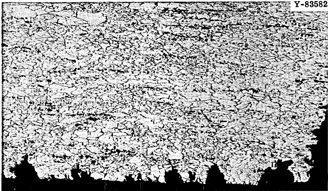
Fig. 75. Photomicrograph Showing a Portion of the Fracture of a Zirconium-Modified Hastelloy N Sample (Heat 21554) Tested at 650°C at a Strain Rate of 0.002 min -1 . Exposed to static fluoride salt for 5500 hr at 650°C before testing. 100X. Etchant: glyceria regia.
