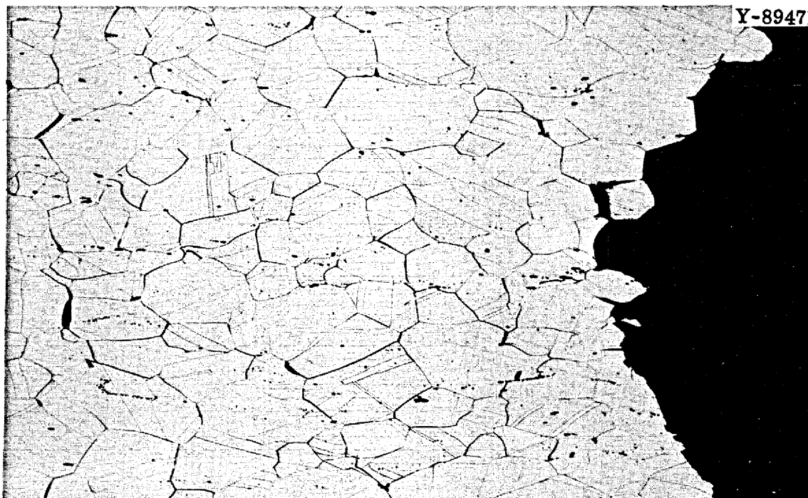
Fig. 99. Fracture of a Sample of Heat 67-504 (0.50% Hf) Annealed 1 hr at 1177°C and Creep Tested at 650°C and 40,000 psi. Etchant: glyceria regia. 100x.
