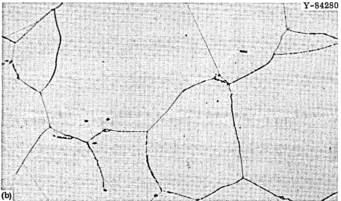
Fig. 80. Typical Photomicrographs of Heat 67-504 (0.50% Hf) Annealed 1 hr at 1177°C. Longitudinal section. (a) 100x and (b) 500x. Etchant: glyceria regia.
