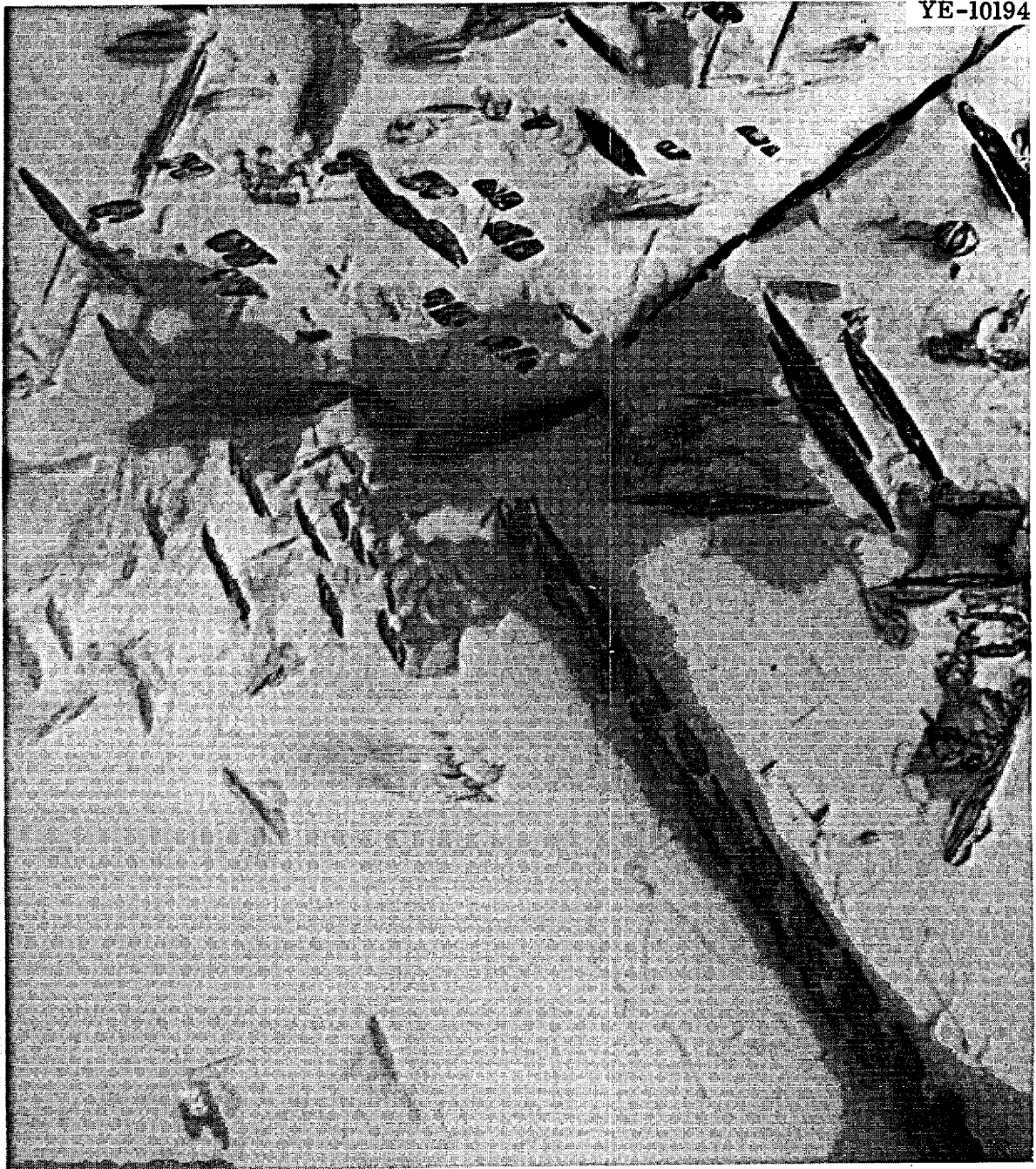
Fig. 108. Transmission Electron Photomicrograph of Alloy 21546 after Irradiation at 666°C for about 1100 hr to a Thermal-Neutron Fluence of 2.4 \times 10^{20} neutrons/cm 2 . 50,000X.
