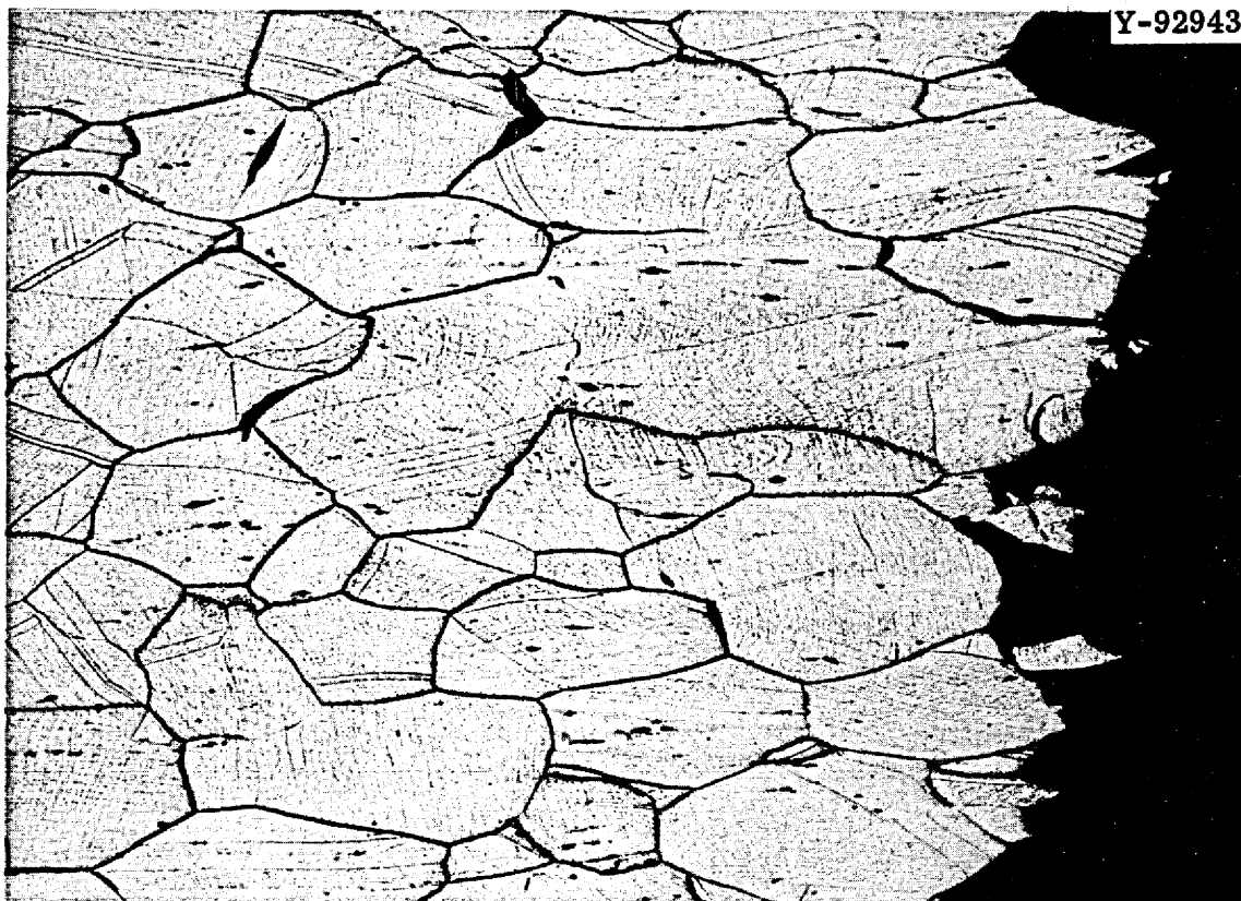
Fig. 96. Photomicrograph of the Fracture of a Sample of Heat 67-504 (0.50% Hf) Annealed 1 hr at 1177°C, Exposed 9800 hr to Fluoride Salt at 650°C, and Tested in Tension at 650°C and a Strain Rate of 0.002 min -1 . 100X.
