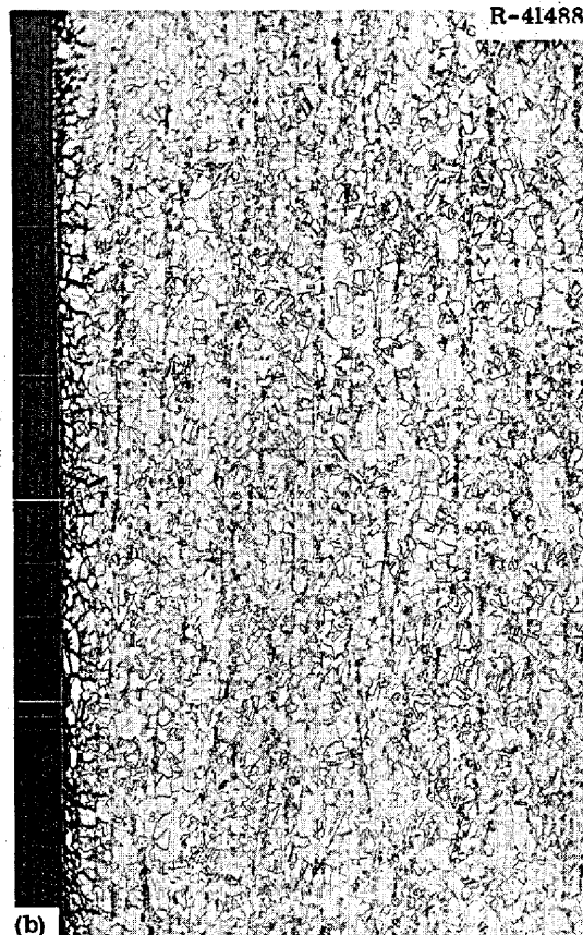
Fig. 74. Photomicrographs of a Zirconium-Modified Hastelloy N Surveillance Sample (Heat 21554) Tested at 650°C at a Strain Rate of 0.002 min -1 . Exposed in the Molten Salt Reactor Experiment core for 5500 hr at 650°C to a thermal fluence of 4.1 \times 10^{20} neutrons/cm 2 . (a) Fracture, 100x; (b) edge of sample about 1/2 in. from fracture, 100x; and (c) edge of sample showing edge cracking. Oxide formed during the tensile test. 500x. Etchant: aqua regia. Reduced 22%.
