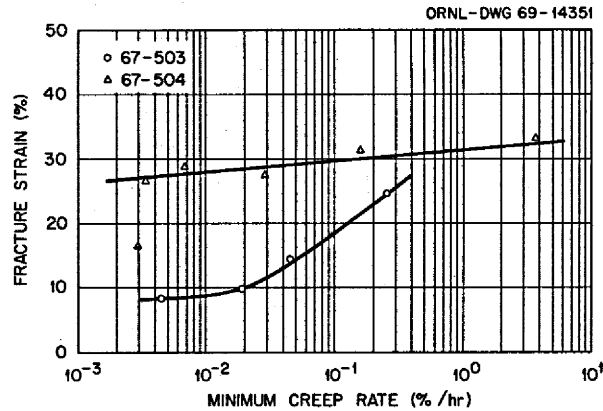
Fig. 92. Fracture Strains at 650°C of Unirradiated Alloys 67-503 and 67-504. All samples annealed 1 hr at 1177°C.
