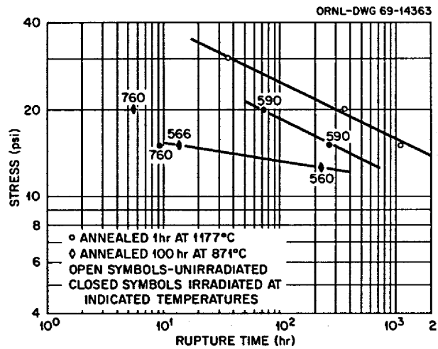
Fig. 61. Stress-Rupture Properties of Alloy 2154 (0.35% Zr) at 760°C.
