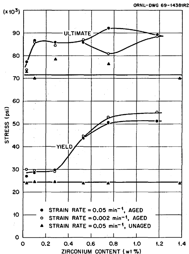
Fig. 39. Influence of Zirconium Content on Tensile Properties after Annealing 1 hr at 1177°C and Aging 1000 hr at 650°C.
