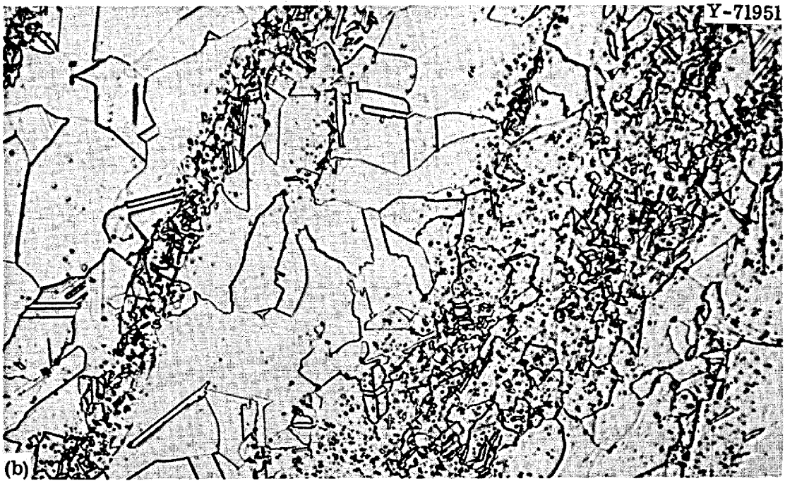
Fig. 100. Photomicrographs of Alloy 21546 Annealed 100 hr at 871°C. The material was cold worked 40% before annealing. (a) 100x and (b) 500x. Etchant: glyceria regia.
