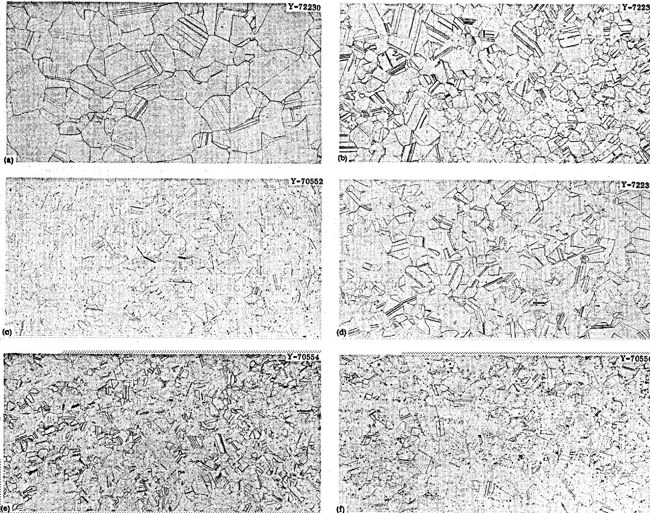
Fig. 36. Typical Photomicrographs of Alloys 100 and 108 Through 112. Annealed 1 hr at 1177°C. (a) Alloy 100 (< 0.03% Zr), (b) alloy 108 (0.10% Zr), (c) alloy 109 (0.28% Zr), (d) alloy 110 (0.53% Zr), (e) alloy 111 (0.75% Zr), and (f) alloy 112 (1.18% Zr). 100X. Etchant: glyceria regia. Reduced 42.5%.
