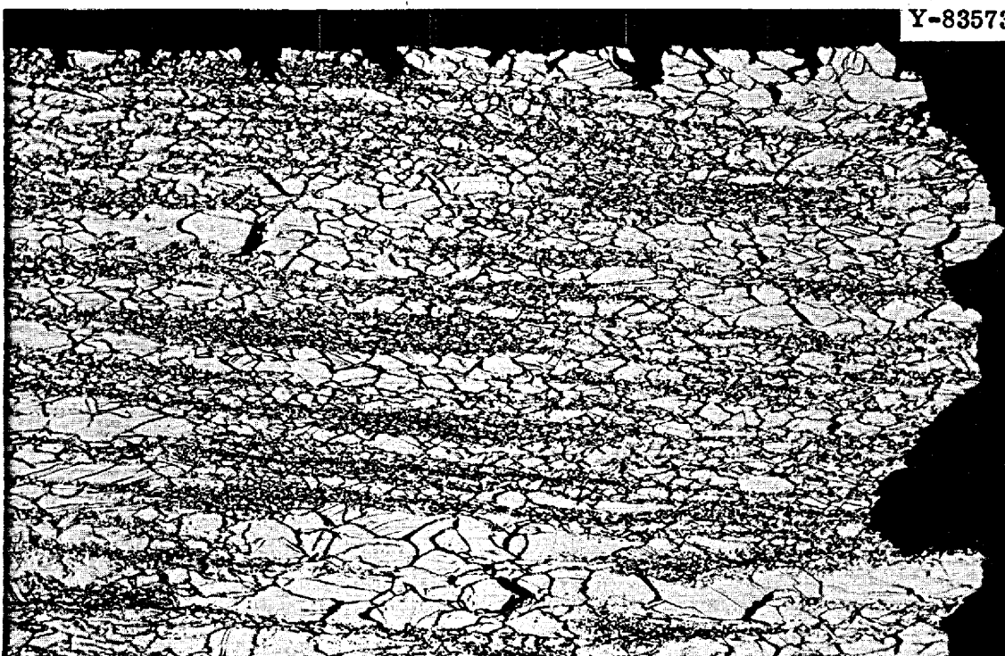
Fig. 35. Photomicrograph Showing a Portion of the Fracture of a Titanium-Modified Hastelloy N Surveillance Sample (Heat 21545) Tested at 650°C at a Strain Rate of 0.002 min -1 . Failed after 40.8% strain. Exposed to static fluoride salt for 5500 hr at 650°C before testing. 100X. Etchant: glyceria regia.
