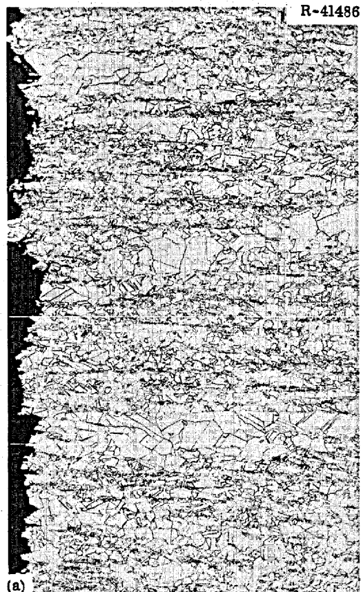
Fig. 74. Photomicrographs of a Zirconium-Modified Hastelloy N Surveillance Sample (Heat 21554) Tested at 650°C at a Strain Rate of 0.002 min -1 . Exposed in the Molten Salt Reactor Experiment core for 5500 hr at 650°C to a thermal fluence of 4.1 \times 10^{20} neutrons/cm 2 . (a) Fracture, 100x; (b) edge of sample about 1/2 in. from fracture, 100x; and (c) edge of sample showing edge cracking. Oxide formed during the tensile test. 500x. Etchant: aqua regia. Reduced 22%.
