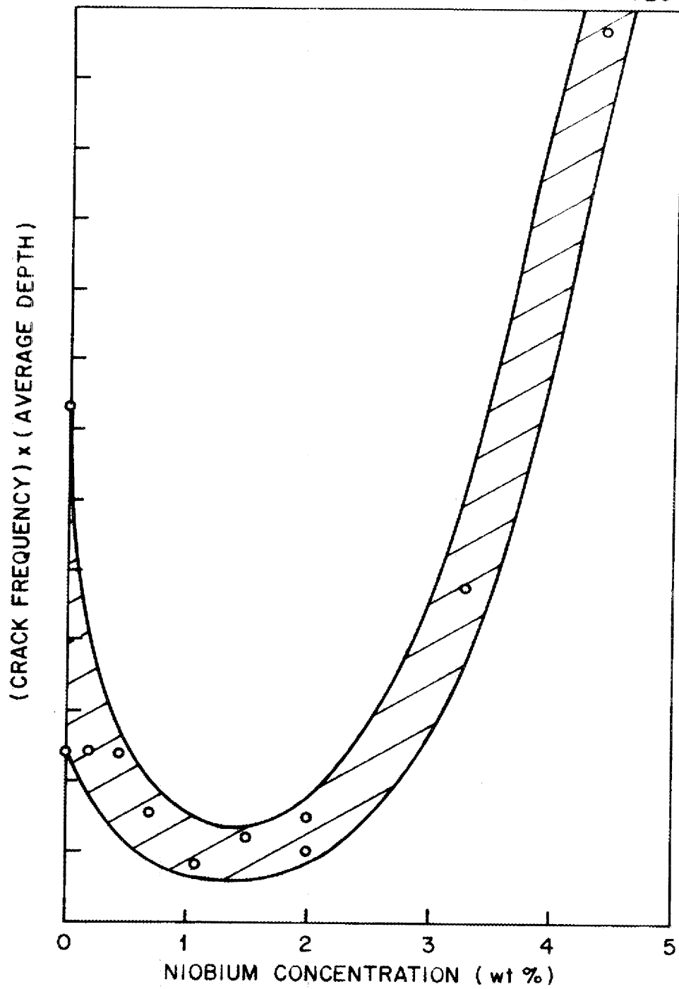
Fig. 9. Effect of Niobium in Modified Hastelloy N on Grain Boundary Cracking when Exposed in Salt- \text{Cr}_3\text{Te}_4 + \text{Cr}_5\text{Te}_6 for 250 hr at 700^\circ\text{C} .
